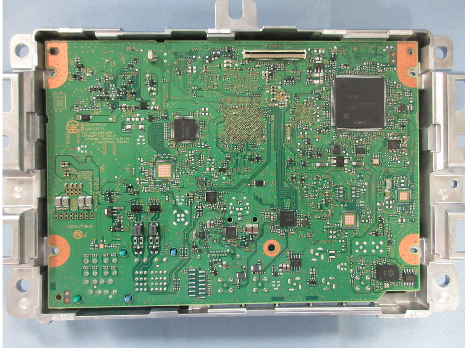
PCB-MAIN S-side
