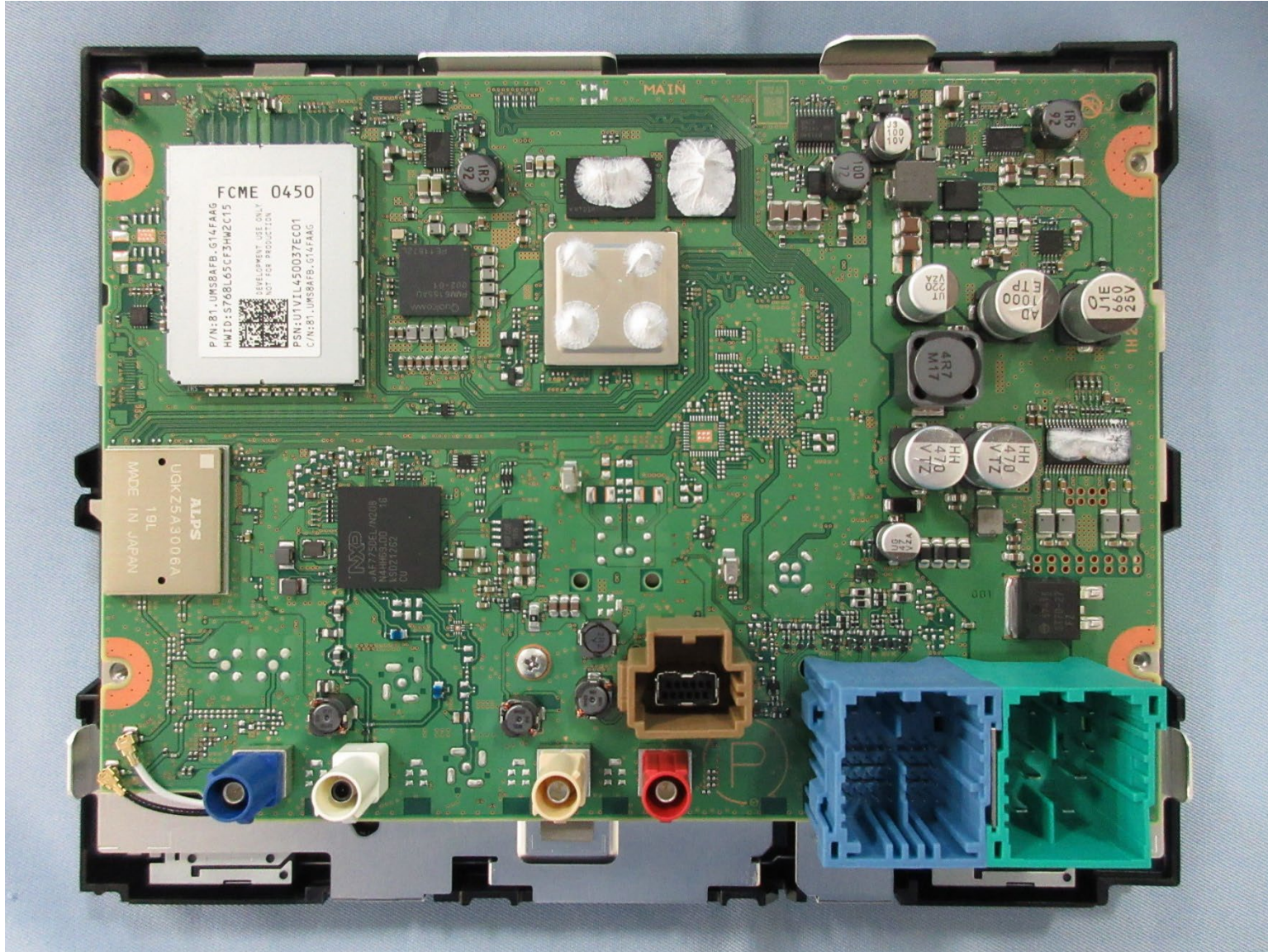
PCB-MAIN C-side
