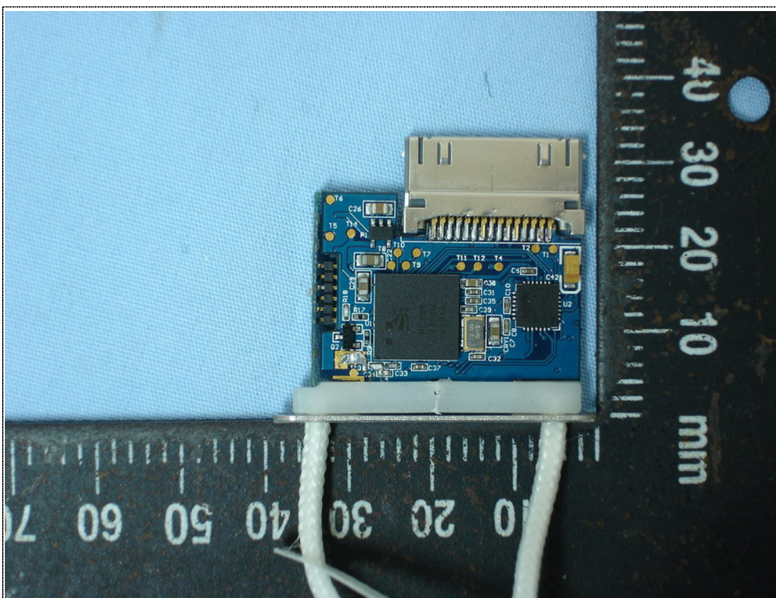
Front View of PCB board
