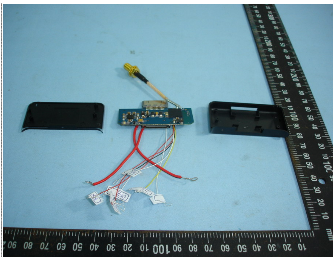
Inner view of Dongle
