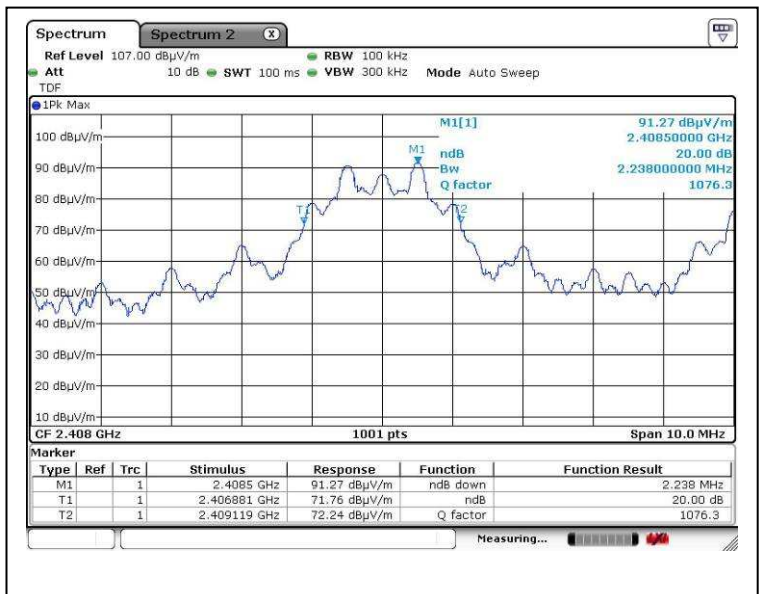
Bandwidth 1 (2408MHz)
