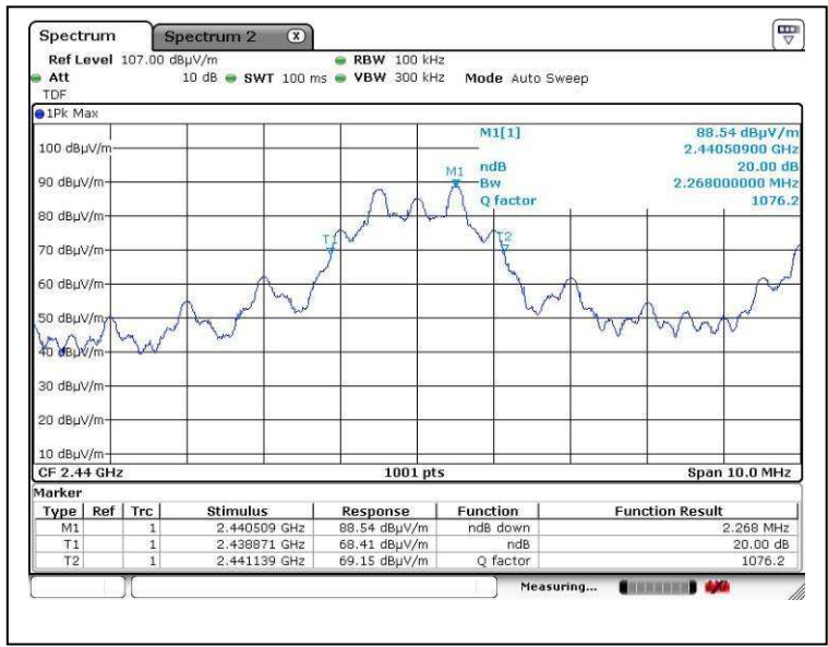
Bandwidth 2 (2440MHz)
