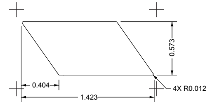
Diecut Outline
