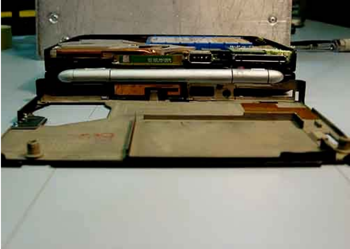
Rear WiFi and BT antenna and shield
