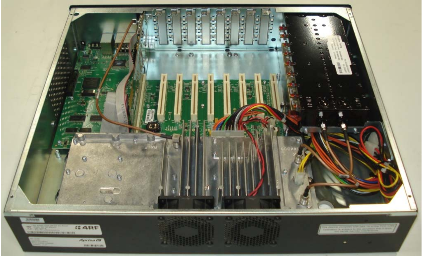
Figure E13.3 – Internal Photo From Front
