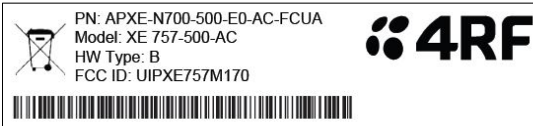
Figure E5.3 – Sample Label, 500kHz Variant
