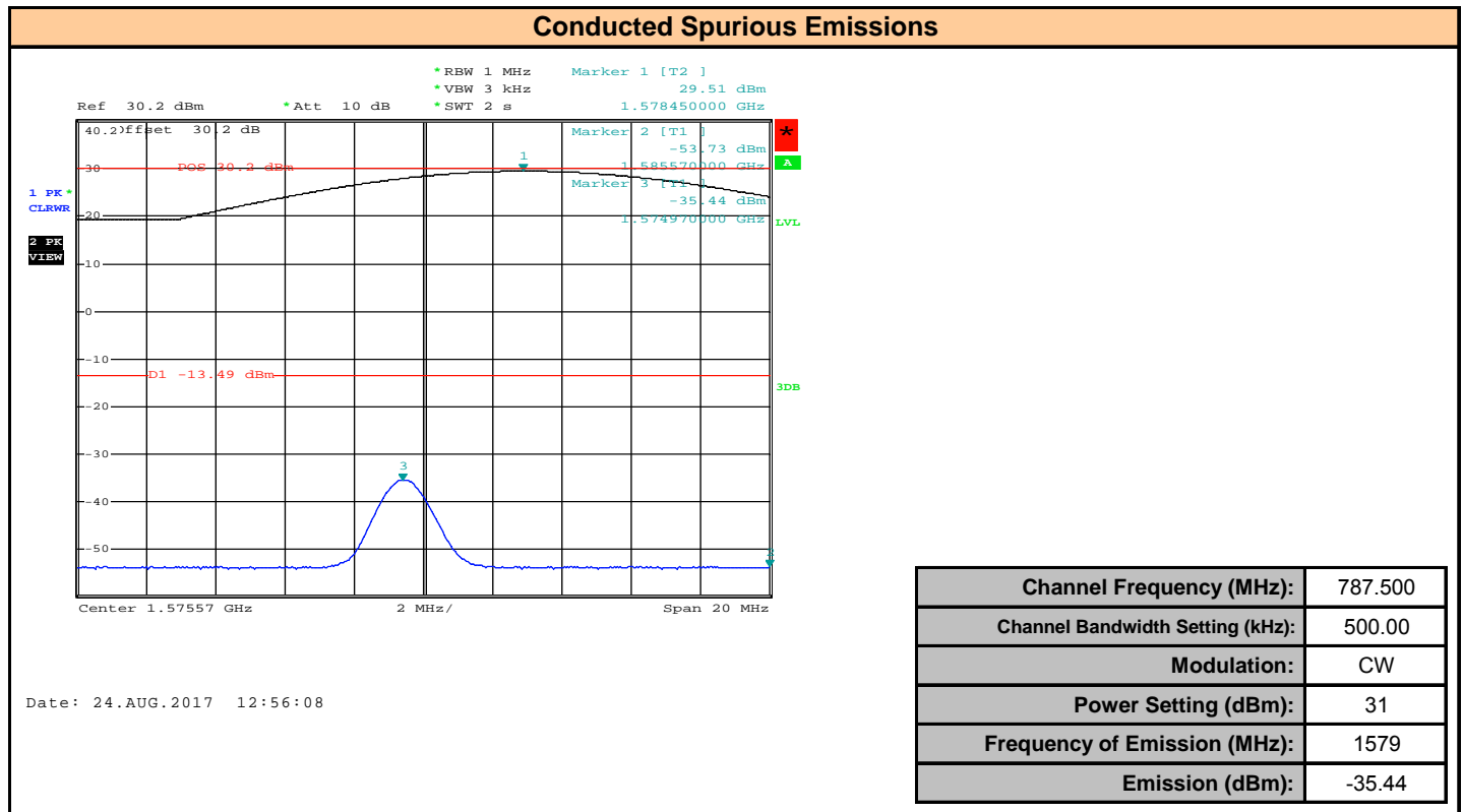
Plot 11.23 – Conducted Spurious Emission, 787.5MHz, 500kHz BW, CW, 2 nd Harmonic
