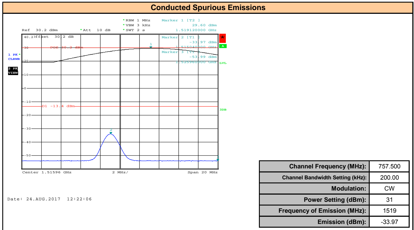
Plot 11.11 – Conducted Spurious Emission, 757.5MHz, 200kHz BW, CW, 2 nd Harmonic
