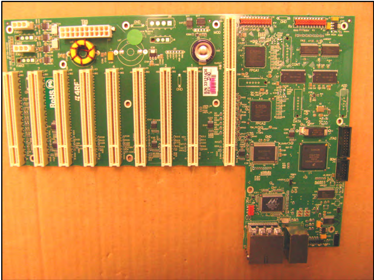
Photograph 35: Main Board – Top View
