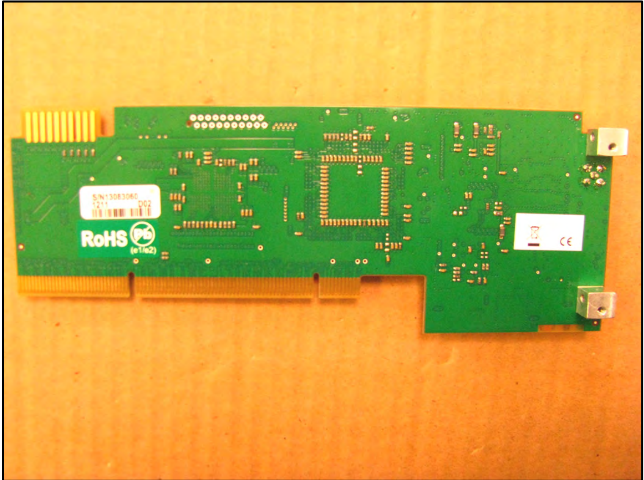
Photograph 34: Modem Card – Back View
