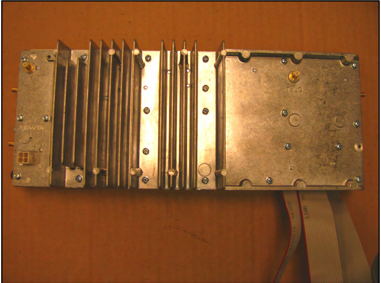
Photograph 22: RF Module – Top View
