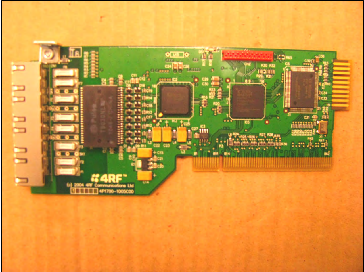
Photograph 30: PJET Card – Front View
