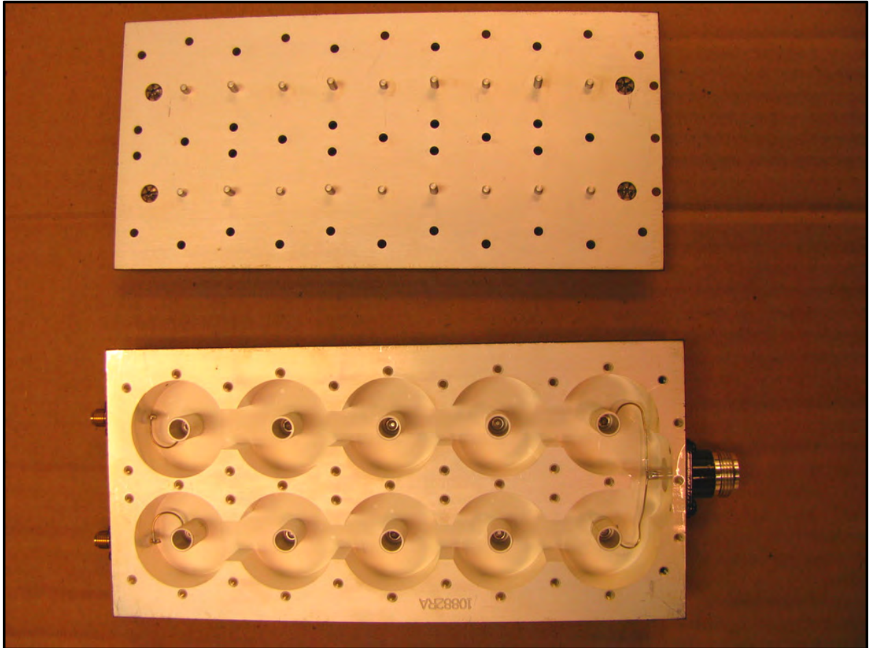
Photograph 17: Duplexer – Inside View
