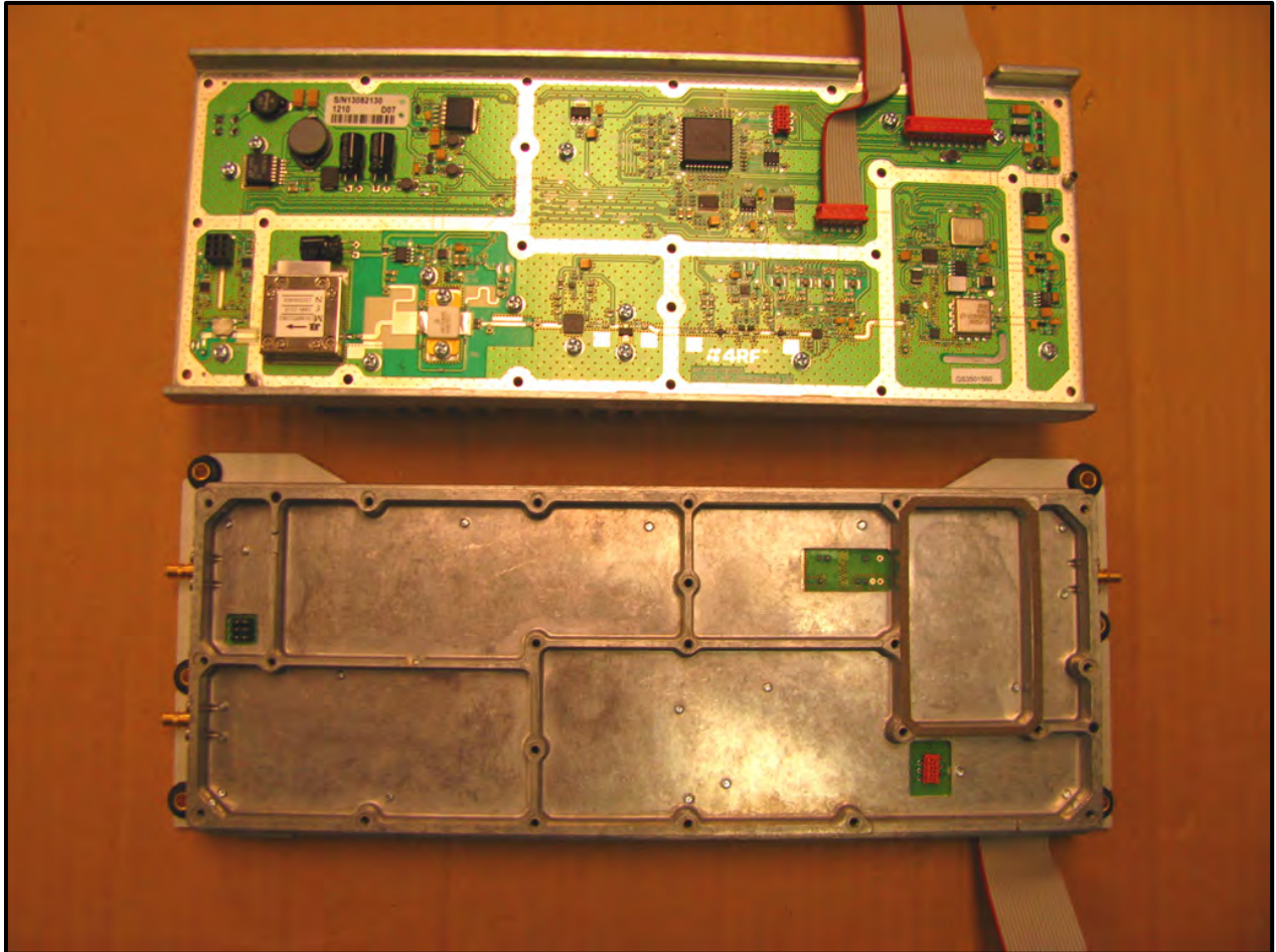
Photograph 24: Upper RF Module Case – Inside View
