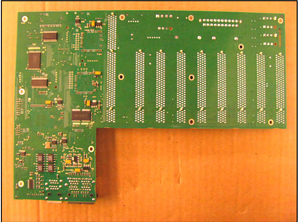
Photograph 36: Main Board – Bottom View
