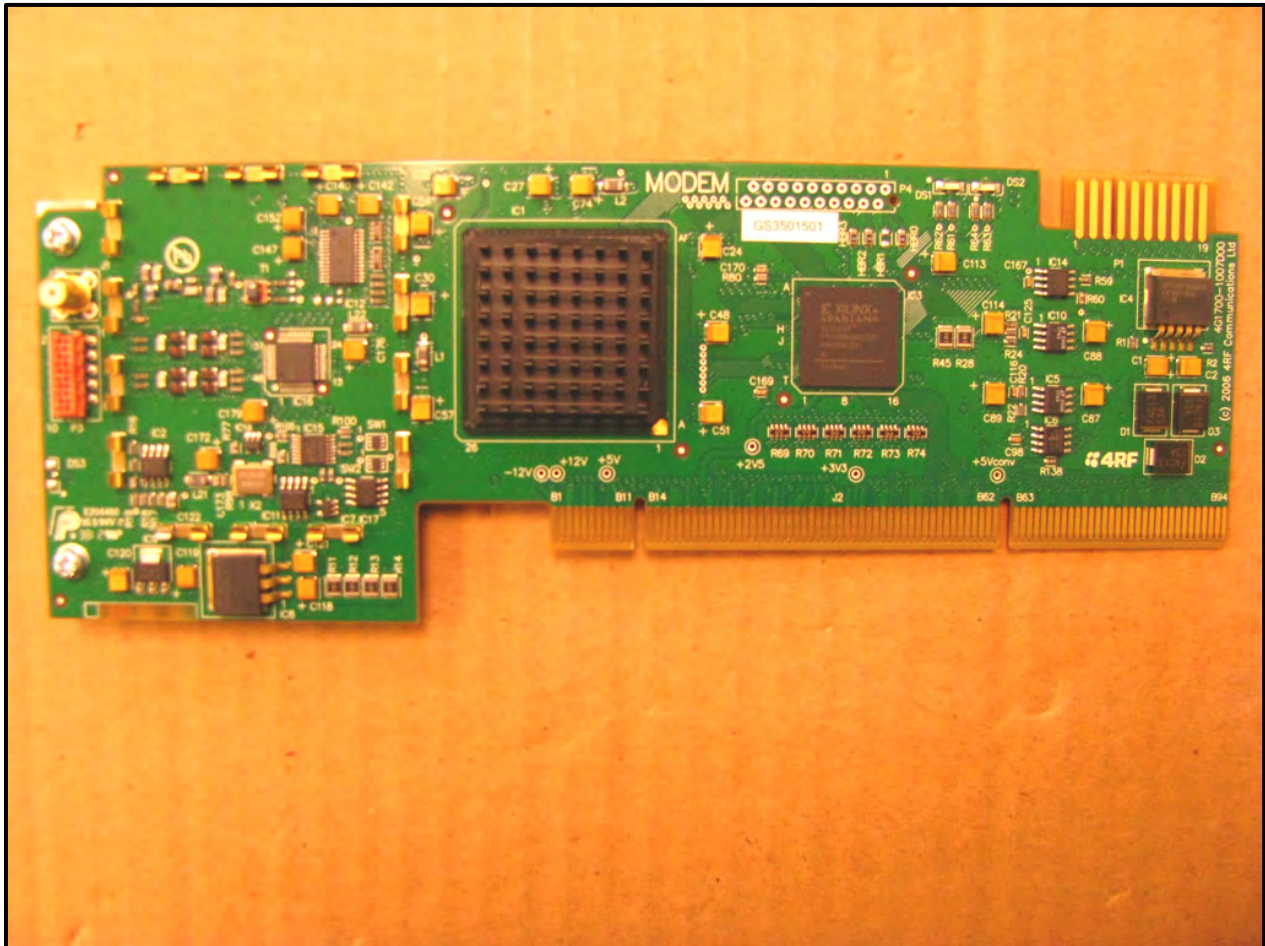
Photograph 33: Modem Card – Front View without Shields
