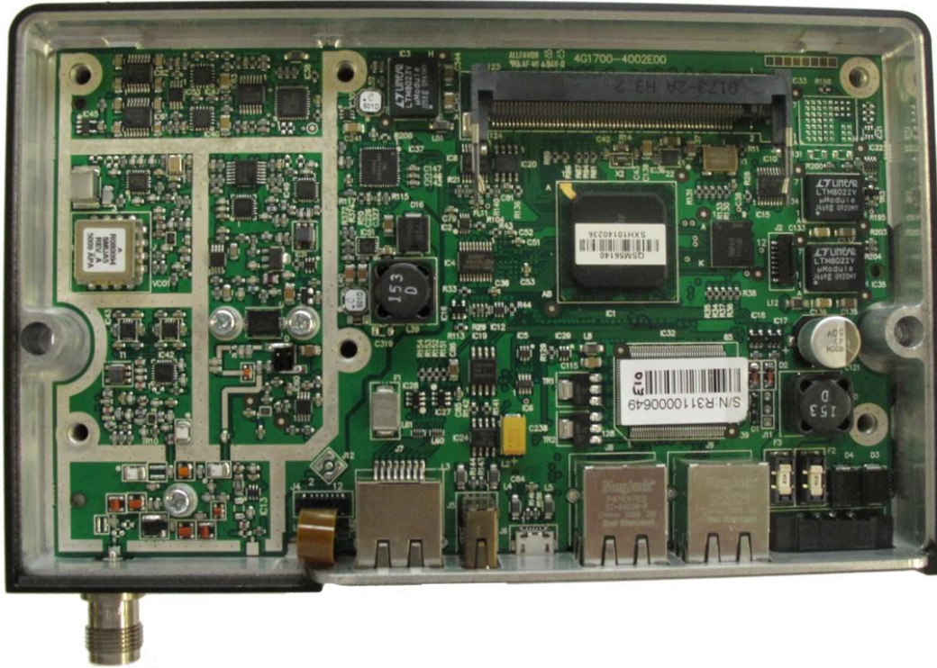
The Aprisa SR Printed Board Assembly mounted in the enclosure base.
