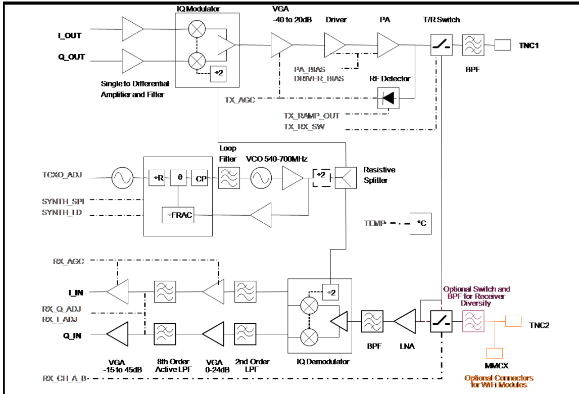
Radio Block Diagram, Aprisa SR (taken from pg, 46 of the user guide)
