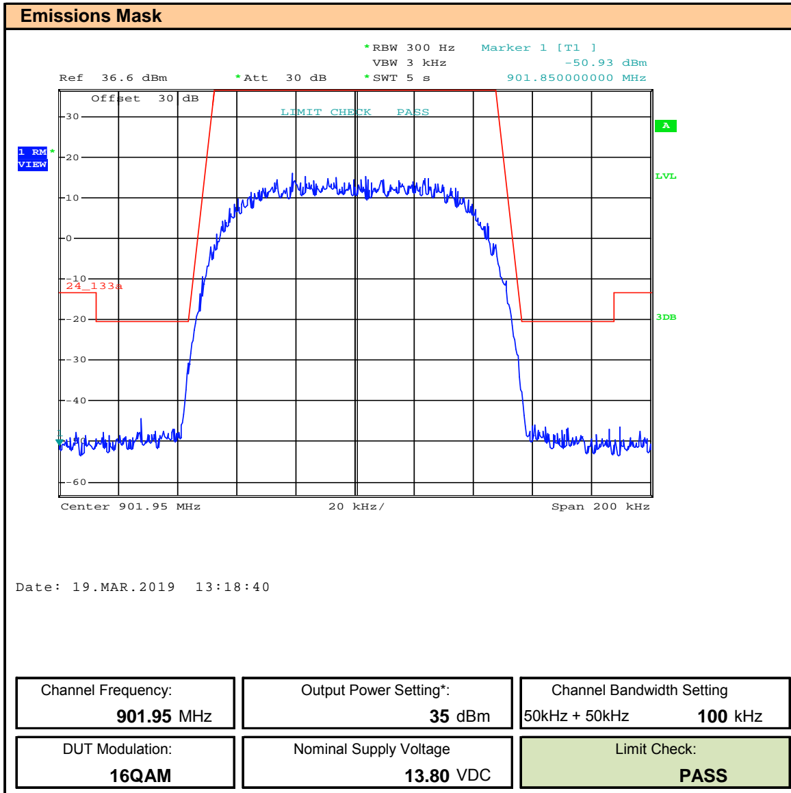
Plot 9.8 – Emissions Mask – 901.95, 100kHz BW, 16QAM
