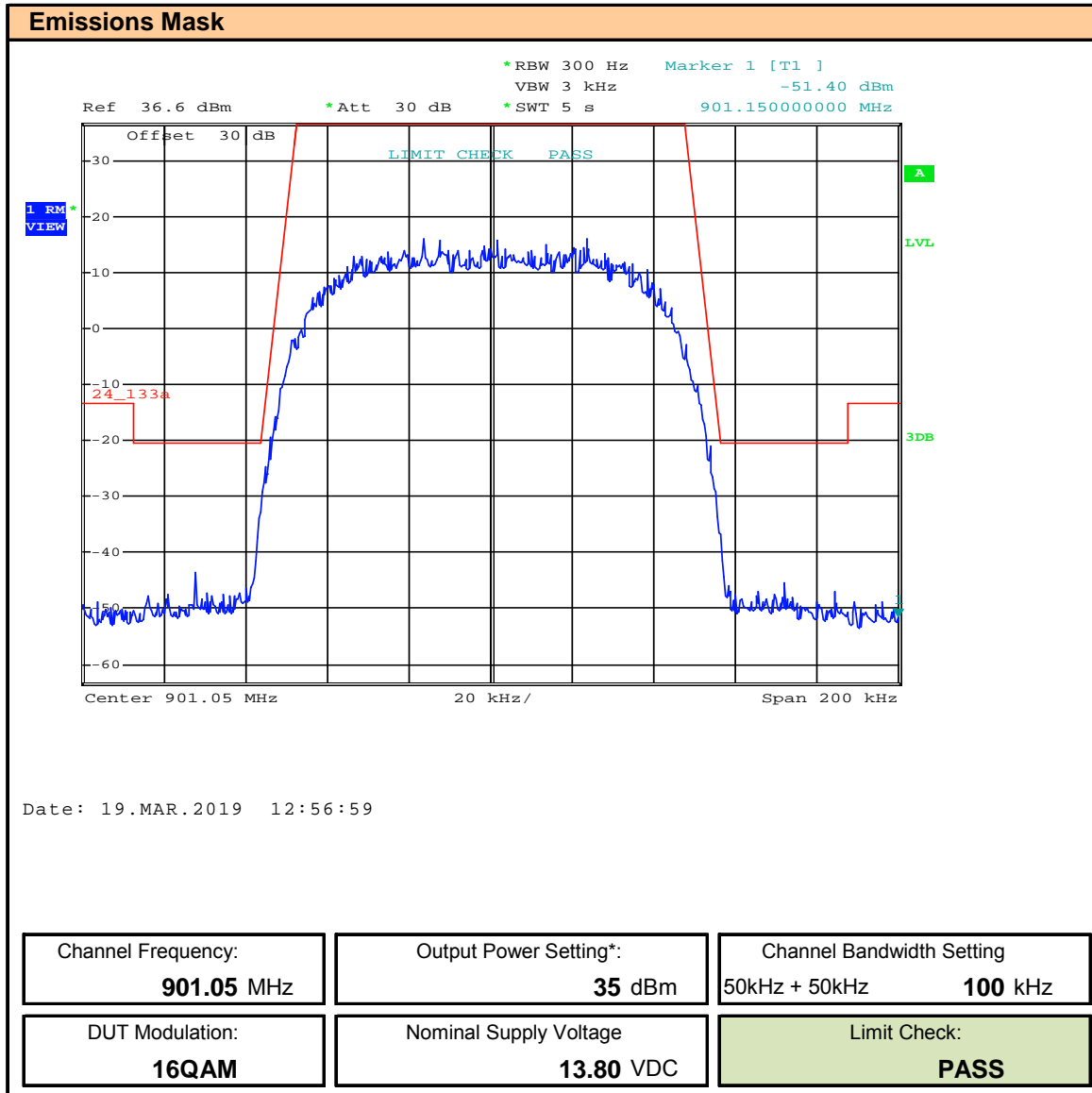
Plot 9.2 – Emissions Mask – 901.05, 100kHz BW, 16QAM
