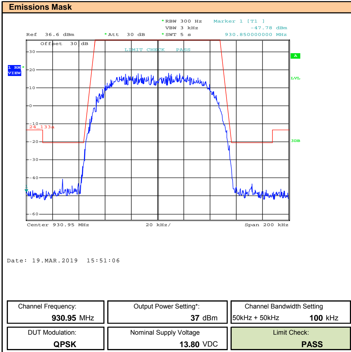
Plot 9.16 – Emissions Mask – 930.95, 100kHz BW, QPSK
