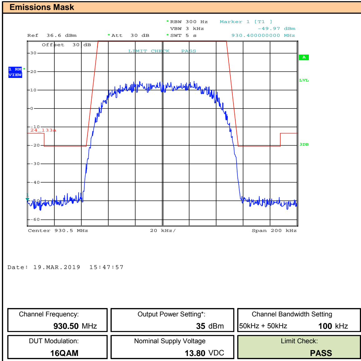
Plot 9.14 – Emissions Mask – 930.5, 100kHz BW, 16QAM
