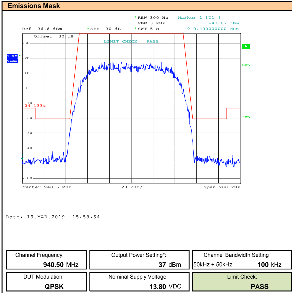
Plot 9.22 – Emissions Mask – 940.5, 100kHz BW, QPSK
