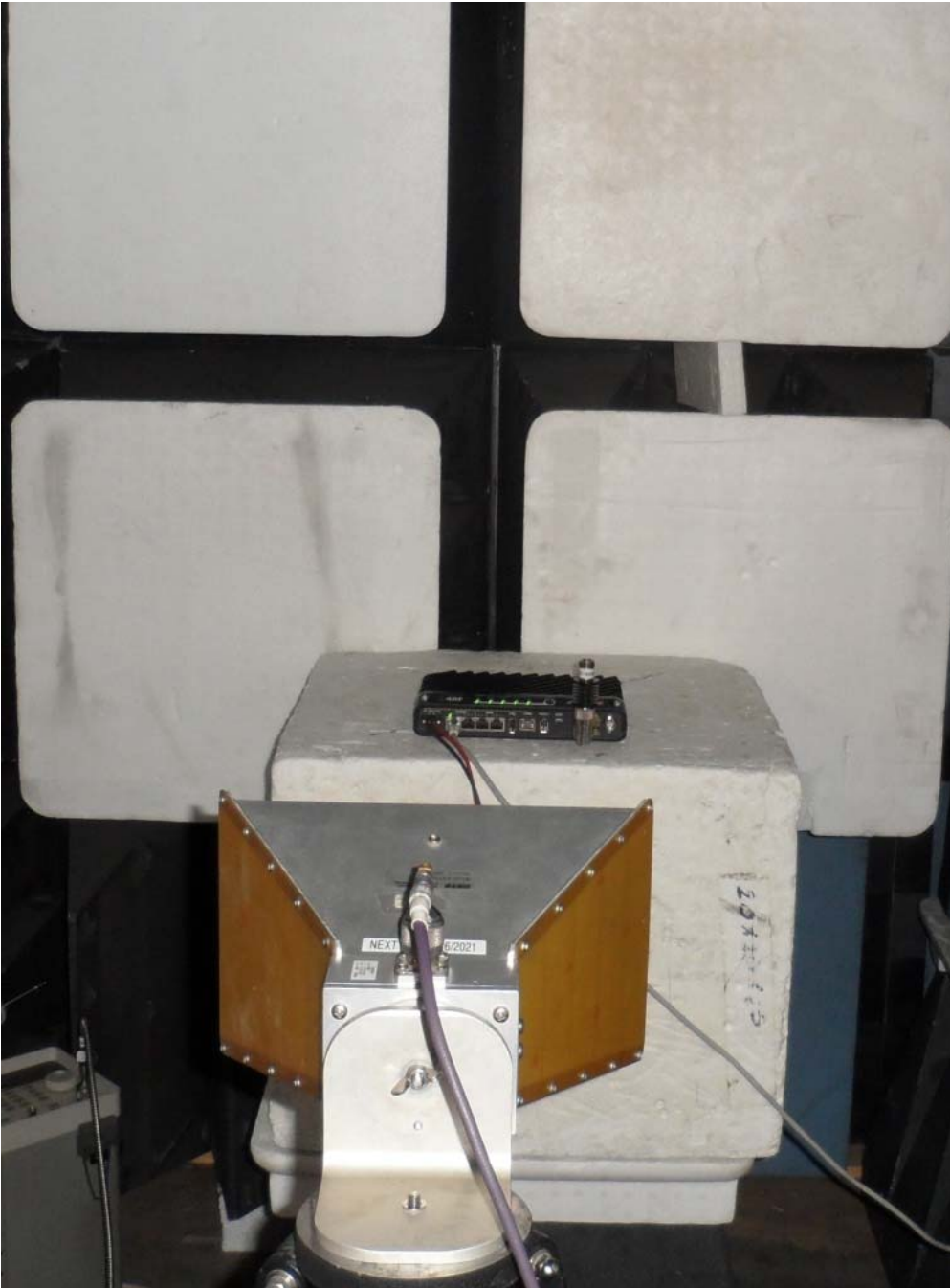
Figure E6.2 – Setup Photo – Radiated Measurements (Pre-Scan)
