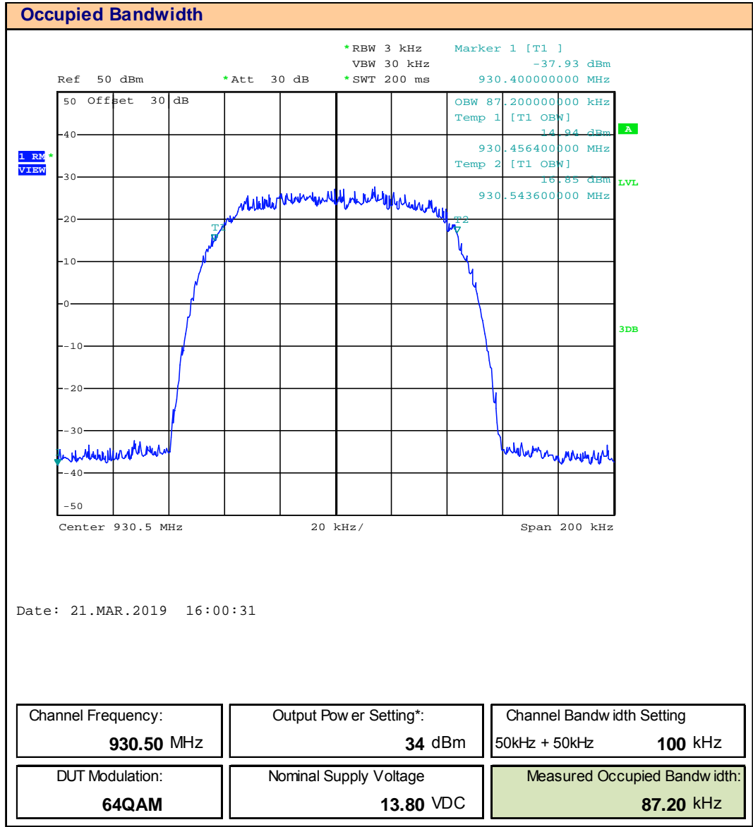
Plot 8.6 – Occupied Bandwidth – 930.5MHz, 100kHz BW, 64QAM
