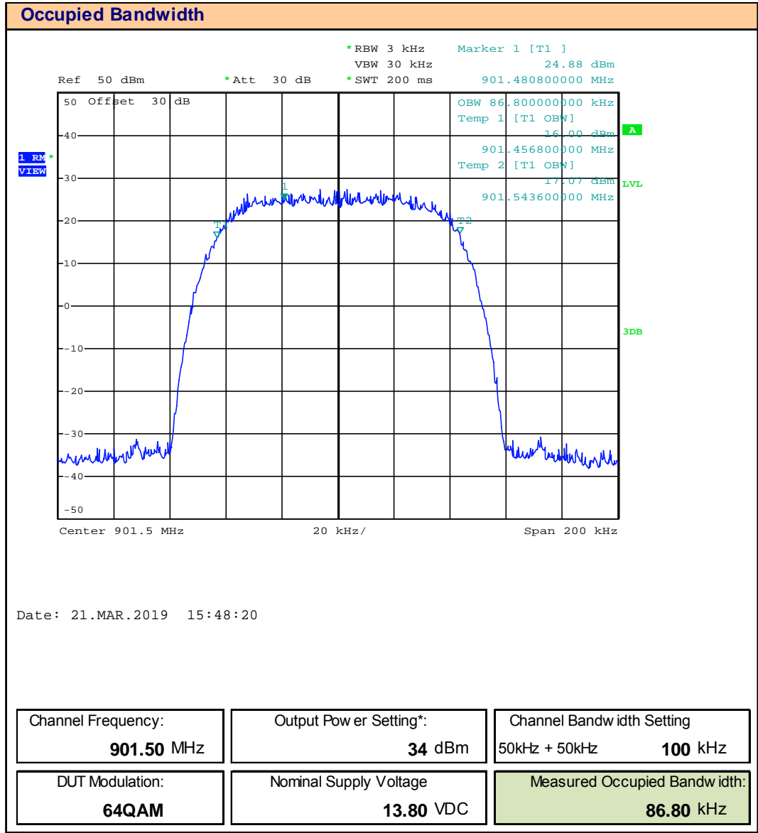
Plot 8.3 – Occupied Bandwidth – 901.5MHz, 100kHz BW, 64QAM
