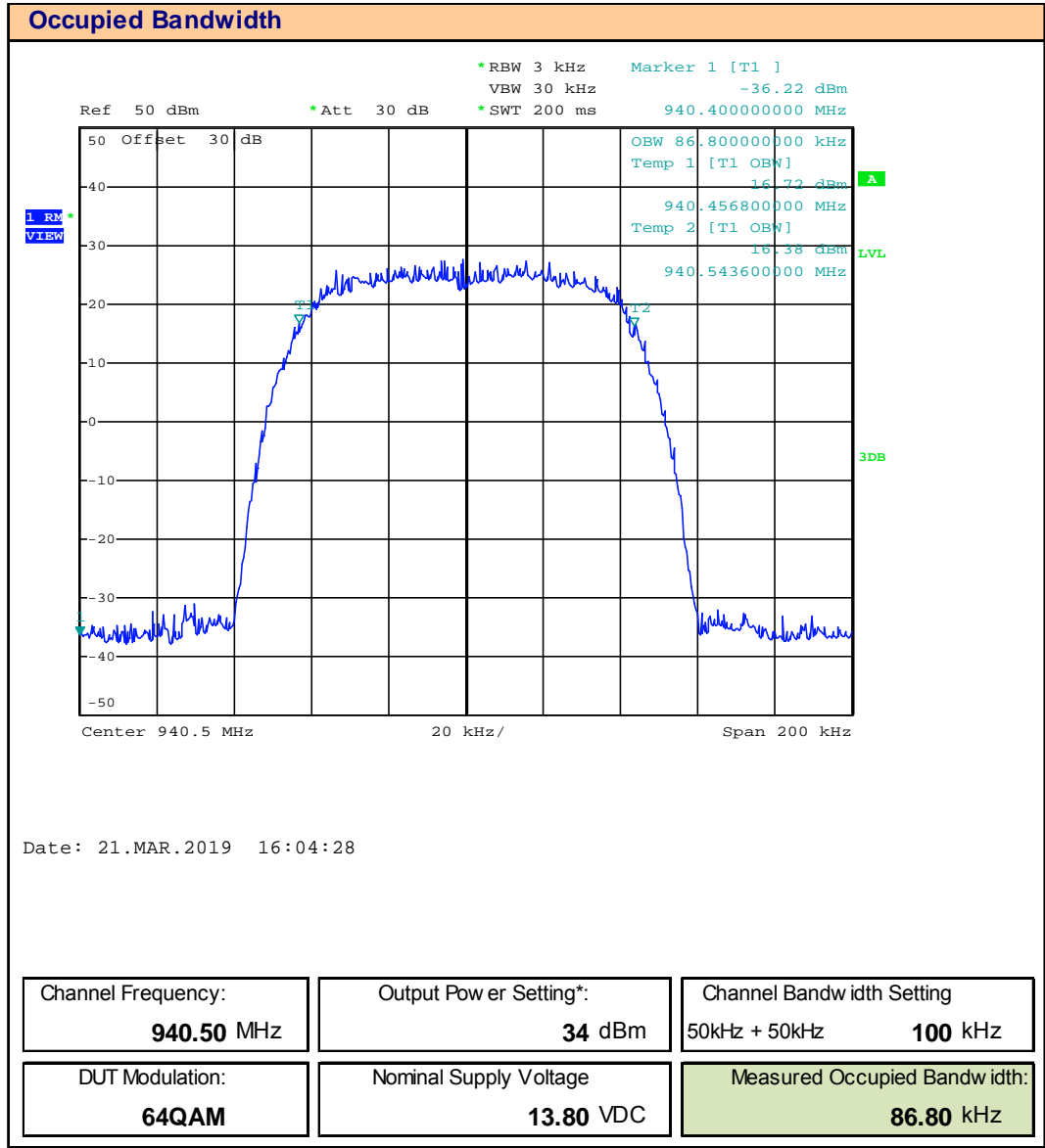
Plot 8.9 – Occupied Bandwidth – 940.5MHz, 100kHz BW, 64QAM
