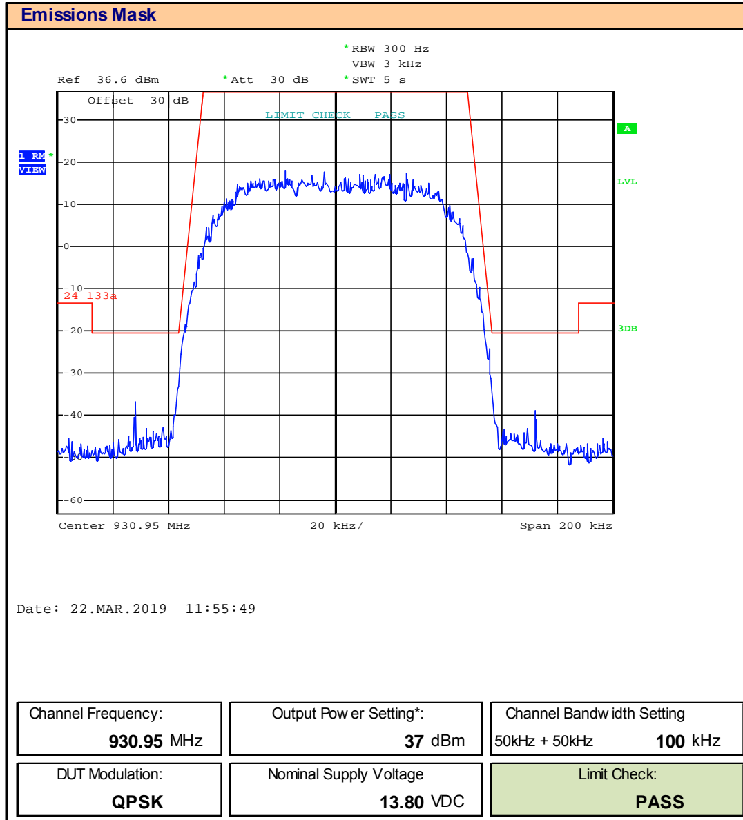
Plot 9.16 – Emissions Mask – 930.95, 100kHz BW, QPSK
