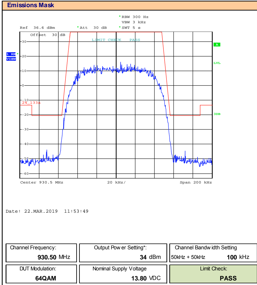
Plot 9.15 – Emissions Mask – 930.5, 100kHz BW, 64QAM
