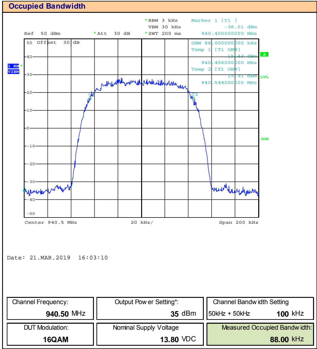
Plot 8.8 – Occupied Bandwidth – 940.5MHz, 100kHz BW, 16QAM
