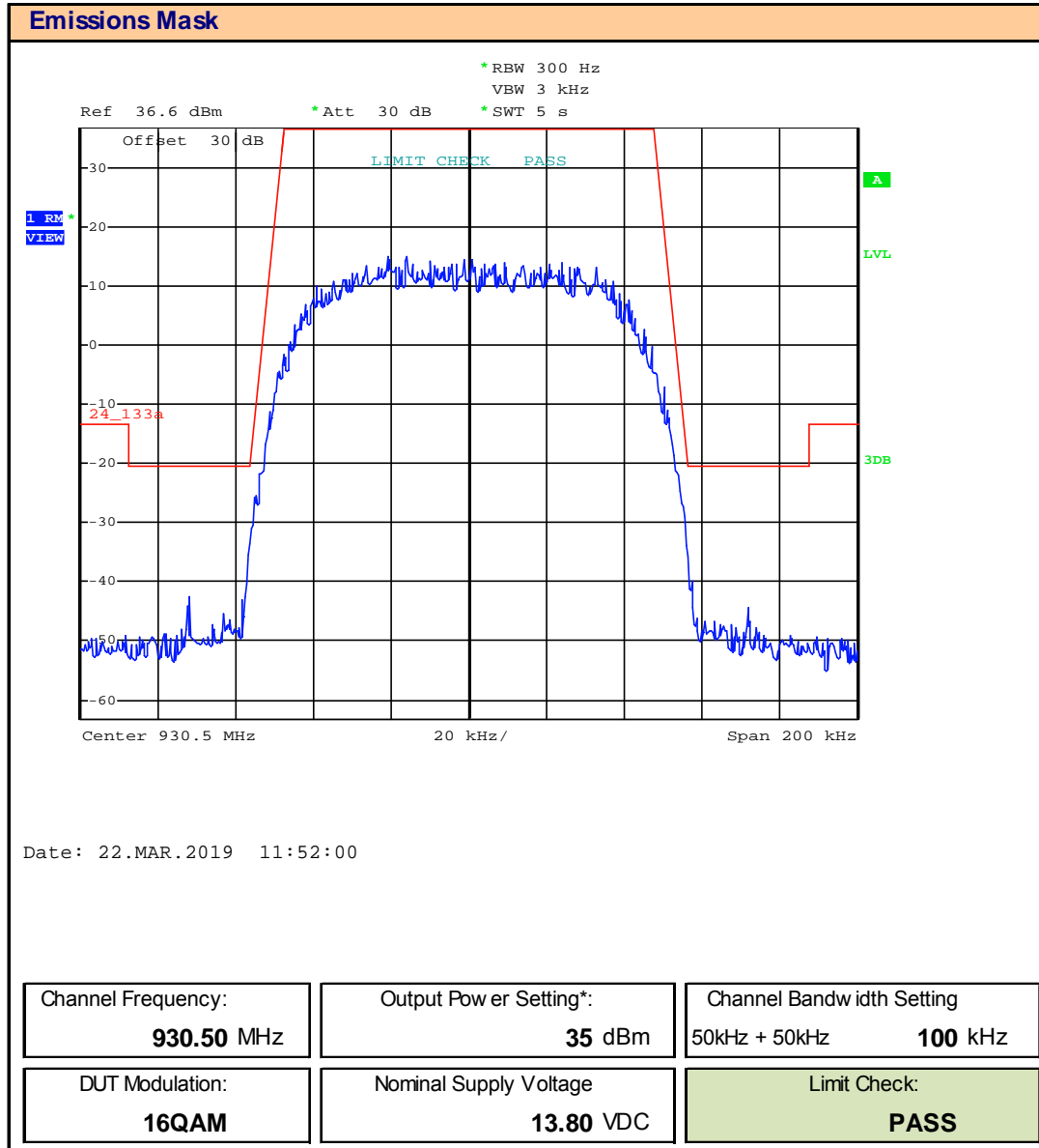
Plot 9.14 – Emissions Mask – 930.5, 100kHz BW, 16QAM
