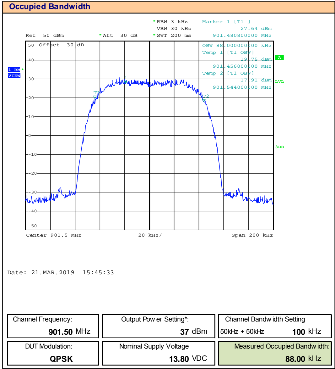
Plot 8.1 – Occupied Bandwidth – 901.5MHz, 100kHz BW, QPSK
