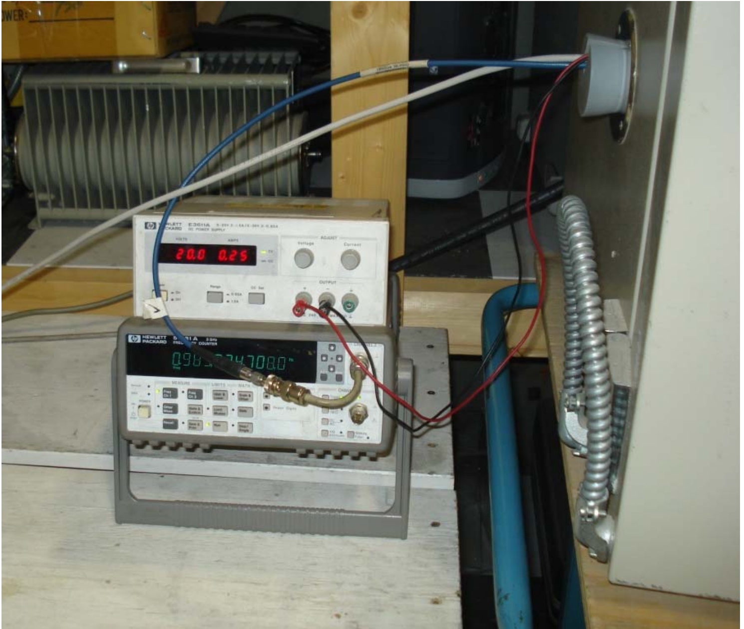
Setup – Frequency Stability
