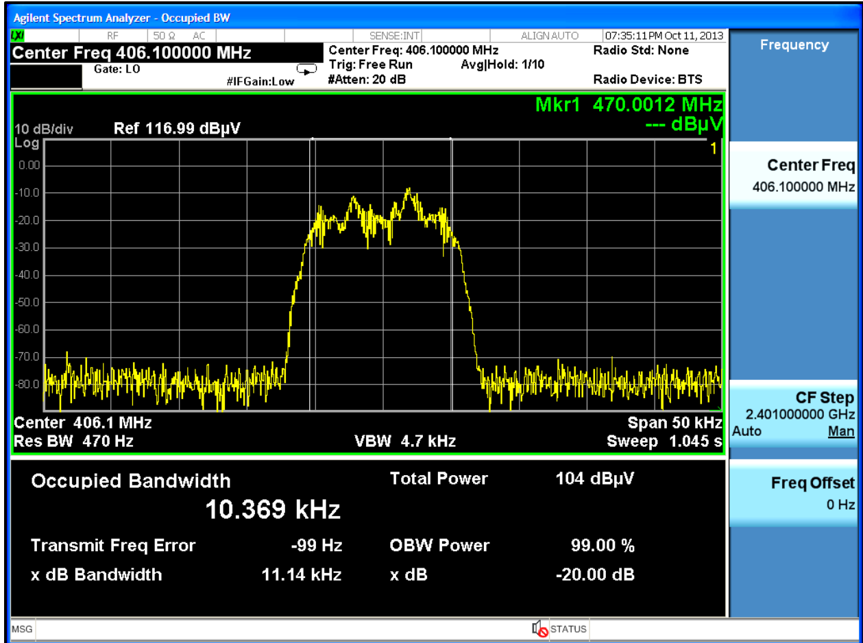
Plot 11-1: Occupied Bandwidth 406.1 MHz; 12.5 kHz Channel Spacing
