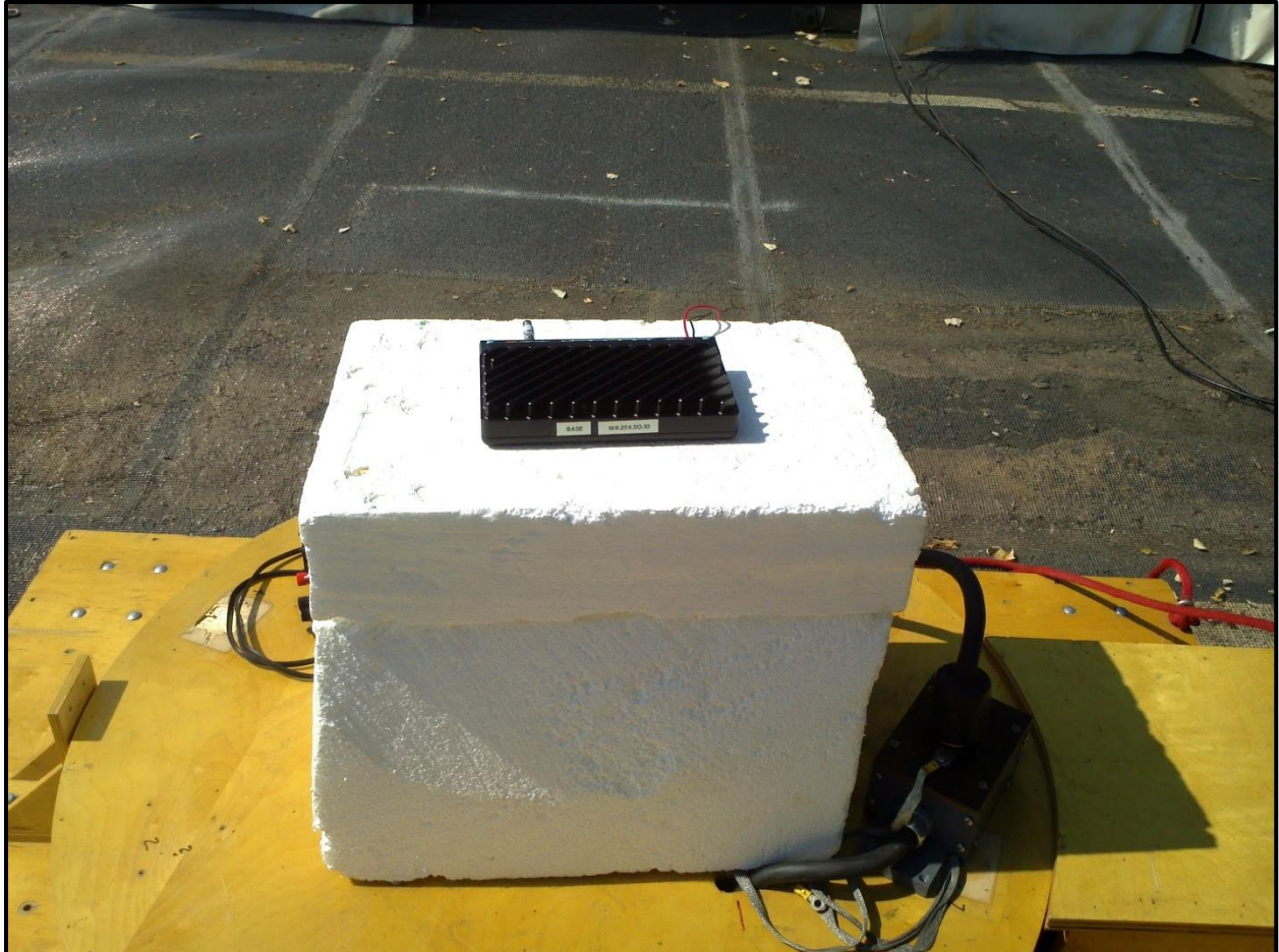
Photograph 1: Radiated Emissions (Spurious/Harmonics) – Front View
