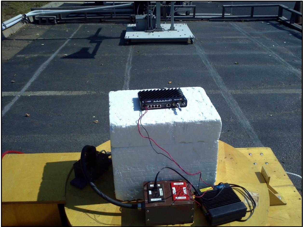
Photograph 2: Radiated Emissions (Spurious/Harmonics) – Back View
