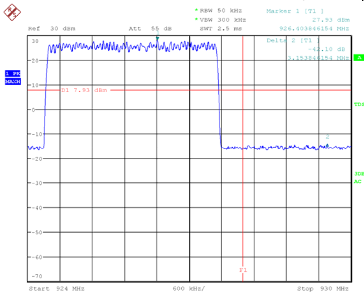
Hopping modulation active
