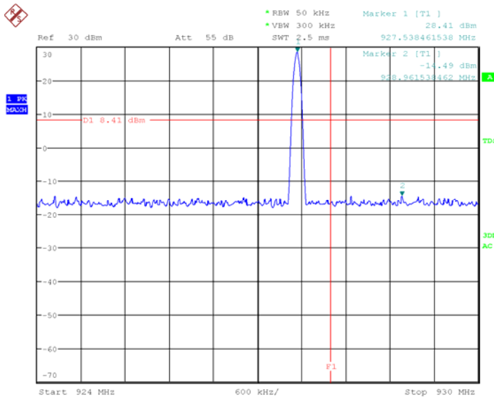
Highest channel transmitting
