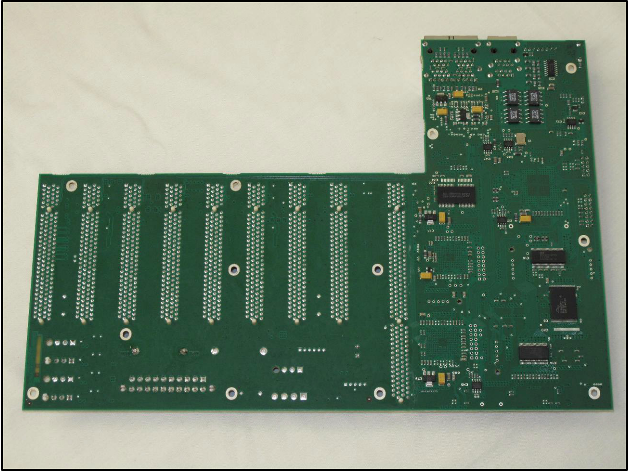
Motherboard Bottom
