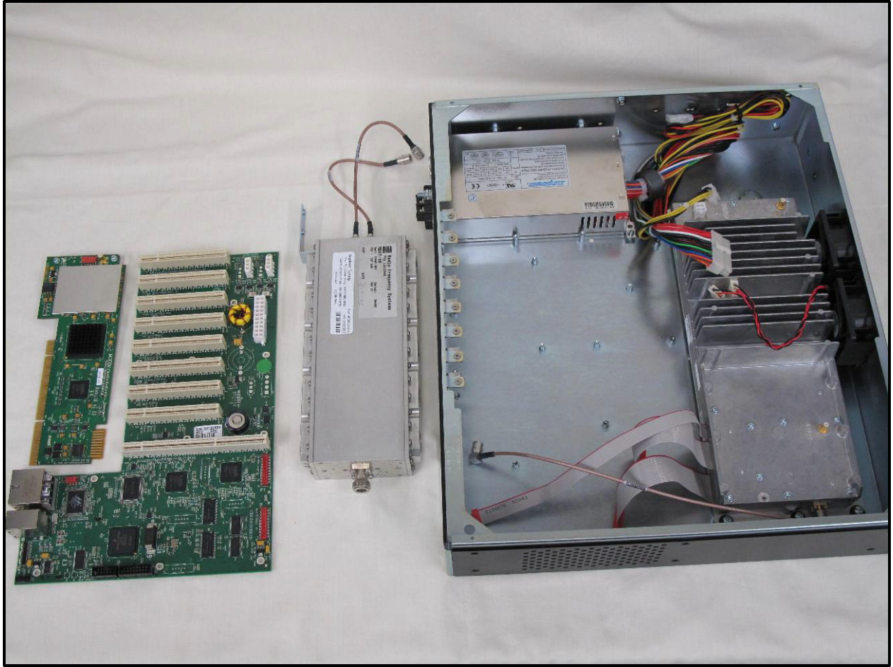
Internal Assembly 4
