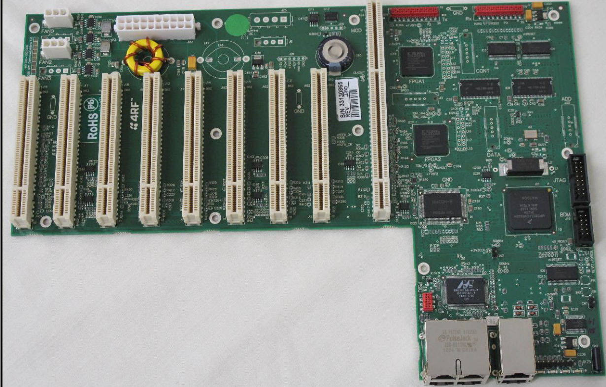
Motherboard Top
