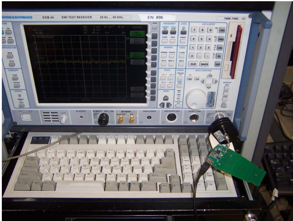
Antenna Conducted Emissions, Occupied Bandwidth, Power Output, Power Spectral Density Setup
