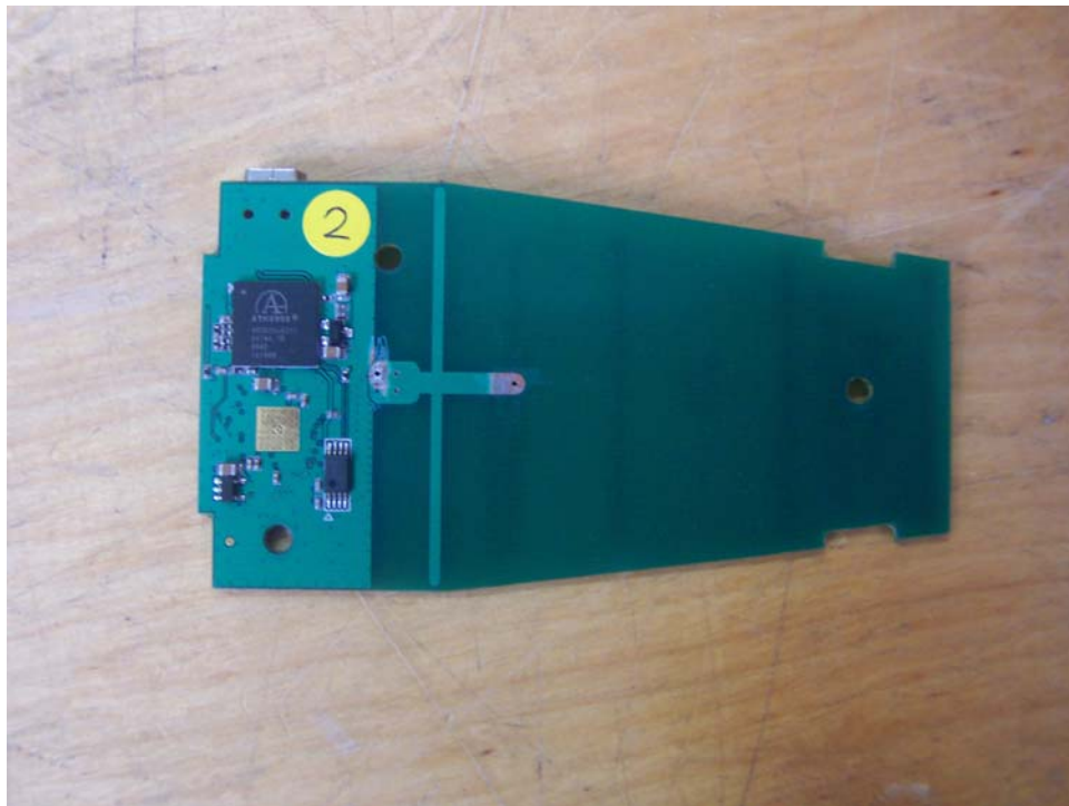
EUT Bottom View of Circuit Board
