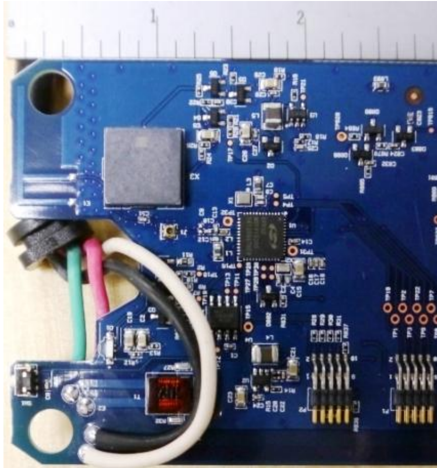
Main PCB – Side 2 – Close-up 1
