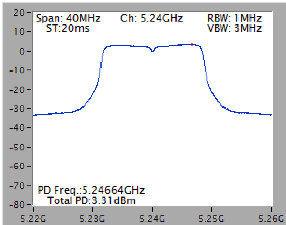
Power Density Plot on Configuration IEEE 802.11a / Ant. 3 + Ant. 4 / 5240 MHz
