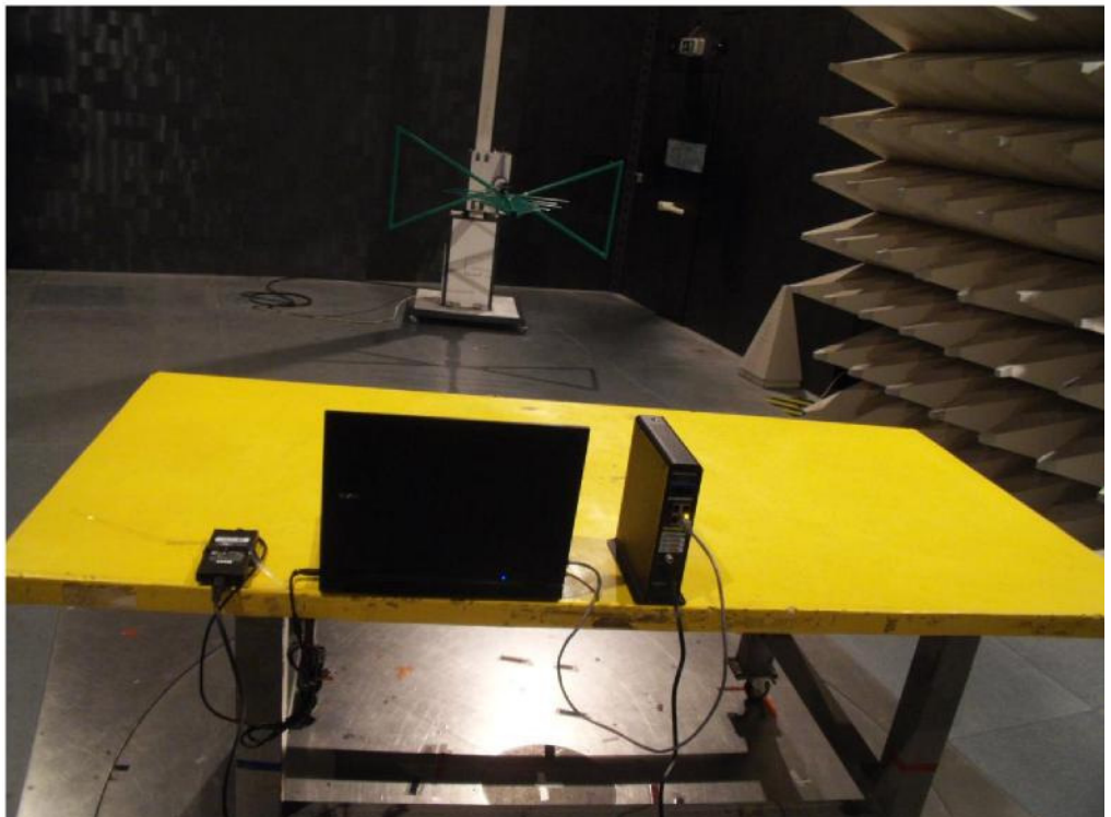
Figure 5: Radiated Emissions above 1GHz – Front and Back Views
