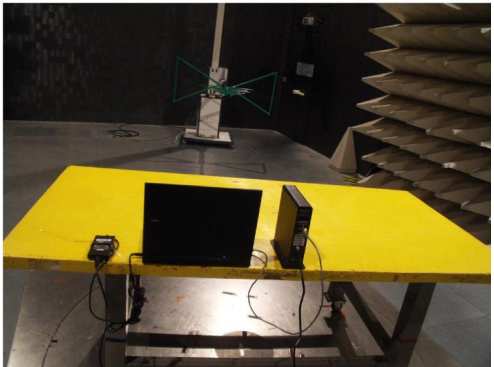
Figure 4: Radiated Emissions 30 MHz~1GHz – Front and Back Views
