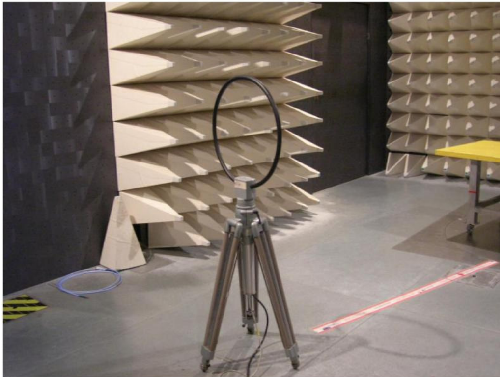
Figure 3: Radiated Emissions 9kHz~30MHz – Front and Back Views
