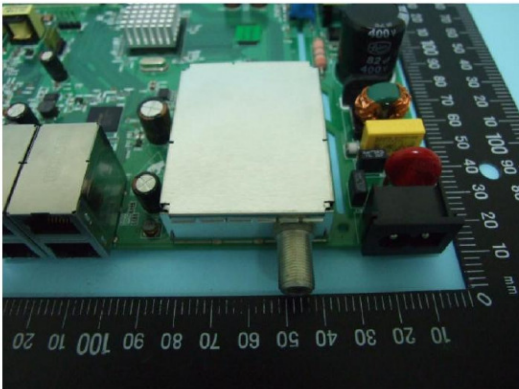
Figure 6: PCB – Close-up
