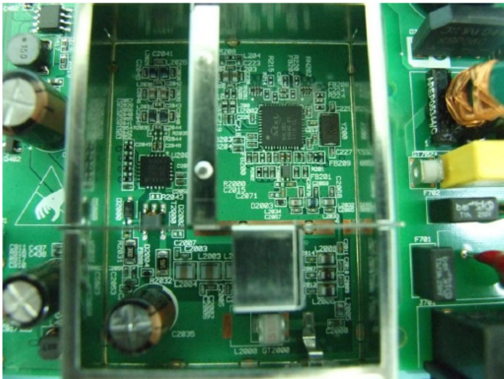
Figure 8: PCB – Without Shields
