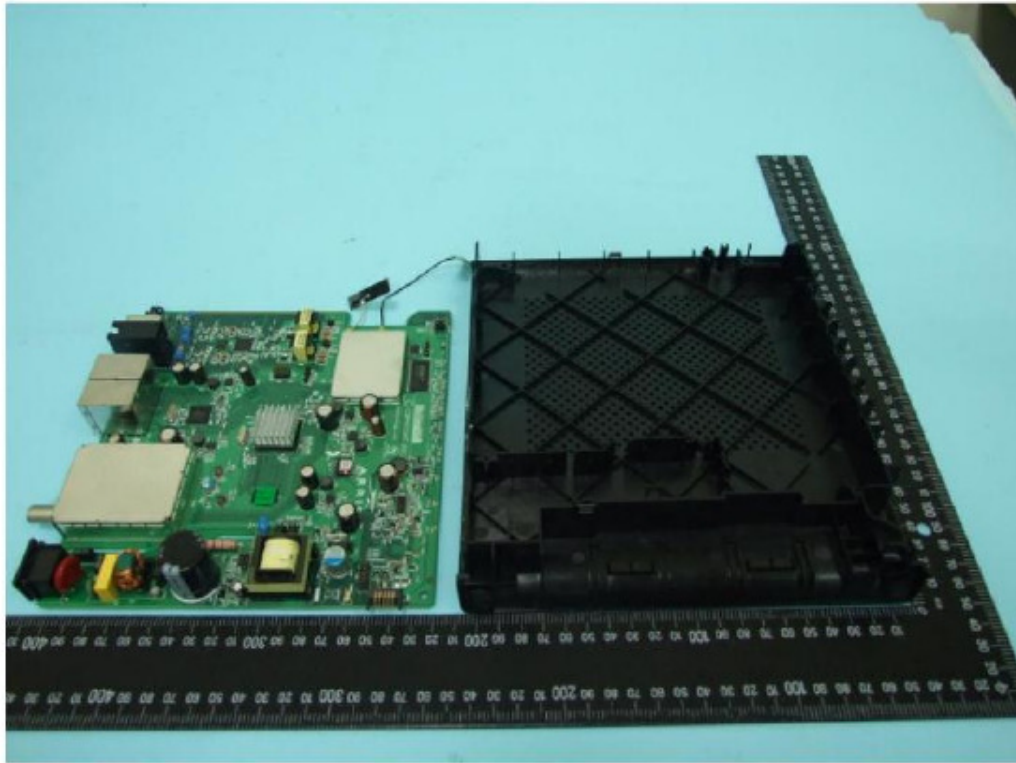
Figure 3: Internal – PCB Removed
