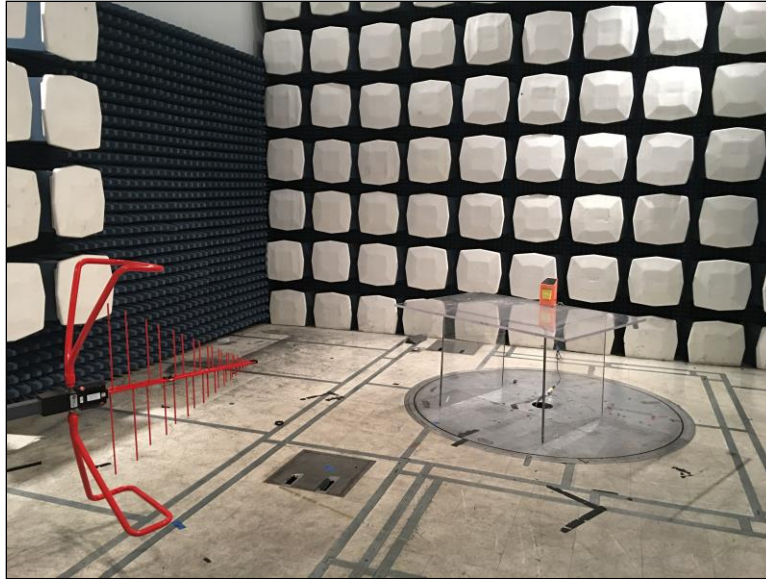
Photograph 2. Radiated Spurious Emissions, Test Setup, 30 MHz -1 GHz
