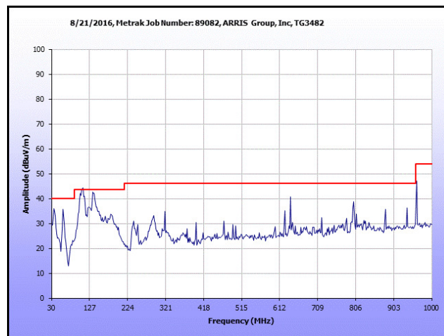
Plot 70. Radiated Spurious Emissions, 30 MHz – 1 GHz, Radio On
