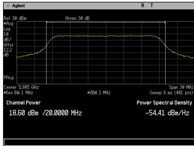
Plot 23. Conducted Output Power, 802.11n 20 MHz, Channel 5805 MHz, 4x8, MCS0 NSS1, CH3
