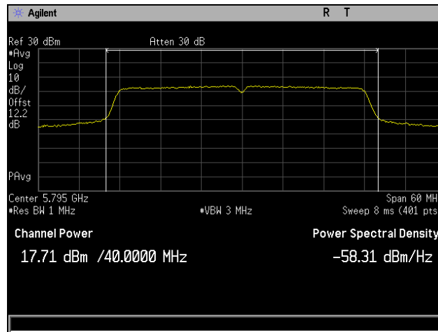
Plot 34. Conducted Output Power, 802.11ac 40 MHz, Channel 5795 MHz, 8x8, MCS0 NSS1, CH1
