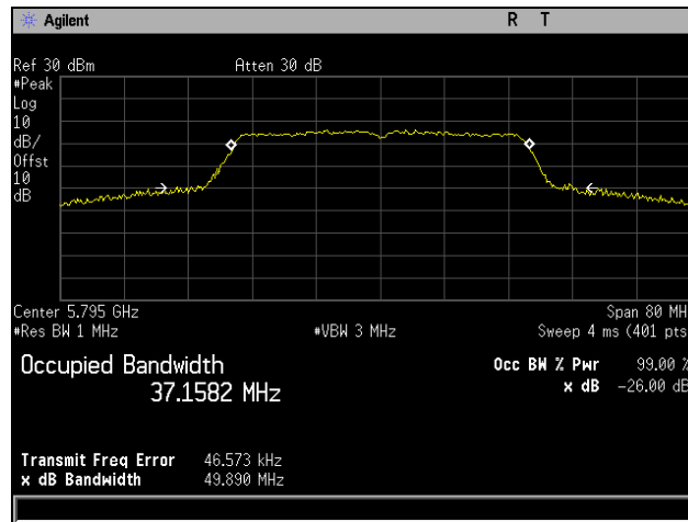
Plot 12. 26 dB Occupied Bandwidth, 802.11n 40 MHz, Channel 5795 MHz, MCS0
