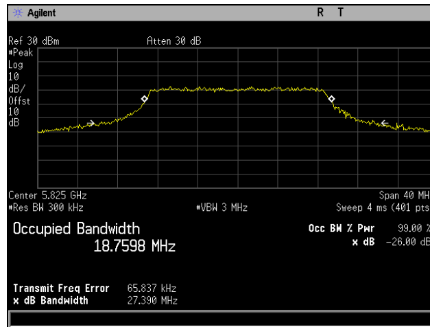
Plot 4. 26 dB Occupied Bandwidth, 802.11ac 20 MHz, Channel 5825 MHz, NSS1 MCS0
