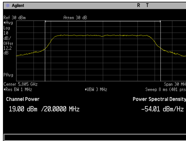
Plot 14. Conducted Output Power, 802.11a 20 MHz, Channel 5805 MHz, 4x8, 6M, CH3
