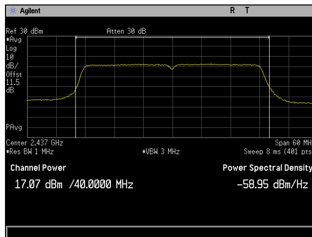
Plot 25. Peak Power Output, 802.11n 40 MHz, Channel 2437 MHz, 2x2, MCS0, CH7
