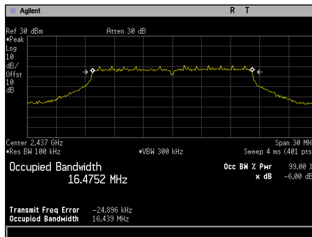
Plot 7. 6 dB Occupied Bandwidth, 802.11g 20 MHz, Channel 2437 MHz, 2x2, 6M
