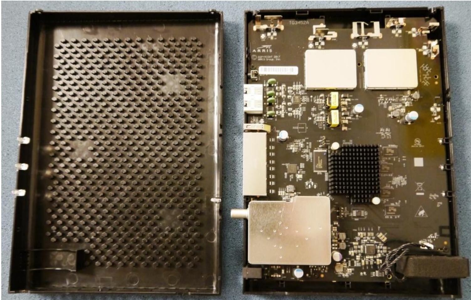
Open cover view - Top
