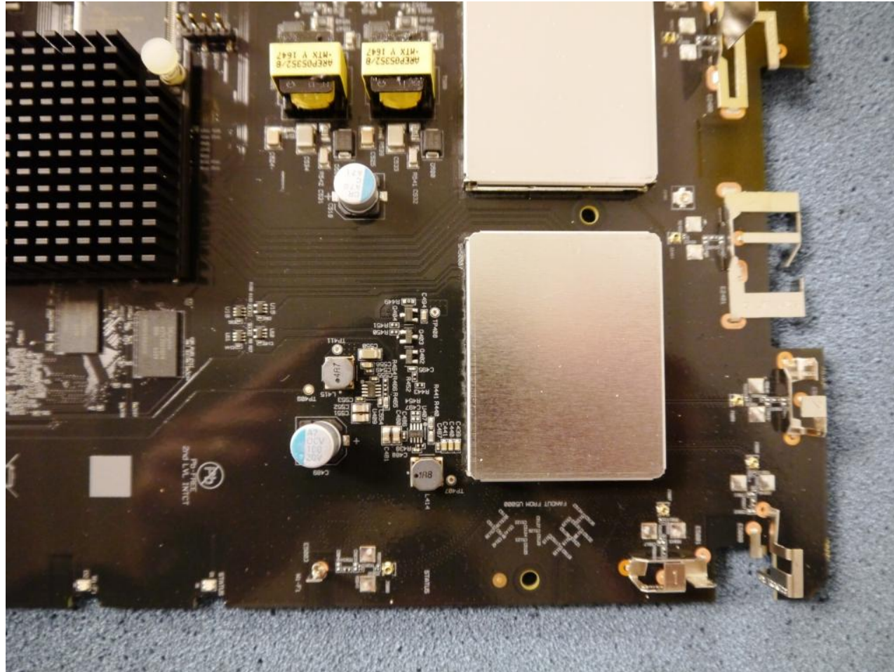
PCB Top – Lower / Right Quadrant
