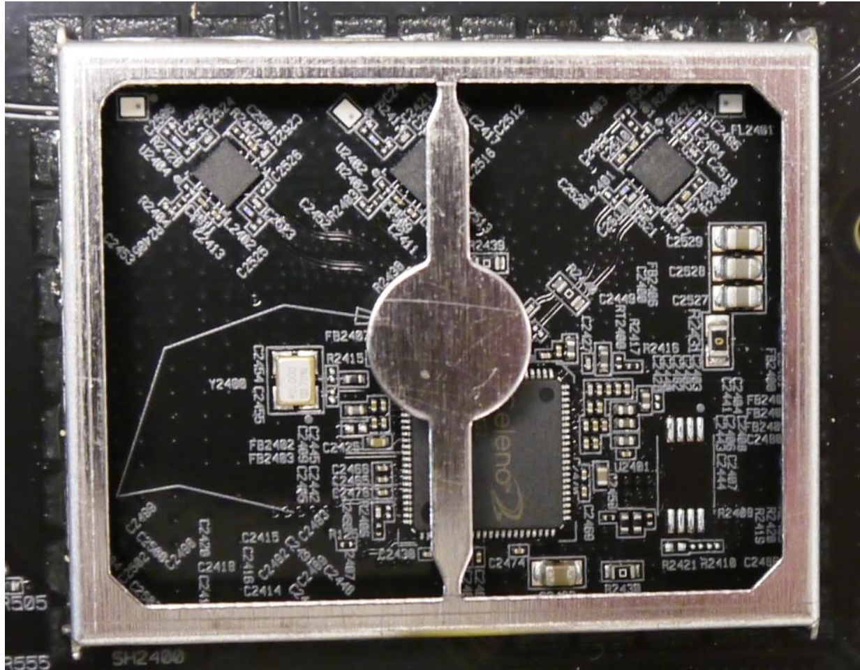
2.4GHz Radio – Can Removed
