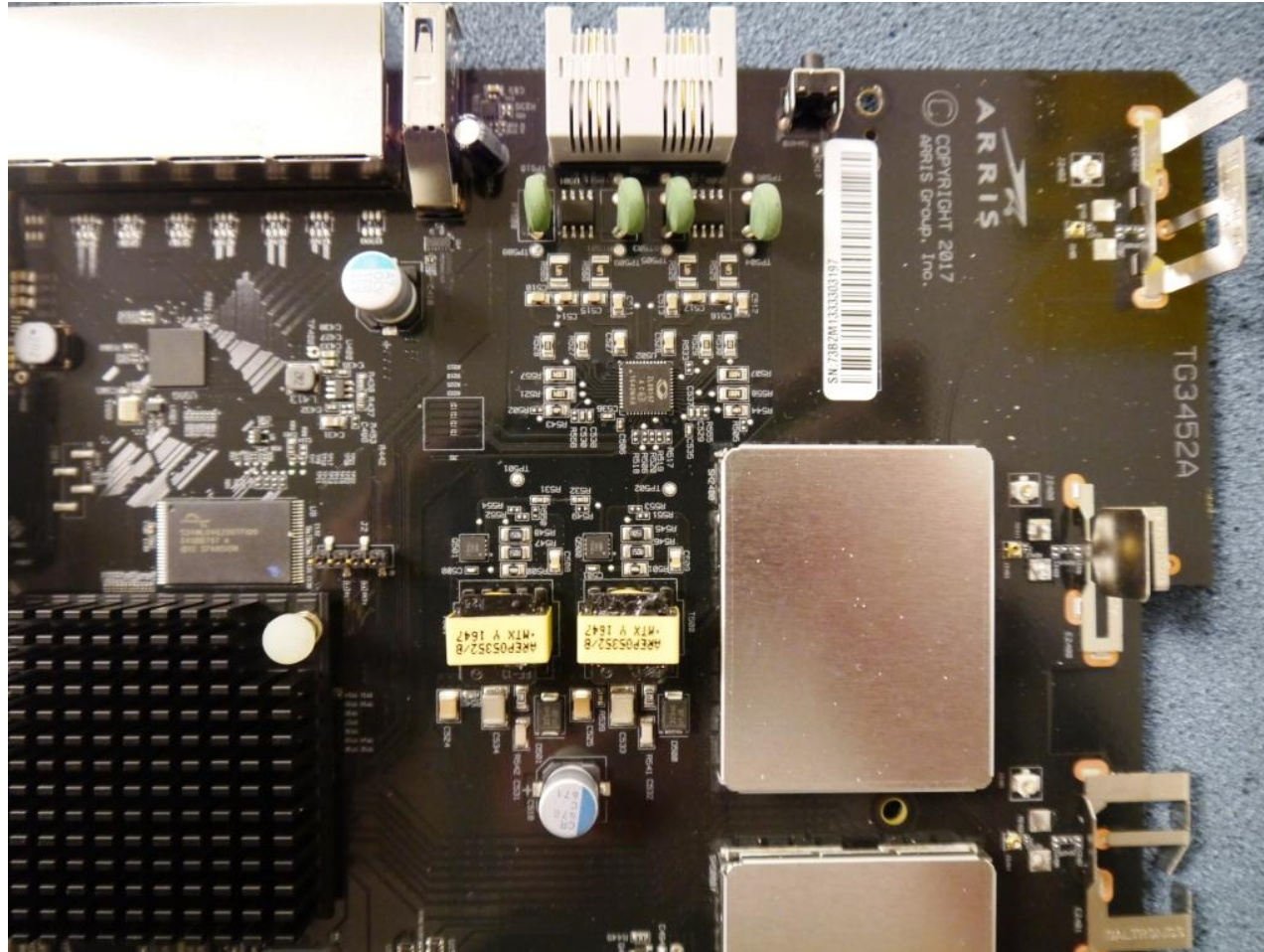
PCB Top – Upper / Right Quadrant
