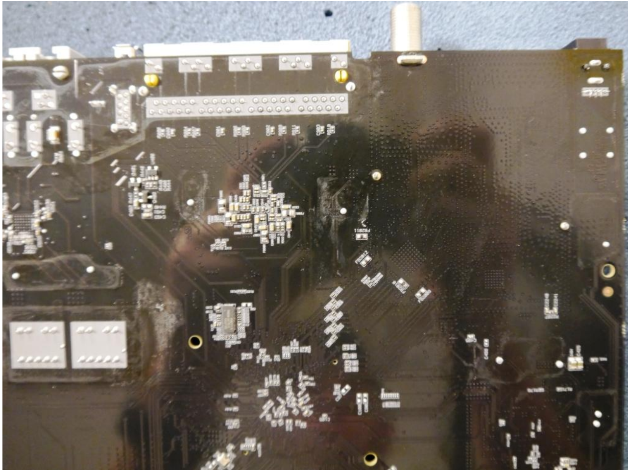
PCB Bottom – Upper / Right Quadrant
