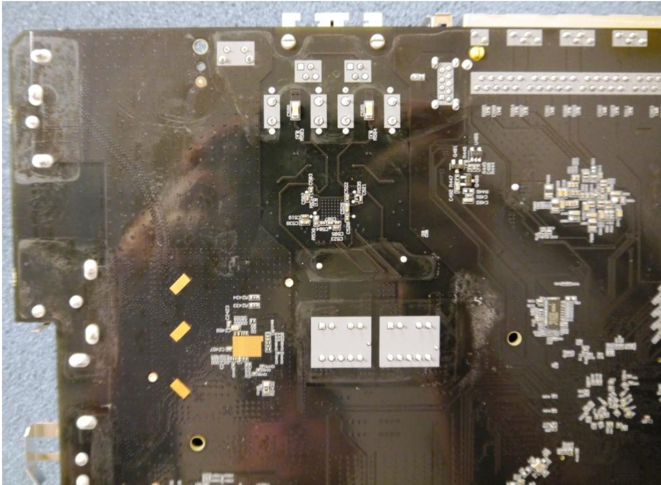
PCB Bottom – Upper / Left Quadrant
