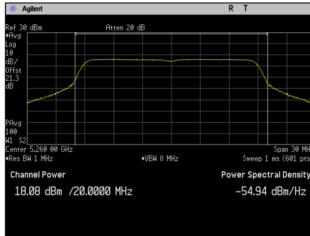
Plot 8. Conducted Output Power, 5260 MHz, 802.11ac 20 MHz, Port 1
