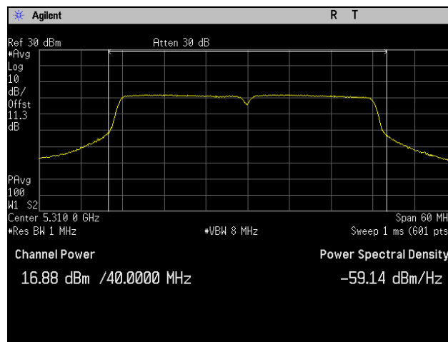
Plot 60. Conducted Output Power, 5310 MHz, 802.11ac 40 MHz, Port 2
