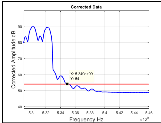
Plot 342. Radiated Band Edge, 5290 MHz, 802.11ac 80 MHz, Average
