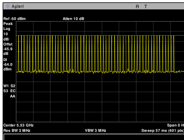
Plot 353. Radar Waveform Calibration, 5530 MHz, Type 1
