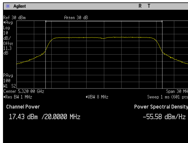
Plot 54. Conducted Output Power, 5320 MHz, 802.11n 20 MHz, Port 2
