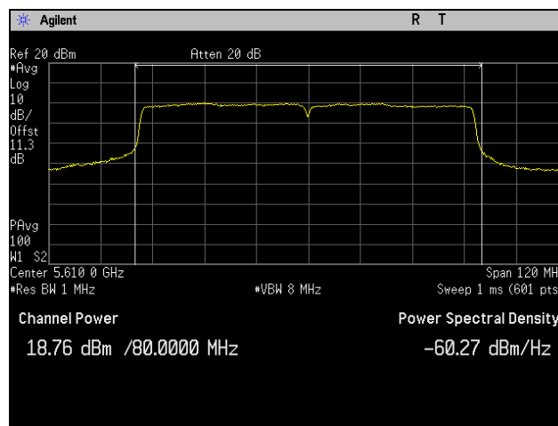
Plot 36. Conducted Output Power, 5610 MHz, 802.11ac 80 MHz, Port 1
