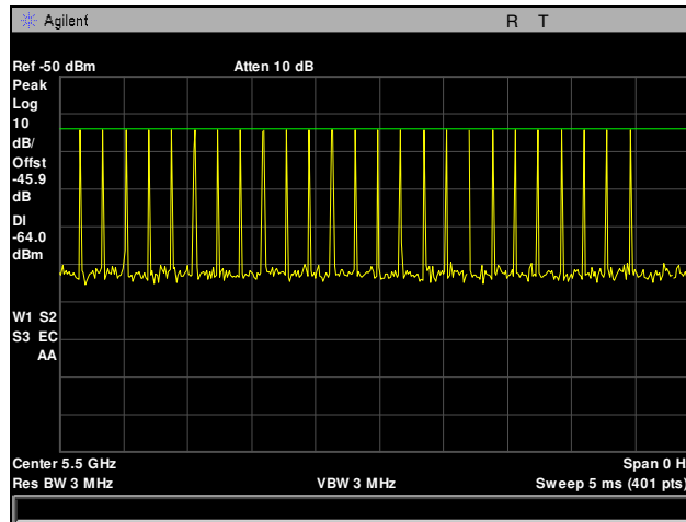
Plot 354. Radar Waveform Calibration, 5500 MHz, Type 2
