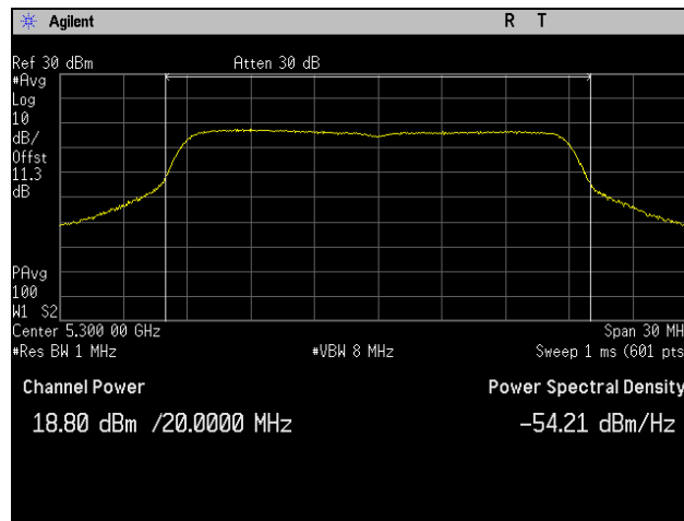
Plot 53. Conducted Output Power, 5300 MHz, 802.11n 20 MHz, Port 2
