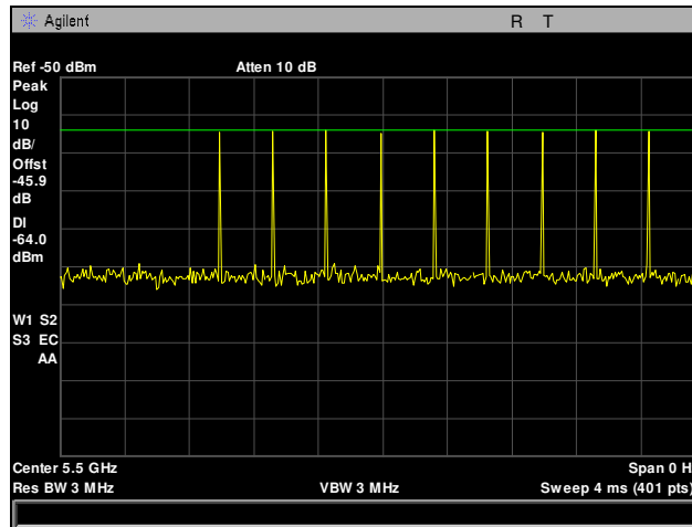
Plot 366. Radar Waveform Calibration, 5500 MHz, Type 6
