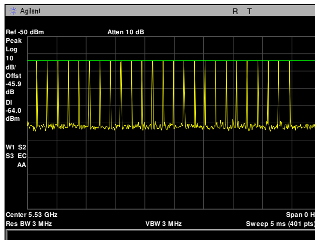
Plot 356. Radar Waveform Calibration, 5530 MHz, Type 2
