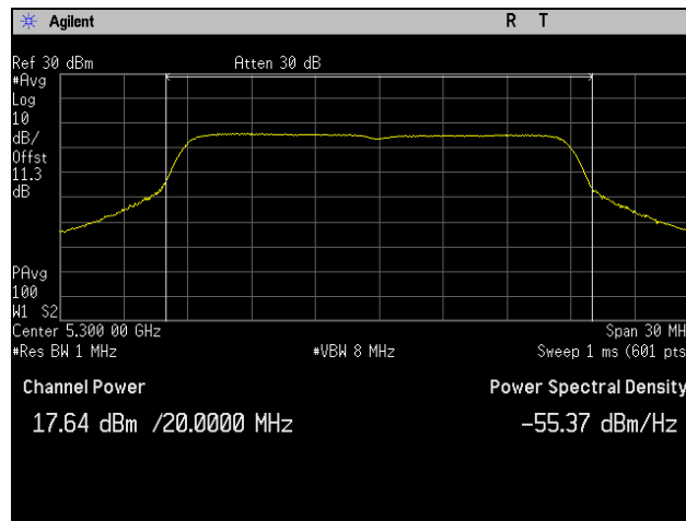
Plot 46. Conducted Output Power, 5300 MHz, 802.11ac 20 MHz, Port 2
