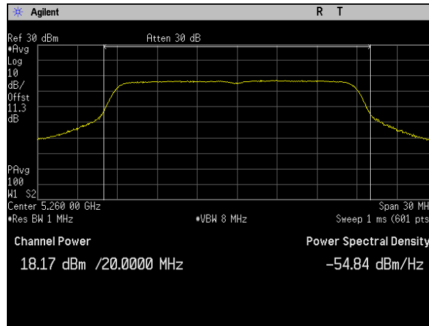
Plot 45. Conducted Output Power, 5260 MHz, 802.11ac 20 MHz, Port 2
