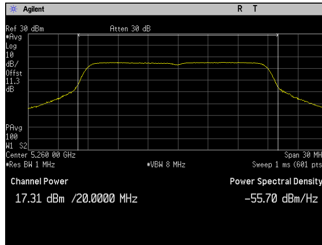
Plot 82. Conducted Output Power, 5260 MHz, 802.11ac 20 MHz, Port 3
