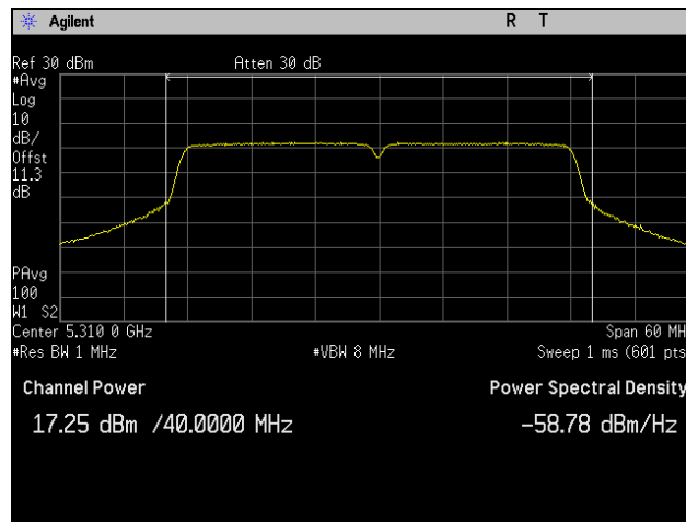
Plot 29. Conducted Output Power, 5310 MHz, 802.11n 40 MHz, Port 1
