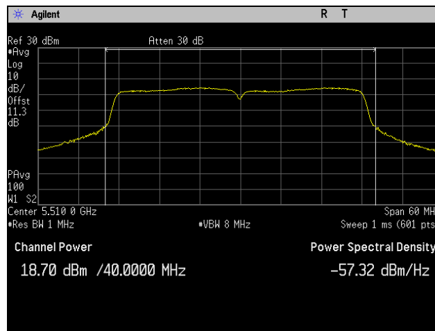
Plot 30. Conducted Output Power, 5510 MHz, 802.11n 40 MHz, Port 1
