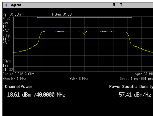
Plot 24. Conducted Output Power, 5510 MHz, 802.11ac 40 MHz, Port 1
