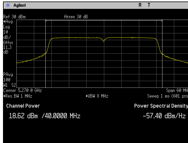
Plot 28. Conducted Output Power, 5270 MHz, 802.11n 40 MHz, Port 1
