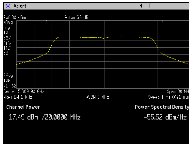
Plot 39. Conducted Output Power, 5300 MHz, 802.11a 20 MHz, Port 2
