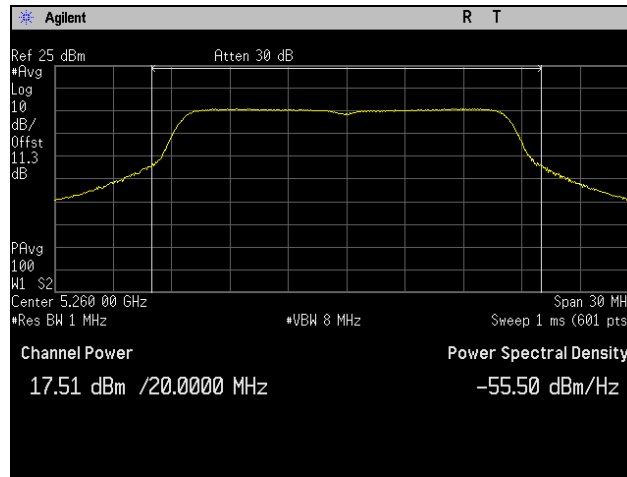
Plot 38. Conducted Output Power, 5260 MHz, 802.11a 20 MHz, Port 2
