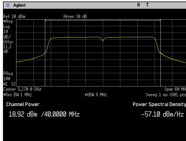
Plot 102. Conducted Output Power, 5270 MHz, 802.11n 40 MHz, Port 3
