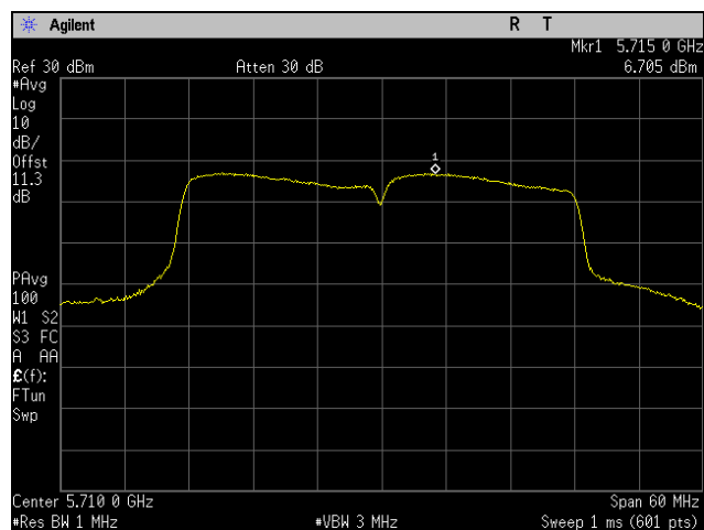
Plot 138. Peak Power Spectral Density, 5710 MHz, 802.11ac 40 MHz, Port 1
