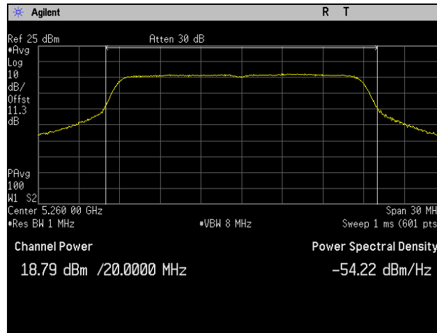
Plot 52. Conducted Output Power, 5260 MHz, 802.11n 20 MHz, Port 2
