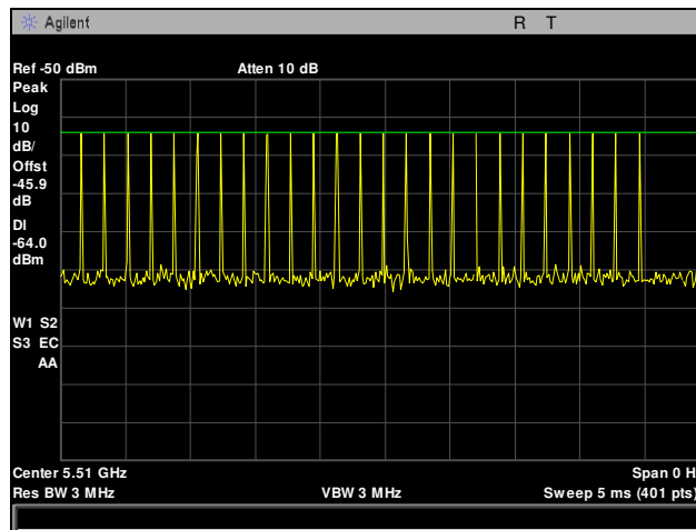
Plot 355. Radar Waveform Calibration, 5510 MHz, Type 2
