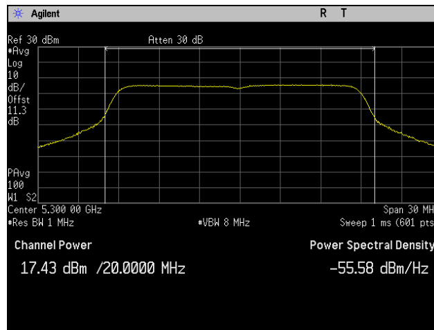
Plot 83. Conducted Output Power, 5300 MHz, 802.11ac 20 MHz, Port 3
