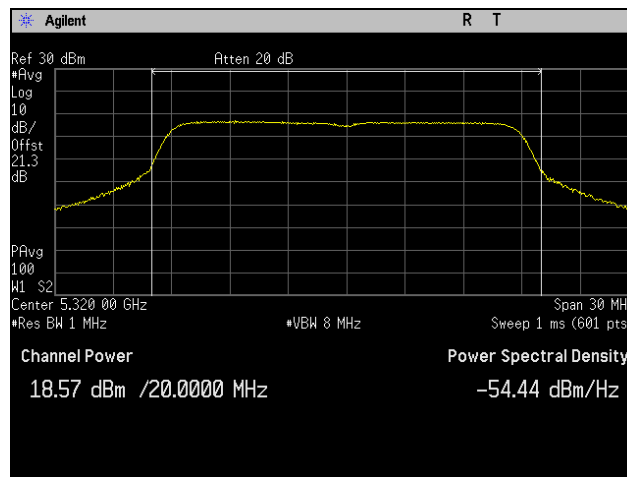
Plot 10. Conducted Output Power, 5320 MHz, 802.11ac 20 MHz, Port 1
