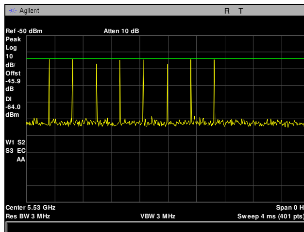
Plot 368. Radar Waveform Calibration, 5530 MHz, Type 6
