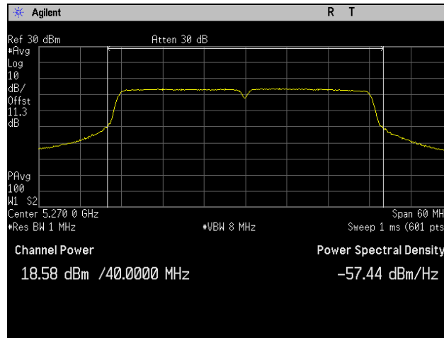
Plot 65. Conducted Output Power, 5270 MHz, 802.11n 40 MHz, Port 2
