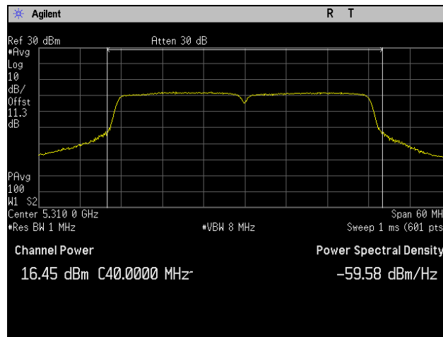
Plot 66. Conducted Output Power, 5310 MHz, 802.11n 40 MHz, Port 2
