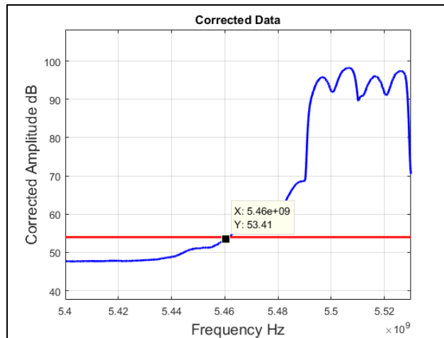
Plot 333. Radiated Band Edge, 5510 MHz, 802.11ac 40 MHz, Average
