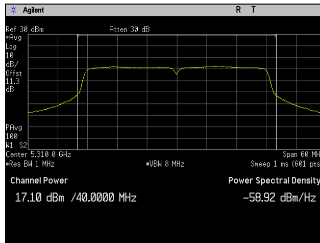
Plot 103. Conducted Output Power, 5310 MHz, 802.11n 40 MHz, Port 3
