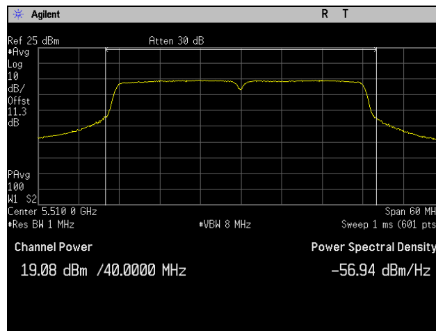
Plot 61. Conducted Output Power, 5510 MHz, 802.11ac 40 MHz, Port 2
