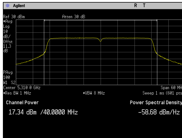
Plot 23. Conducted Output Power, 5310 MHz, 802.11ac 40 MHz, Port 1
