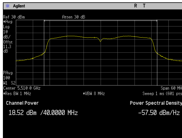
Plot 104. Conducted Output Power, 5510 MHz, 802.11n 40 MHz, Port 3
