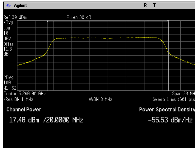
Plot 89. Conducted Output Power, 5260 MHz, 802.11n 20 MHz, Port 3
