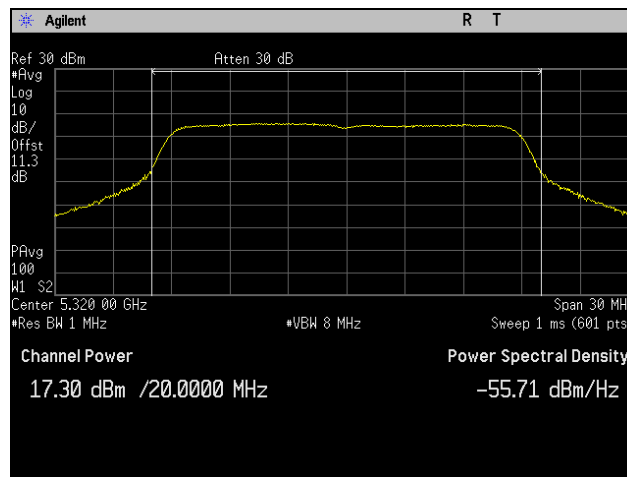
Plot 91. Conducted Output Power, 5320 MHz, 802.11n 20 MHz, Port 3
