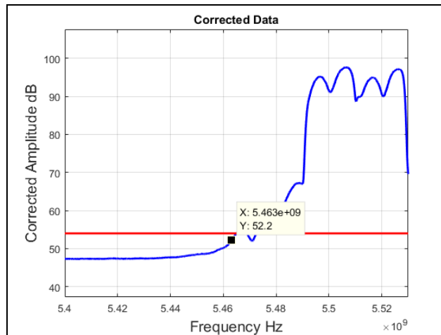
Plot 339. Radiated Band Edge, 5510 MHz, 802.11n 40 MHz, Average
