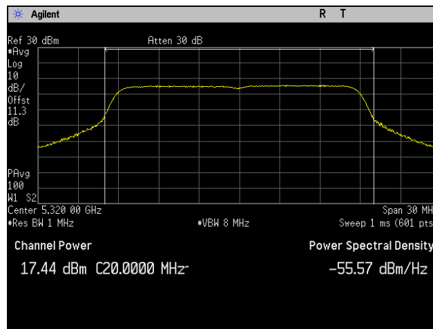
Plot 47. Conducted Output Power, 5320 MHz, 802.11ac 20 MHz, Port 2
