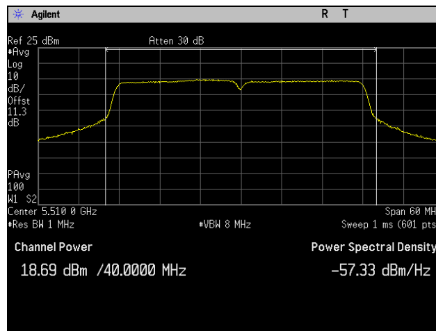
Plot 67. Conducted Output Power, 5510 MHz, 802.11n 40 MHz, Port 2
