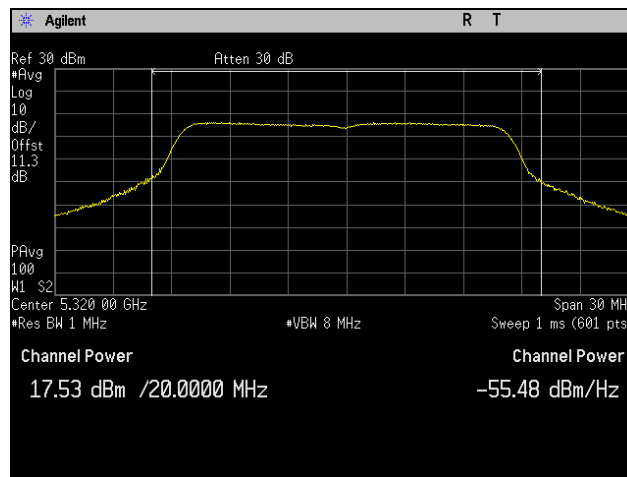
Plot 40. Conducted Output Power, 5320 MHz, 802.11a 20 MHz, Port 2
