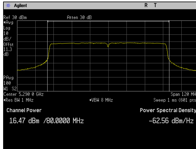
Plot 34. Conducted Output Power, 5290 MHz, 802.11ac 80 MHz, Port 1
