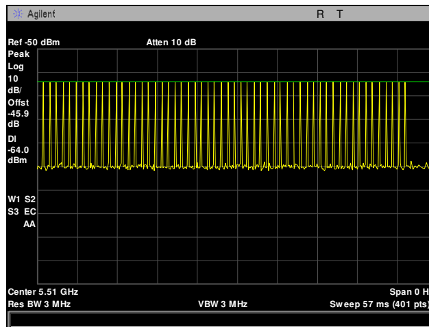
Plot 352. Radar Waveform Calibration, 5510 MHz, Type 1
