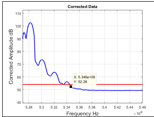
Plot 335. Radiated Band Edge, 5270 MHz, 802.11n 40 MHz, Average
