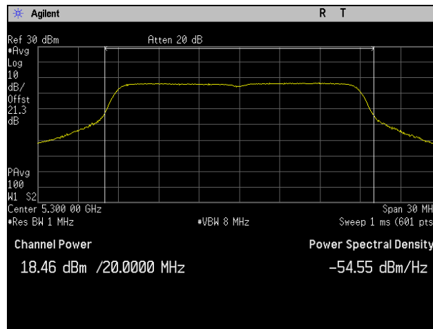
Plot 9. Conducted Output Power, 5300 MHz, 802.11ac 20 MHz, Port 1
