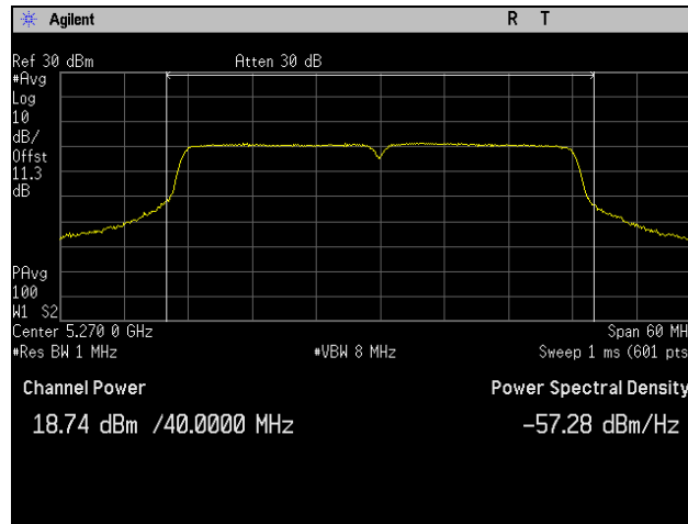
Plot 59. Conducted Output Power, 5270 MHz, 802.11ac 40 MHz, Port 2
