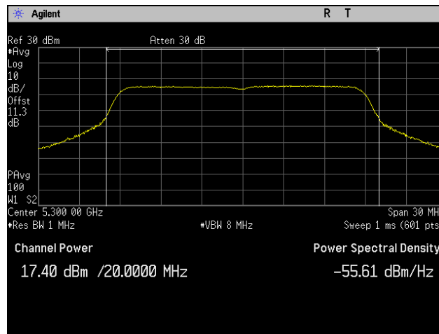
Plot 90. Conducted Output Power, 5300 MHz, 802.11n 20 MHz, Port 3
