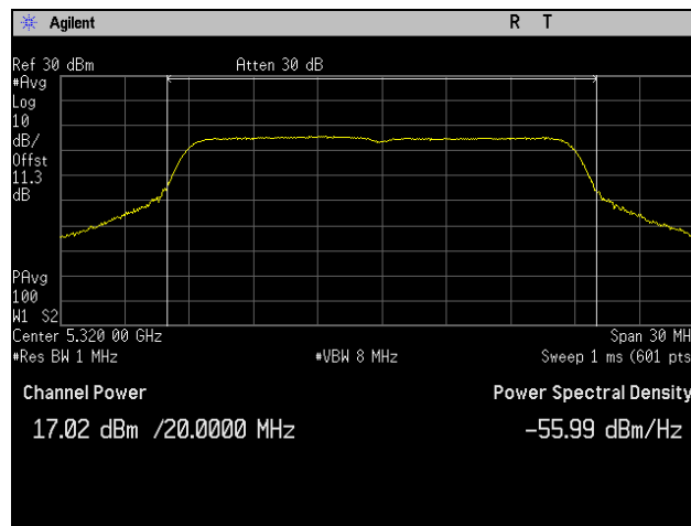
Plot 84. Conducted Output Power, 5320 MHz, 802.11ac 20 MHz, Port 3
