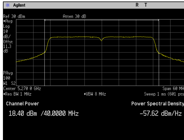
Plot 22. Conducted Output Power, 5270 MHz, 802.11ac 40 MHz, Port 1
