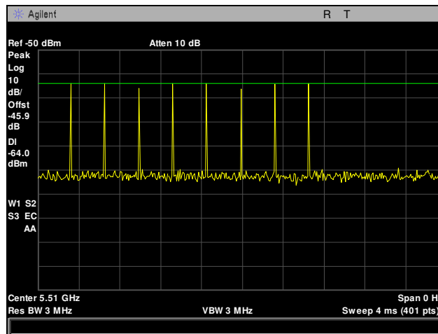
Plot 367. Radar Waveform Calibration, 5510 MHz, Type 6
