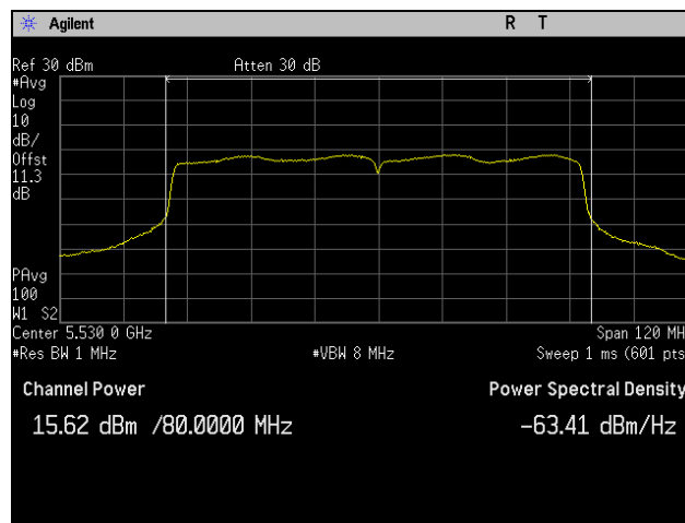
Plot 35. Conducted Output Power, 5530 MHz, 802.11ac 80 MHz, Port 1
