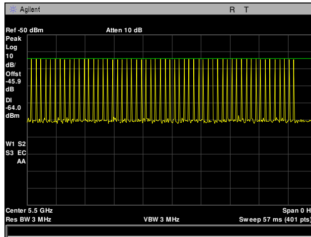
Plot 351. Radar Waveform Calibration, 5500 MHz, Type 1
