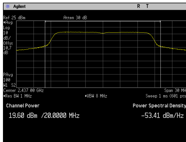
Plot 19. Peak Power Output, Mid Channel, 802.11g 20 MHz, Port 2
