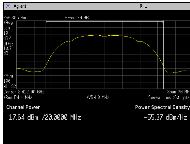
Plot 3. Peak Power Output, Low Channel, 802.11b 20 MHz, Port 1
