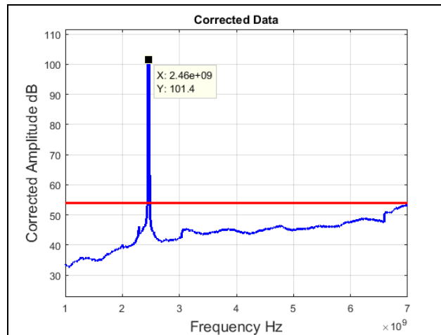
Plot 44. Radiated Spurious Emissions, High Channel, 802.11n 20 MHz, 1 GHz – 7 GHz, Average
