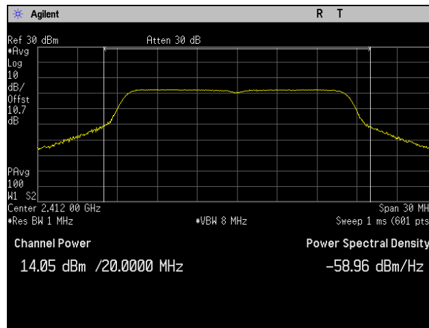
Plot 18. Peak Power Output, Low Channel, 802.11g 20 MHz, Port 2
