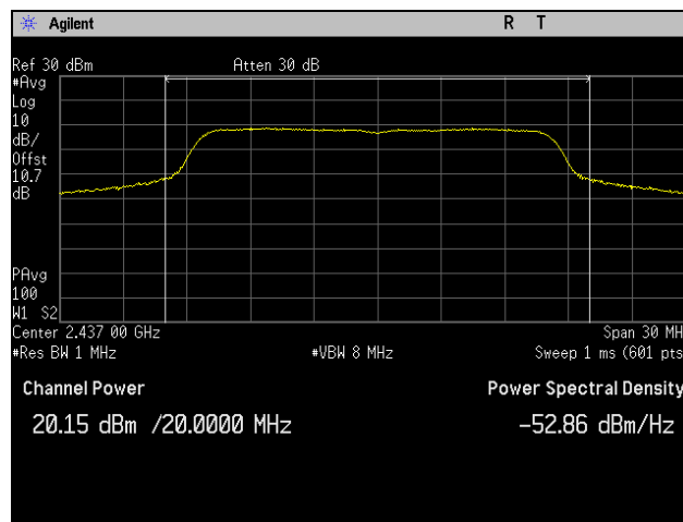
Plot 7. Peak Power Output, Mid Channel, 802.11g 20 MHz, Port 1
