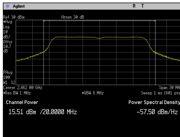
Plot 8. Peak Power Output, High Channel, 802.11g 20 MHz, Port 1
