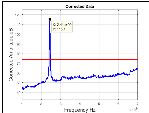
Plot 43. Radiated Spurious Emissions, Mid Channel, 802.11n 20 MHz, 1 GHz – 7 GHz, Peak
