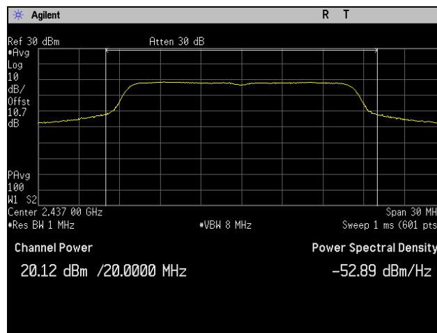
Plot 10. Peak Power Output, Mid Channel, 802.11n 20 MHz, Port 1
