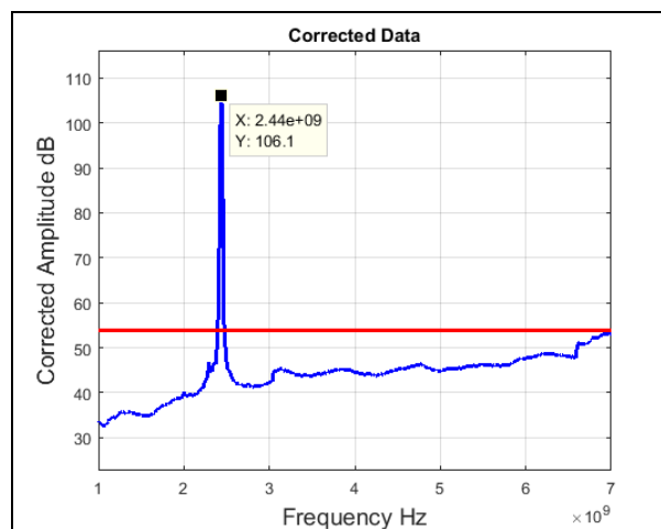
Plot 42. Radiated Spurious Emissions, Mid Channel, 802.11n 20 MHz, 1 GHz – 7 GHz, Average
