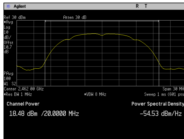
Plot 17. Peak Power Output, High Channel, 802.11b 20 MHz, Port 2
