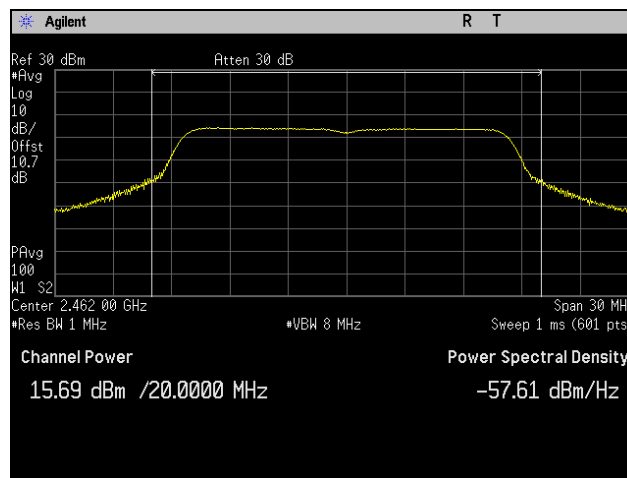
Plot 20. Peak Power Output, High Channel, 802.11g 20 MHz, Port 2
