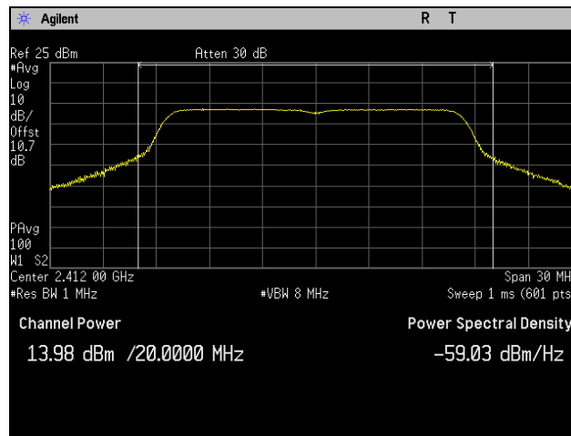
Plot 21. Peak Power Output, Low Channel, 802.11n 20 MHz, Port 2
