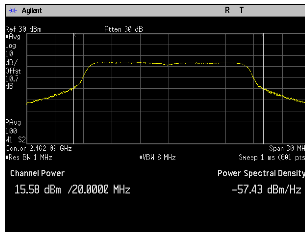
Plot 11. Peak Power Output, High Channel, 802.11n 20 MHz, Port 1
