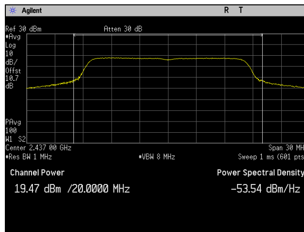
Plot 22. Peak Power Output, Mid Channel, 802.11n 20 MHz, Port 2
