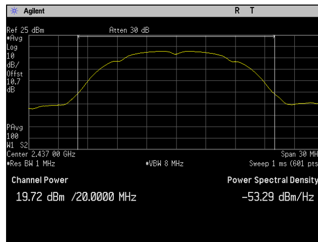
Plot 16. Peak Power Output, Mid Channel, 802.11b 20 MHz, Port 2
