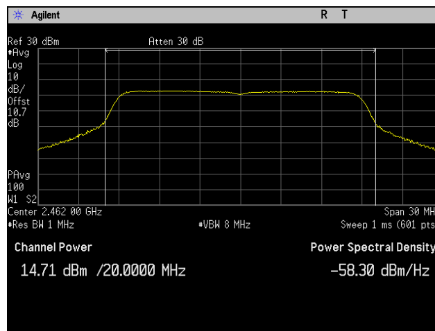
Plot 23. Peak Power Output, High Channel, 802.11n 20 MHz, Port 2
