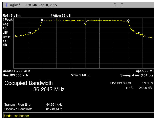
Plot 40. 26 dB Occupied Bandwidth, High Channel, 802.11n 40 MHz, Chain 1
