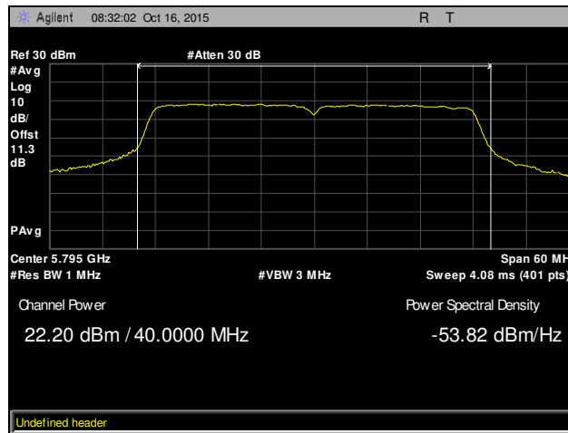
Plot 64. Maximum Conducted Output Power, High Channel, 802.11ac 40 MHz, Chain 1
