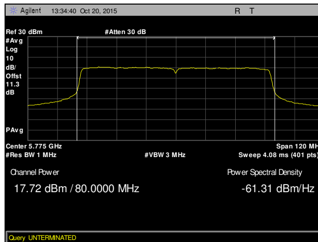
Plot 69. Maximum Conducted Output Power, Low Channel, 802.11ac 80 MHz, Chain 2
