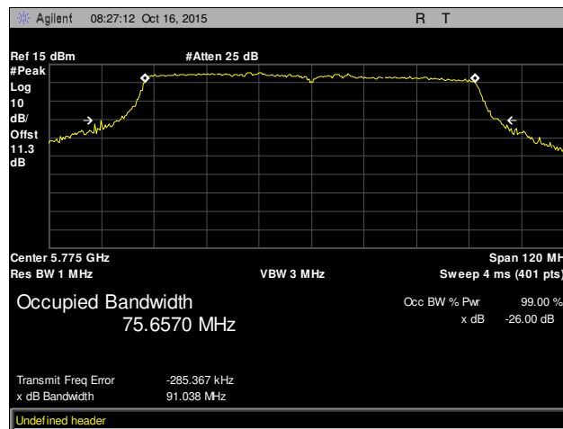
Plot 26. 26 dB Occupied Bandwidth, Channel 149, 802.11ac 80 MHz, Chain 1
