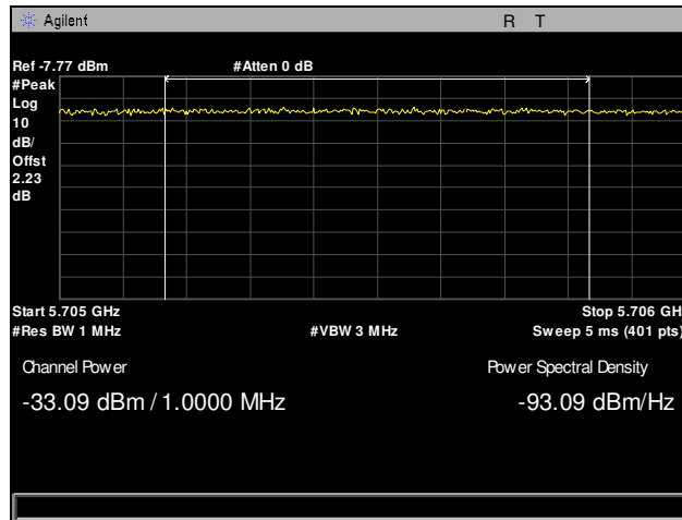
Plot 191. Radiated Band Edge, Low Channel, 802.11n 40 MHz, 5705 Edge, Integration
