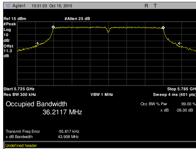
Plot 19. 26 dB Occupied Bandwidth, Low Channel, 802.11ac 40 MHz, Chain 0
