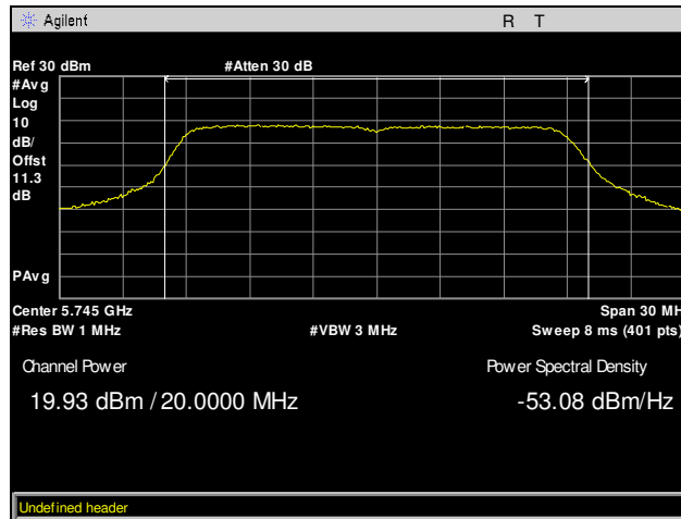
Plot 55. Maximum Conducted Output Power, Low Channel, 802.11ac 20 MHz, Chain 1
