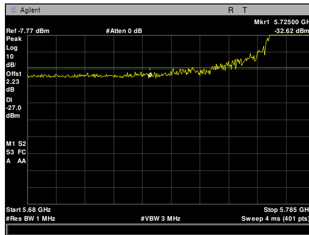
Plot 150. Radiated Band Edge, Mid Channel, 802.11a 20 MHz, 5725 Edge
