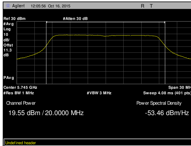
Plot 73. Maximum Conducted Output Power, Low Channel, 802.11n 20 MHz, Chain 1
