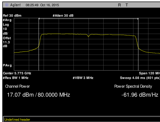
Plot 68. Maximum Conducted Output Power, Low Channel, 802.11ac 80 MHz, Chain 1
