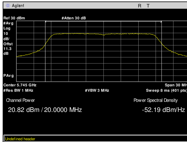
Plot 58. Maximum Conducted Output Power, Low Channel, 802.11ac 20 MHz, Chain 2
