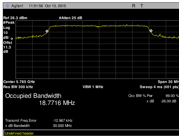
Plot 29. 26 dB Occupied Bandwidth, Mid Channel, 802.11n 20 MHz, Chain 0
