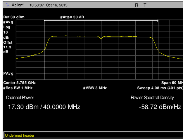
Plot 63. Maximum Conducted Output Power, Low Channel, 802.11ac 40 MHz, Chain 1
