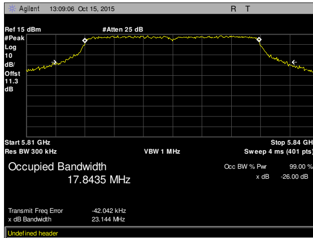
Plot 12. 26 dB Occupied Bandwidth, High Channel, 802.11ac 20 MHz, Chain 0
