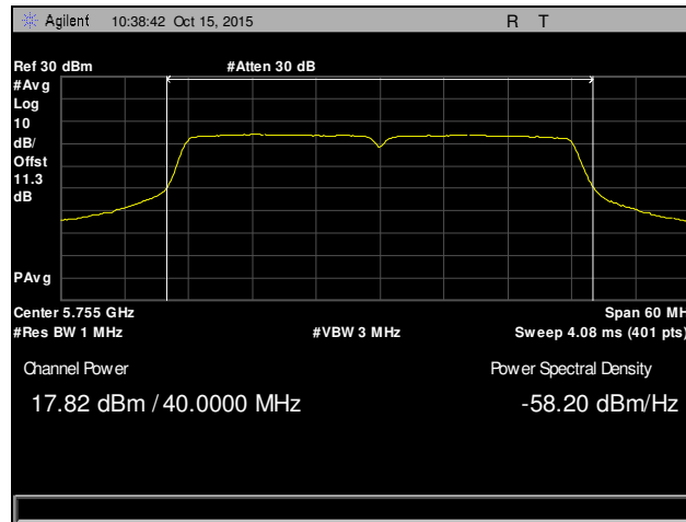
Plot 79. Maximum Conducted Output Power, Low Channel, 802.11n 40 MHz, Chain 0
