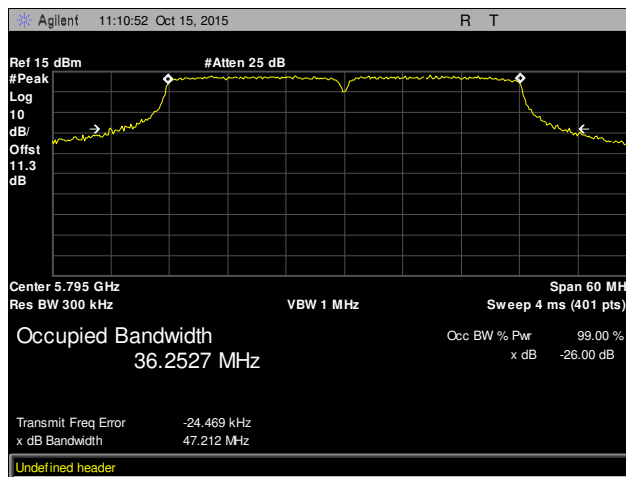
Plot 38. 26 dB Occupied Bandwidth, High Channel, 802.11n 40 MHz, Chain 0
