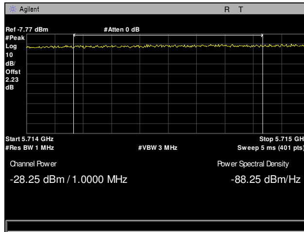
Plot 167. Radiated Band Edge, Low Channel, 802.11ac 40 MHz, 5715 Edge, Integration
