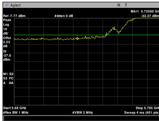
Plot 186. Radiated Band Edge, Mid Channel, 802.11n 20 MHz, 5725 Edge
