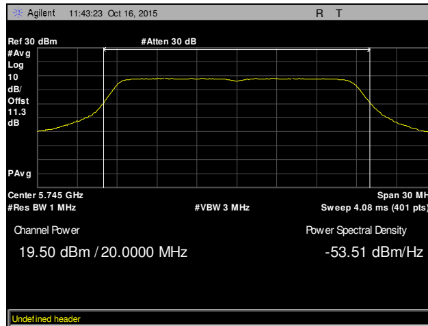
Plot 76. Maximum Conducted Output Power, Low Channel, 802.11n 20 MHz, Chain 2
