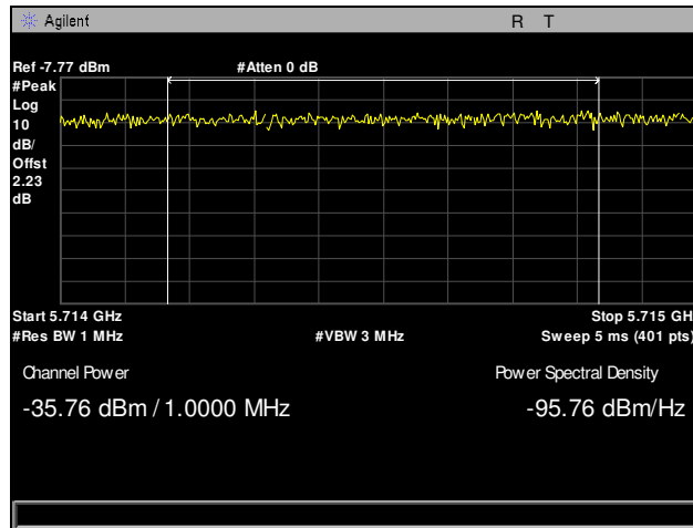
Plot 155. Radiated Band Edge, Low Channel, 802.11ac 20 MHz, 5715 Edge, Integration
