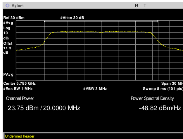
Plot 77. Maximum Conducted Output Power, Mid Channel, 802.11n 20 MHz, Chain 2
