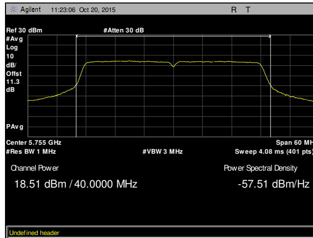
Plot 83. Maximum Conducted Output Power, Low Channel, 802.11n 40 MHz, Chain 2
