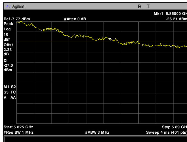
Plot 174. Radiated Band Edge, High Channel, 802.11ac 40 MHz, 5860 Edge
