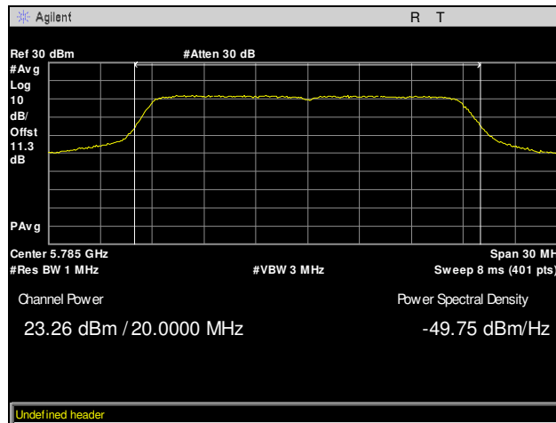
Plot 74. Maximum Conducted Output Power, Mid Channel, 802.11n 20 MHz, Chain 1
