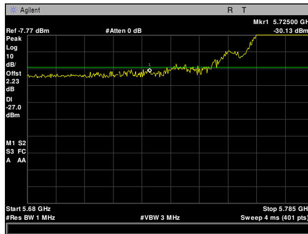
Plot 162. Radiated Band Edge, Mid Channel, 802.11ac 20 MHz, 5725 Edge
