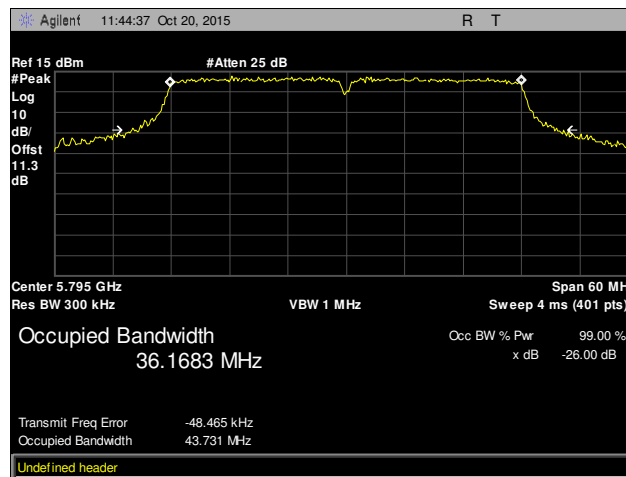
Plot 42. 26 dB Occupied Bandwidth, High Channel, 802.11n 40 MHz, Chain 2
