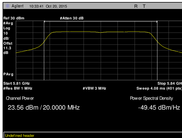
Plot 78. Maximum Conducted Output Power, High Channel, 802.11n 20 MHz, Chain 2
