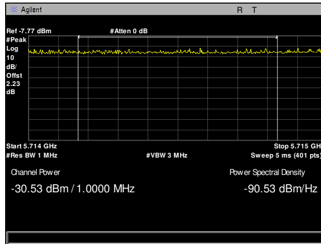
Plot 175. Radiated Band Edge, Low Channel, 802.11ac 80 MHz, 5715 Edge, Integration
