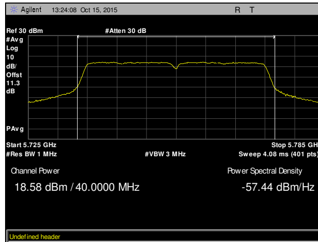
Plot 61. Maximum Conducted Output Power, Low Channel, 802.11ac 40 MHz, Chain 0
