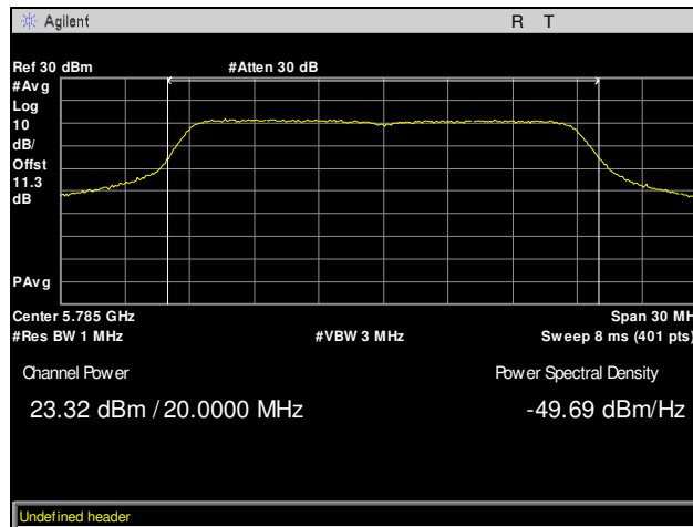
Plot 56. Maximum Conducted Output Power, Mid Channel, 802.11ac 20 MHz, Chain 1
