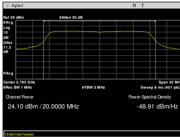
Plot 59. Maximum Conducted Output Power, Mid Channel, 802.11ac 20 MHz, Chain 2
