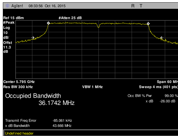
Plot 22. 26 dB Occupied Bandwidth, High Channel, 802.11ac 40 MHz, Chain 1
