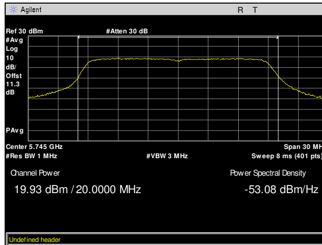
Plot 52. Maximum Conducted Output Power, Low Channel, 802.11ac 20 MHz, Chain 0
