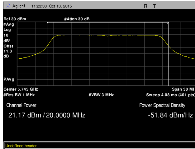
Plot 70. Maximum Conducted Output Power, Low Channel, 802.11n 20 MHz, Chain 0
