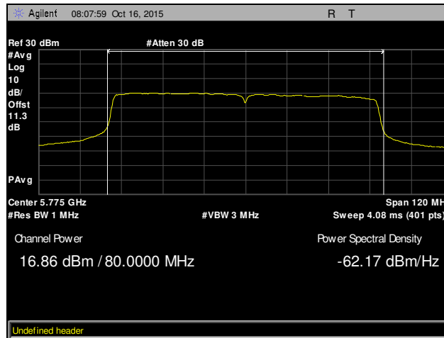
Plot 67. Maximum Conducted Output Power, Low Channel, 802.11ac 80 MHz, Chain 0
