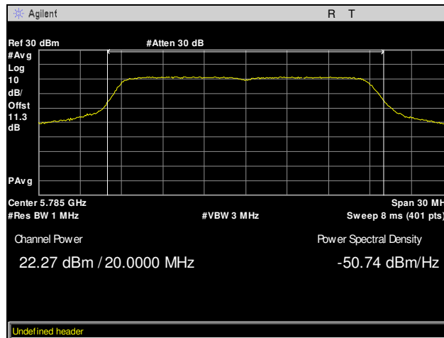
Plot 53. Maximum Conducted Output Power, Mid Channel, 802.11ac 20 MHz, Chain 0
