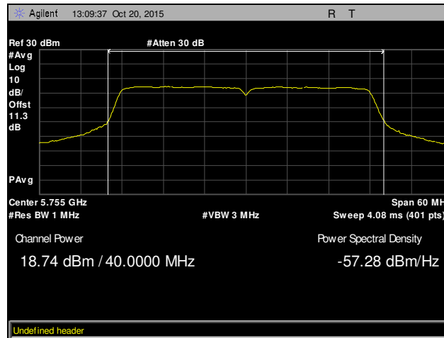
Plot 65. Maximum Conducted Output Power, Low Channel, 802.11ac 40 MHz, Chain 2
