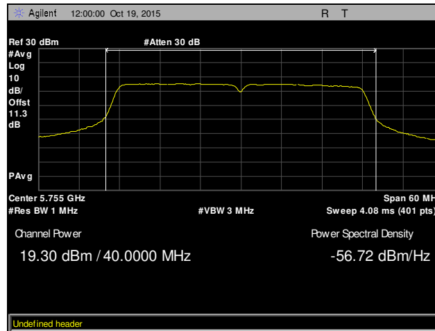
Plot 81. Maximum Conducted Output Power, Low Channel, 802.11n 40 MHz, Chain 1
