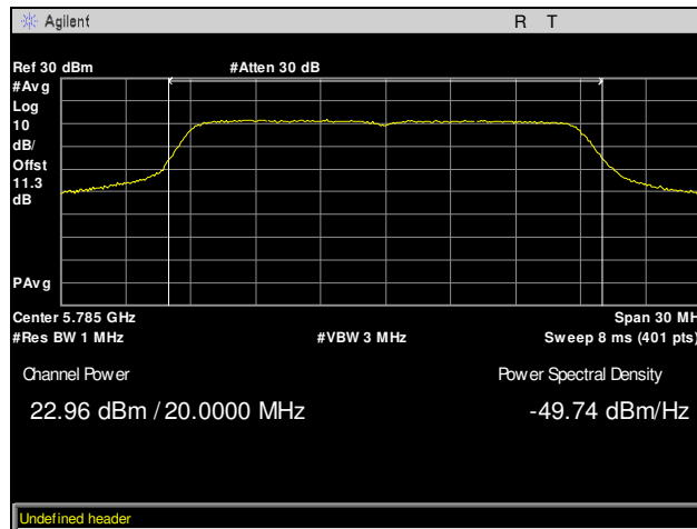
Plot 71. Maximum Conducted Output Power, Mid Channel, 802.11n 20 MHz, Chain 0
