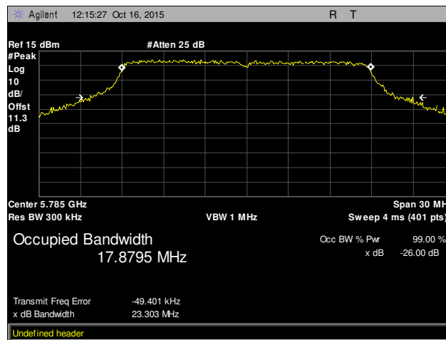
Plot 32. 26 dB Occupied Bandwidth, Mid Channel, 802.11n 20 MHz, Chain 1
