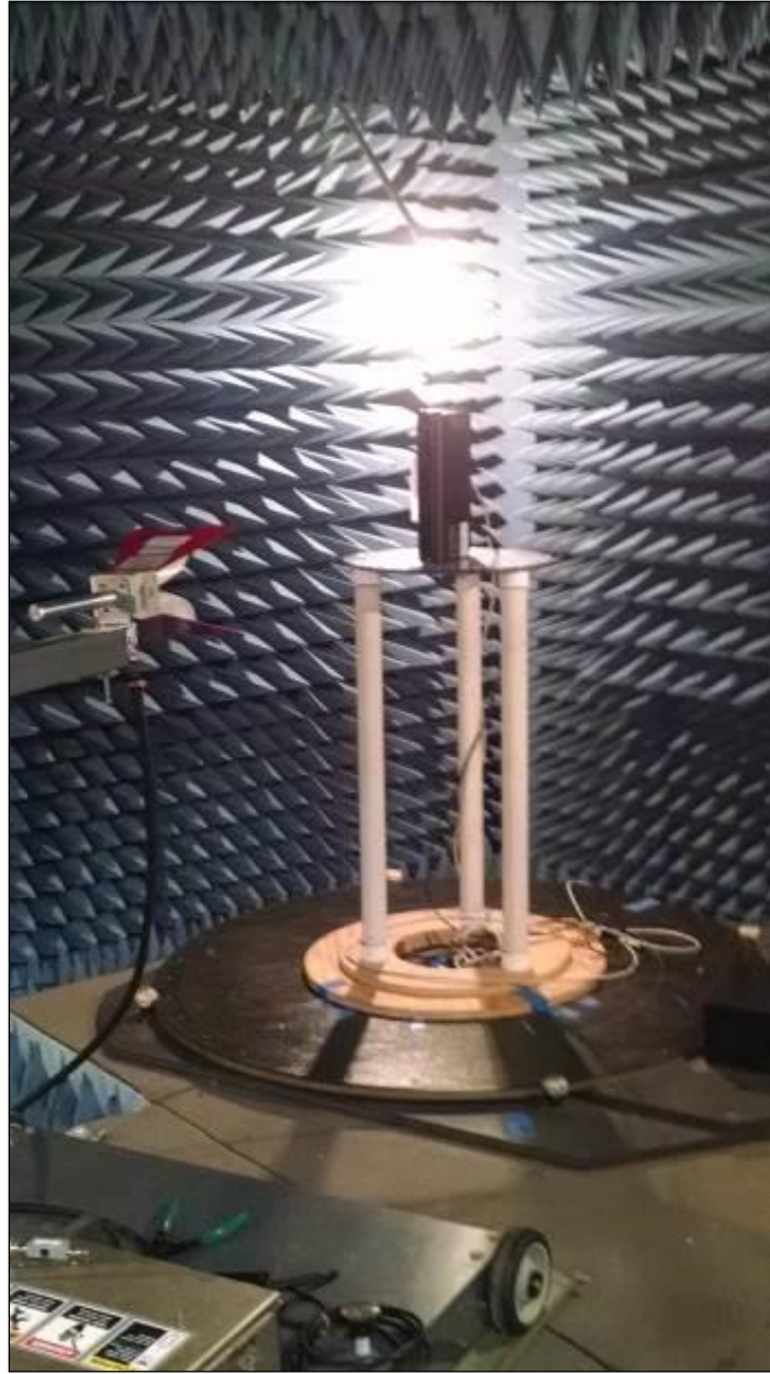
Photograph 2. Radiated Spurious Emissions, Test Setup, 1 GHz – 18 GHz
