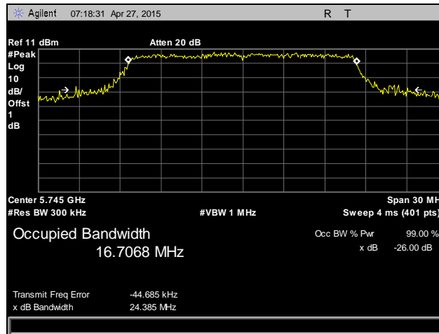
Plot 112. Occupied Bandwidth, 802.11a, Low Channel, 5745 MHz, Antenna 1
