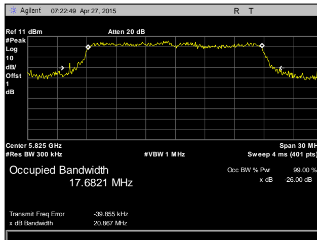
Plot 15. Occupied Bandwidth, 802.11n 20 MHz, High Channel, 5825 MHz, Antenna 1
