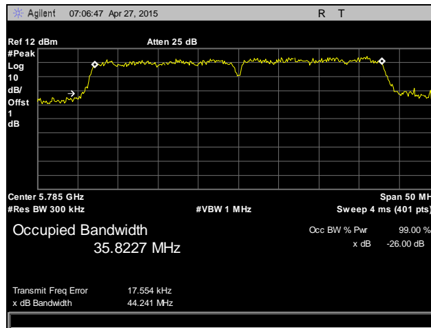
Plot 128. Occupied Bandwidth, 802.11n 40 MHz, Mid Channel, 5785 MHz, Antenna 0
