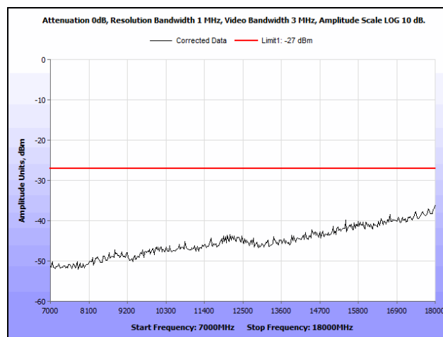
Plot 96. Radiated Spurious Emissions, 5785 MHz, 802.11n 20 MHz, 7 GHz – 18 GHz
