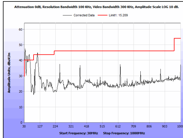
Plot 97. Radiated Spurious Emissions, 5825 MHz, 802.11n 20 MHz, 30 MHz – 1 GHz
