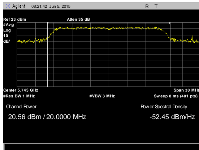
Plot 43. RF Output Power, 802.11n 20 MHz, Low Channel, 5745 MHz, Antenna 2
