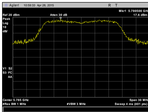
Plot 59. Peak Power Spectral Density, 802.11a, Mid Channel, 5785 MHz, Antenna 1
