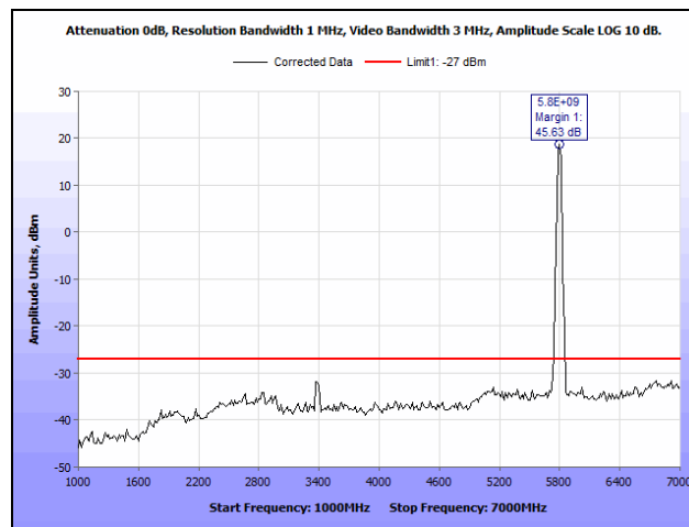
Plot 107. Radiated Spurious Emissions, 5795 MHz, 802.11n 40 MHz, 1 GHz – 7 GHz
