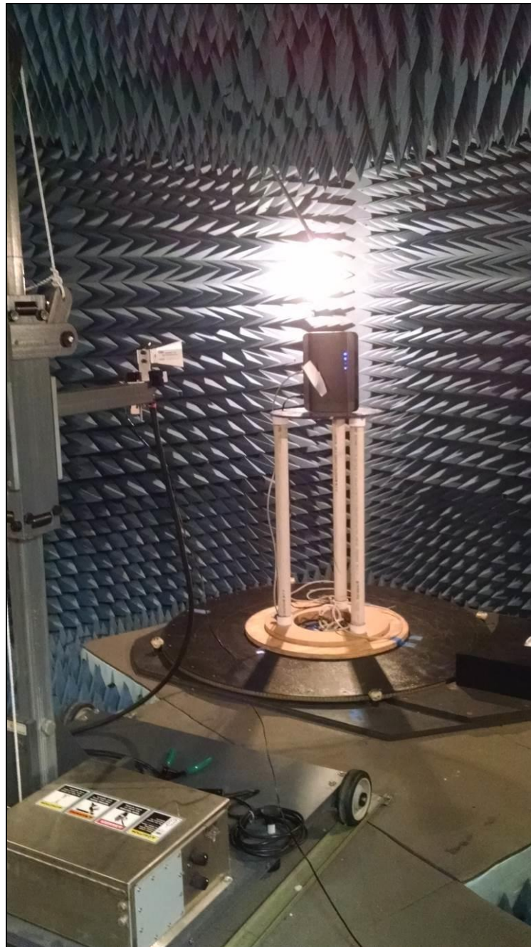
Photograph 3. Radiated Spurious Emissions, Test Setup, 18 GHz – 40 GHz
