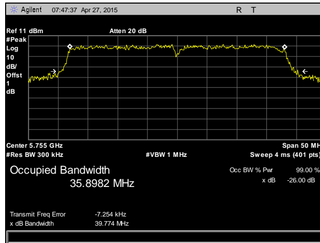
Plot 25. Occupied Bandwidth, 802.11n 40 MHz, Low Channel, 5755 MHz, Antenna 2
