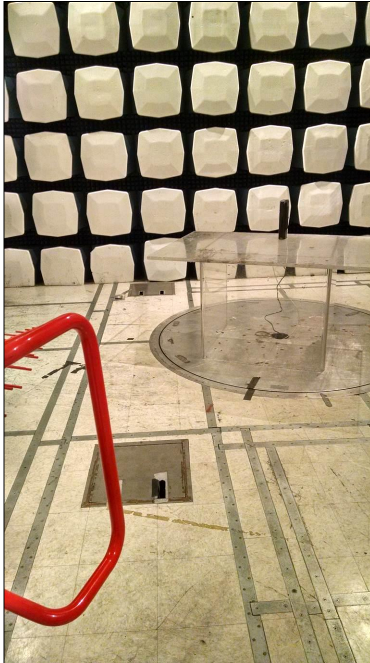
Photograph 1. Radiated Spurious Emissions, Test Setup, 30 MHz – 1 GHz
