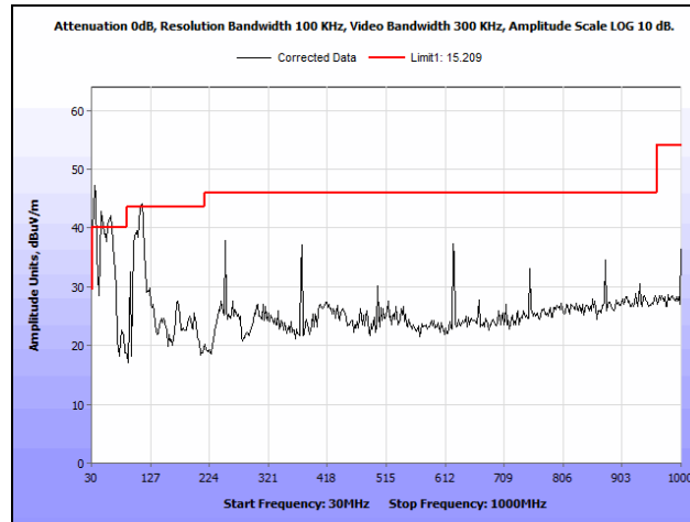
Plot 94. Radiated Spurious Emissions, 5785 MHz, 802.11n 20 MHz, 30 MHz – 1 GHz
