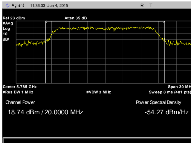
Plot 29. RF Output Power, 802.11a, Mid Channel, 5785 MHz, Antenna 0
