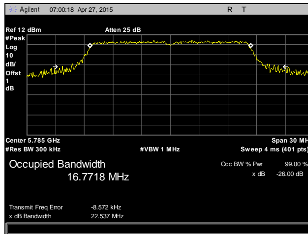
Plot 2. Occupied Bandwidth, 802.11a, Mid Channel, 5785 MHz, Antenna 0
