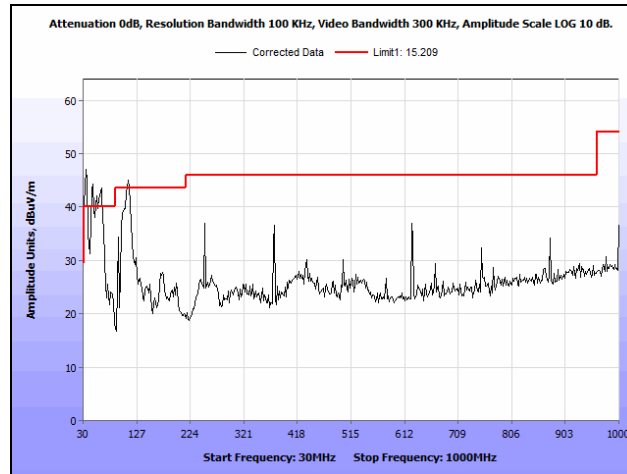
Plot 103. Radiated Spurious Emissions, 5785 MHz, 802.11n 40 MHz, 30 MHz – 1 GHz
