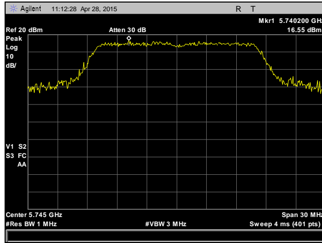
Plot 61. Peak Power Spectral Density, 802.11a, Low Channel, 5745 MHz, Antenna 2
