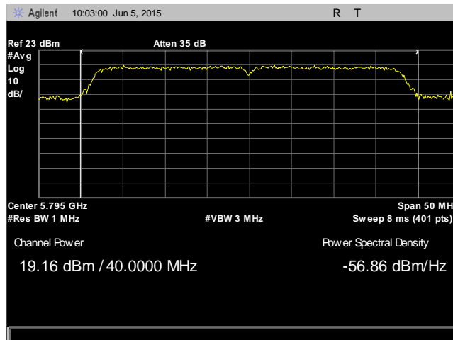
Plot 54. RF Output Power, 802.11n 40 MHz, High Channel, 5795 MHz, Antenna 2
