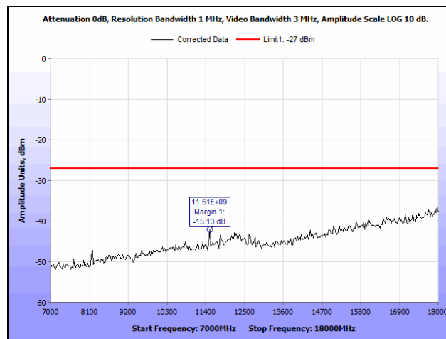
Plot 93. Radiated Spurious Emissions, 5745 MHz, 802.11n 20 MHz, 7 GHz – 18 GHz
