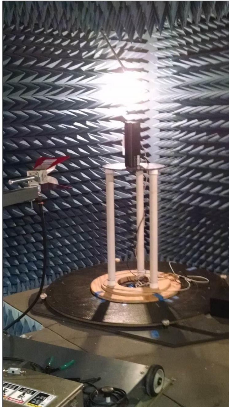
Photograph 2. Radiated Spurious Emissions, Test Setup, 1 GHz – 18 GHz
