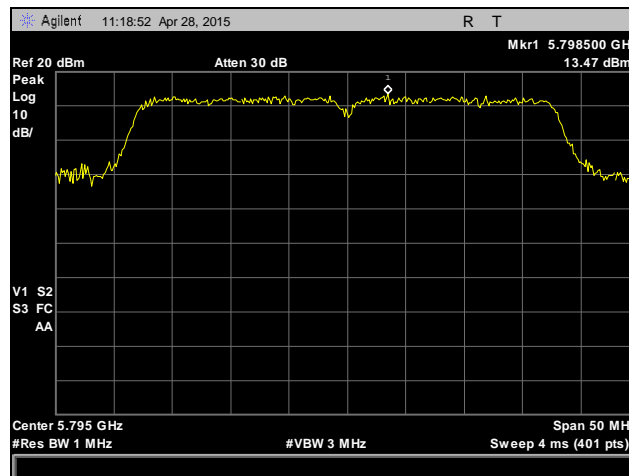
Plot 81. Peak Power Spectral Density, 802.11n 40 MHz, High Channel, 5795 MHz, Antenna 2
