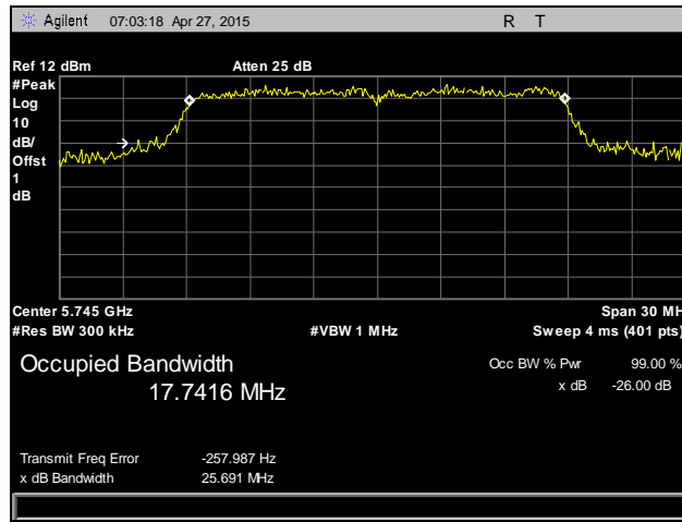
Plot 10. Occupied Bandwidth, 802.11n 20 MHz, Low Channel, 5745 MHz, Antenna 0
