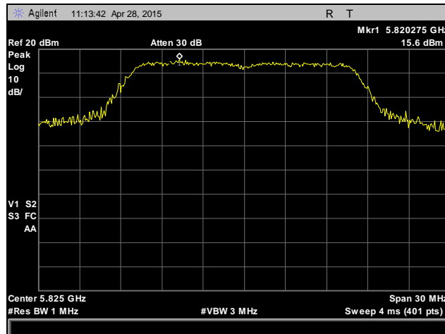
Plot 63. Peak Power Spectral Density, 802.11a, High Channel, 5825 MHz, Antenna 2
