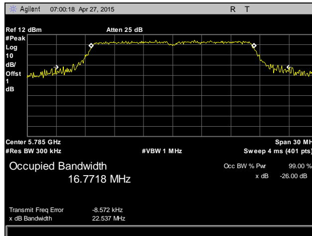
Plot 110. Occupied Bandwidth, 802.11a, Mid Channel, 5785 MHz, Antenna 0
