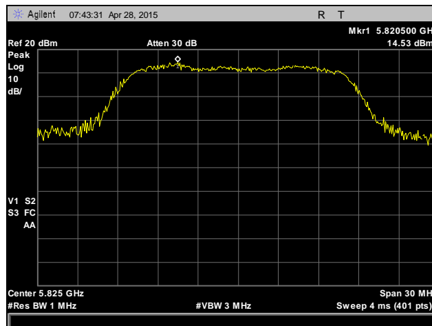
Plot 57. Peak Power Spectral Density, 802.11a, High Channel, 5825 MHz, Antenna 0
