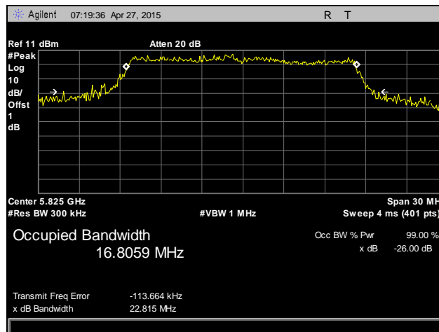
Plot 114. Occupied Bandwidth, 802.11a, High Channel, 5825 MHz, Antenna 1
