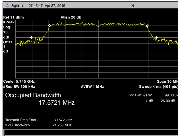
Plot 16. Occupied Bandwidth, 802.11n 20 MHz, Low Channel, 5745 MHz, Antenna 2
