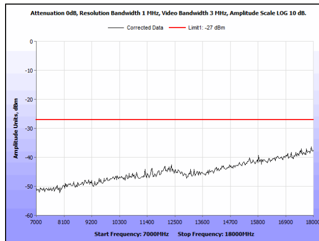
Plot 87. Radiated Spurious Emissions, 5785 MHz, 802.11a 20 MHz, 7 GHz – 18 GHz
