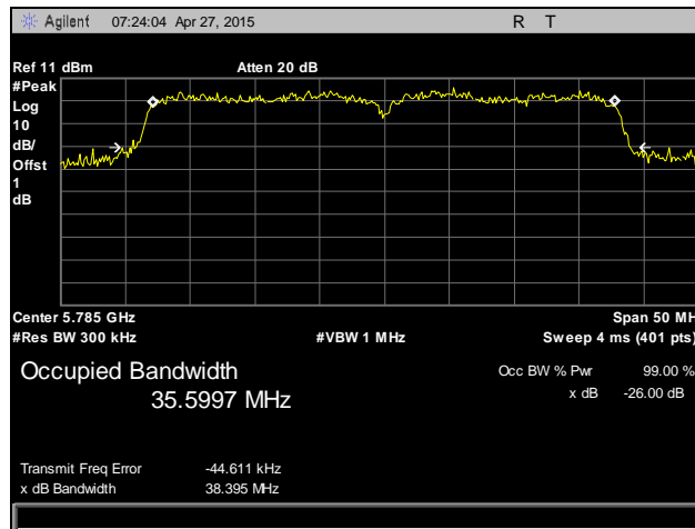
Plot 131. Occupied Bandwidth, 802.11n 40 MHz, Mid Channel, 5785 MHz, Antenna 1
