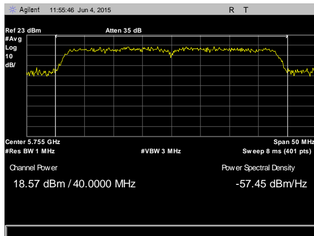
Plot 46. RF Output Power, 802.11n 40 MHz, Low Channel, 5755 MHz, Antenna 0
