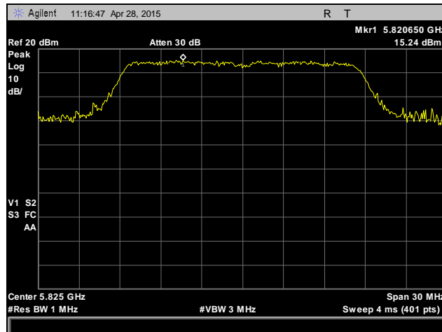
Plot 72. Peak Power Spectral Density, 802.11n 20 MHz, High Channel, 5825 MHz, Antenna 2
