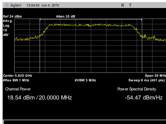
Plot 33. RF Output Power, 802.11a, High Channel, 5825 MHz, Antenna 1
