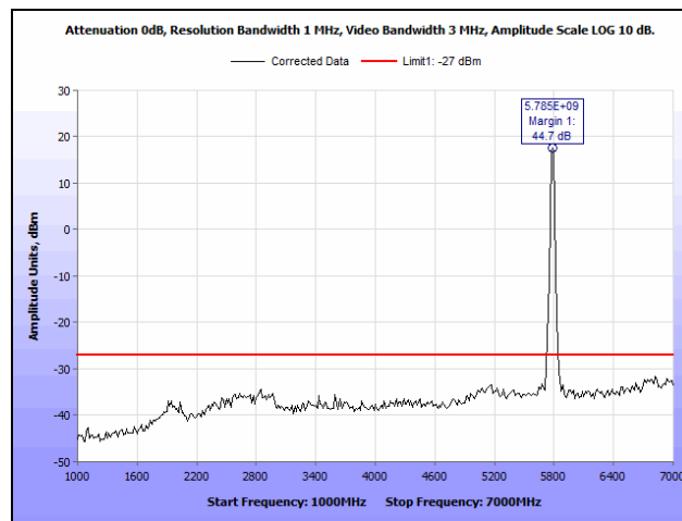
Plot 104. Radiated Spurious Emissions, 5785 MHz, 802.11n 40 MHz, 1 GHz – 7 GHz
