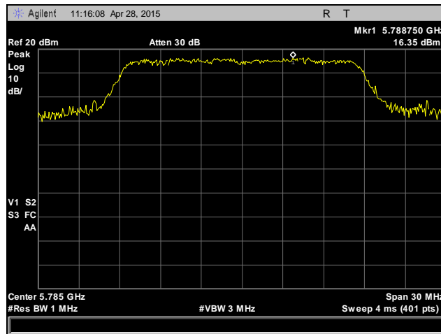
Plot 71. Peak Power Spectral Density, 802.11n 20 MHz, Mid Channel, 5785 MHz, Antenna 2
