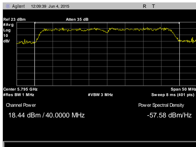
Plot 48. RF Output Power, 802.11n 40 MHz, High Channel, 5795 MHz, Antenna 0
