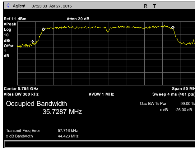
Plot 22. Occupied Bandwidth, 802.11n 40 MHz, Low Channel, 5755 MHz, Antenna 1
