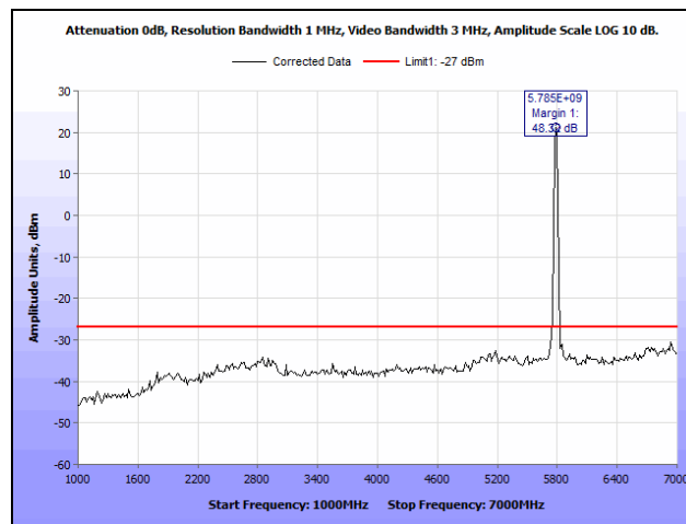
Plot 95. Radiated Spurious Emissions, 5785 MHz, 802.11n 20 MHz, 1 GHz – 7 GHz
