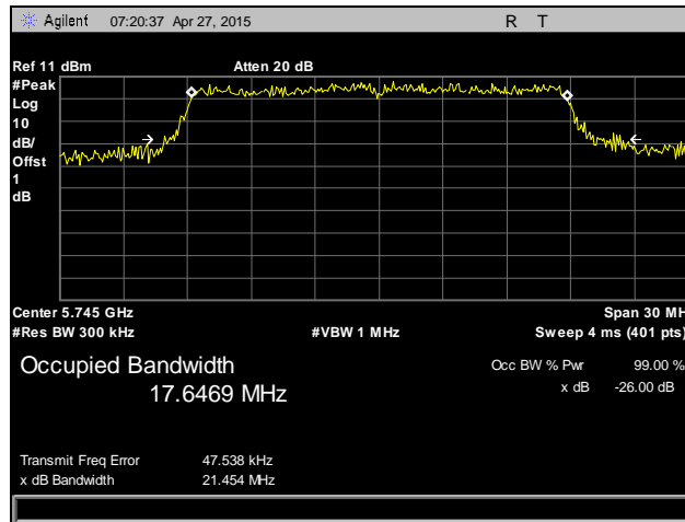
Plot 13. Occupied Bandwidth, 802.11n 20 MHz, Low Channel, 5745 MHz, Antenna 1
