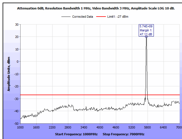
Plot 83. Radiated Spurious Emissions, 5745 MHz, 802.11a 20 MHz, 1 GHz – 7 GHz
