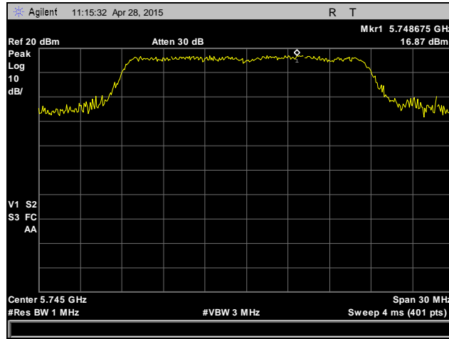
Plot 70. Peak Power Spectral Density, 802.11n 20 MHz, Low Channel, 5745 MHz, Antenna 2
