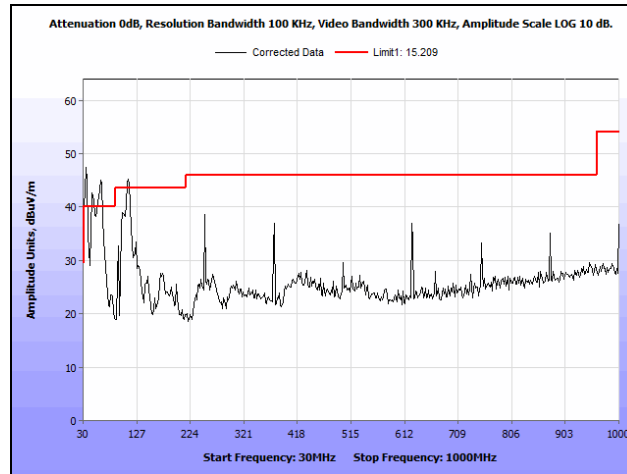
Plot 100. Radiated Spurious Emissions, 5755 MHz, 802.11n 40 MHz, 30 MHz – 1 GHz
