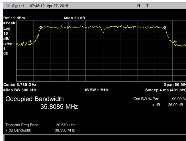
Plot 134. Occupied Bandwidth, 802.11n 40 MHz, Mid Channel, 5785 MHz, Antenna 2
