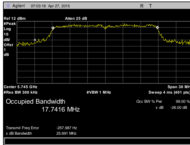
Plot 118. Occupied Bandwidth, 802.11n 20 MHz, Low Channel, 5745 MHz, Antenna 0
