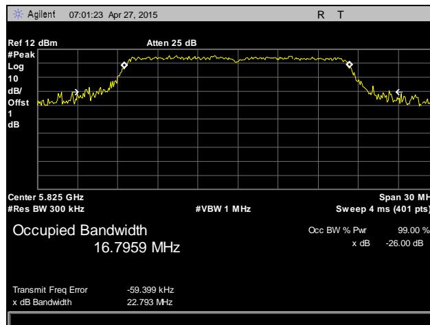
Plot 3. Occupied Bandwidth, 802.11a, High Channel, 5825 MHz, Antenna 0
