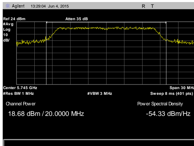
Plot 31. RF Output Power, 802.11a, Low Channel, 5745 MHz, Antenna 1
