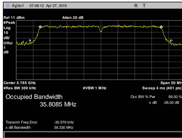
Plot 26. Occupied Bandwidth, 802.11n 40 MHz, Mid Channel, 5785 MHz, Antenna 2
