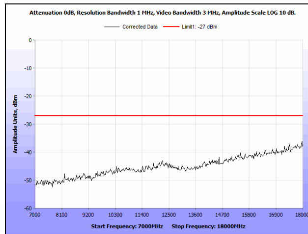
Plot 105. Radiated Spurious Emissions, 5785 MHz, 802.11n 40 MHz, 7 GHz – 18 GHz
