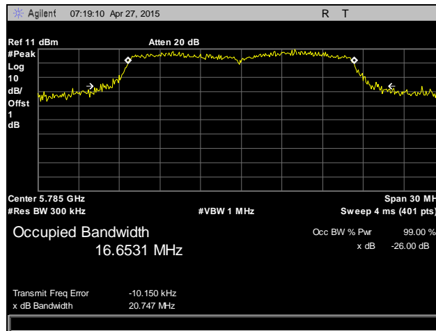
Plot 113. Occupied Bandwidth, 802.11a, Mid Channel, 5785 MHz, Antenna 1
