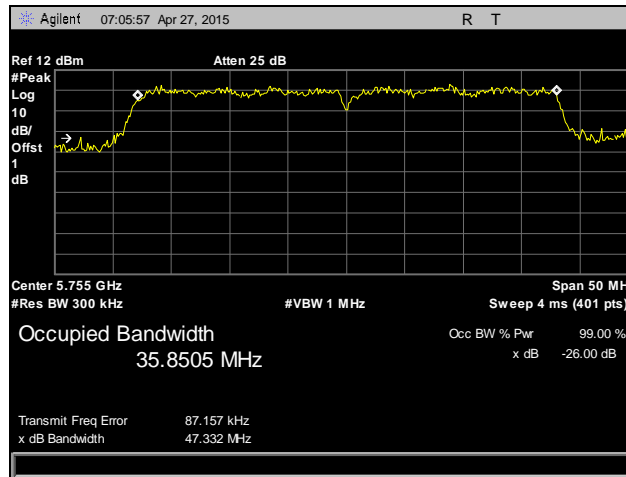
Plot 127. Occupied Bandwidth, 802.11n 40 MHz, Low Channel, 5755 MHz, Antenna 0
