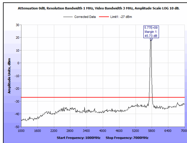
Plot 101. Radiated Spurious Emissions, 5755 MHz, 802.11n 40 MHz, 1 GHz – 7 GHz
