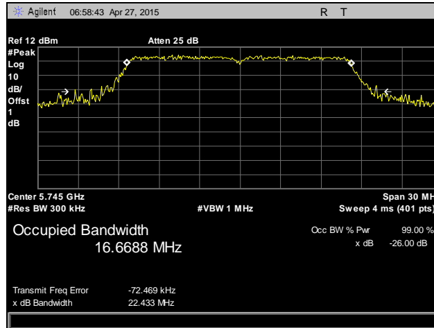
Plot 109. Occupied Bandwidth, 802.11a, Low Channel, 5745 MHz, Antenna 0
