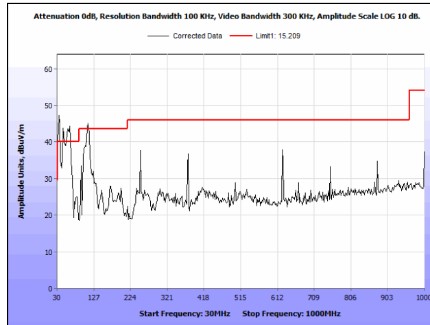
Plot 91. Radiated Spurious Emissions, 5745 MHz, 802.11n 20 MHz, 30 MHz – 1 GHz
