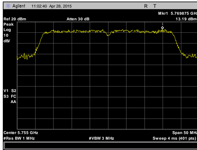
Plot 76. Peak Power Spectral Density, 802.11n 40 MHz, Low Channel, 5755 MHz, Antenna 1
