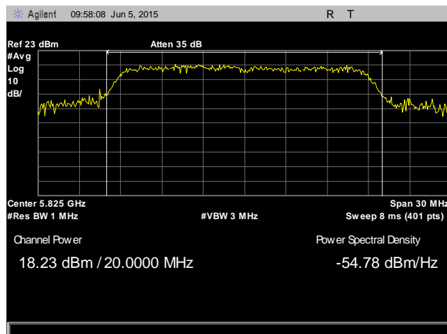
Plot 45. RF Output Power, 802.11n 20 MHz, High Channel, 5825 MHz, Antenna 2
