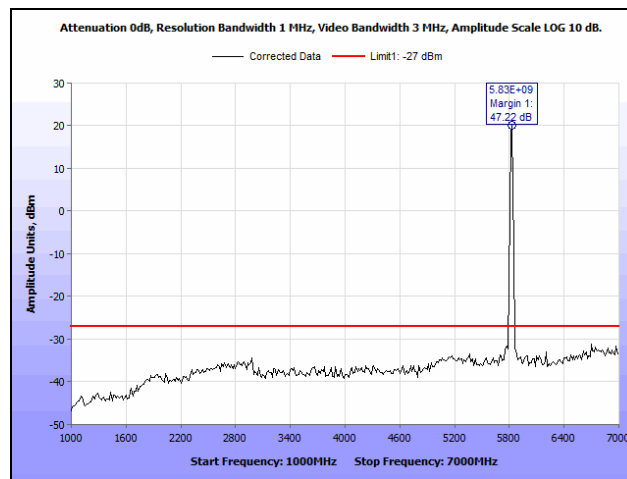
Plot 98. Radiated Spurious Emissions, 5825 MHz, 802.11n 20 MHz, 1 GHz – 7 GHz
