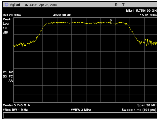
Plot 64. Peak Power Spectral Density, 802.11n 20 MHz, Low Channel, 5745 MHz, Antenna 0
