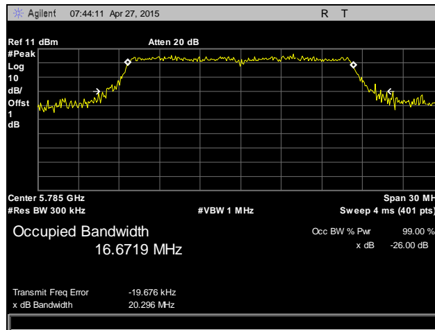
Plot 116. Occupied Bandwidth, 802.11a, Mid Channel, 5785 MHz, Antenna 2
