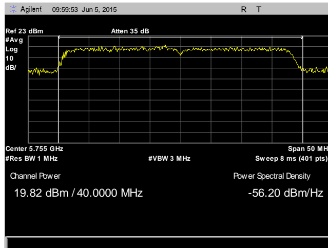
Plot 52. RF Output Power, 802.11n 40 MHz, Low Channel, 5755 MHz, Antenna 2
