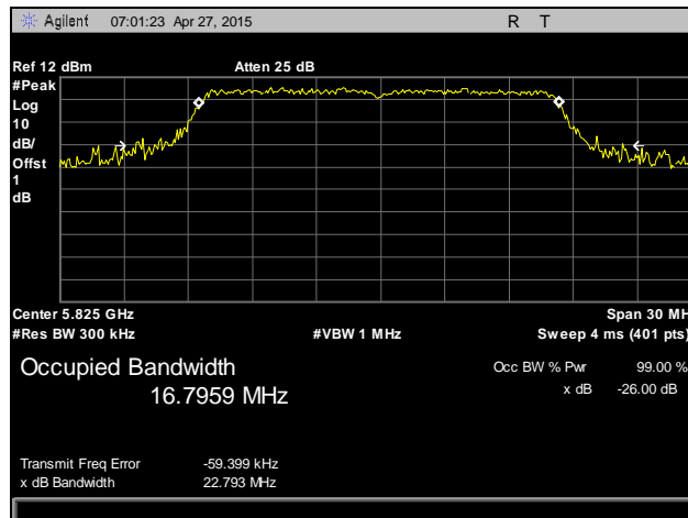
Plot 111. Occupied Bandwidth, 802.11a, High Channel, 5825 MHz, Antenna 0
