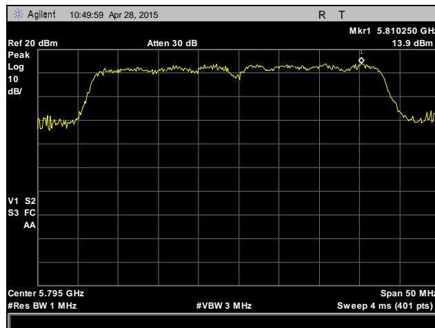
Plot 75. Peak Power Spectral Density, 802.11n 40 MHz, High Channel, 5795 MHz, Antenna 0
