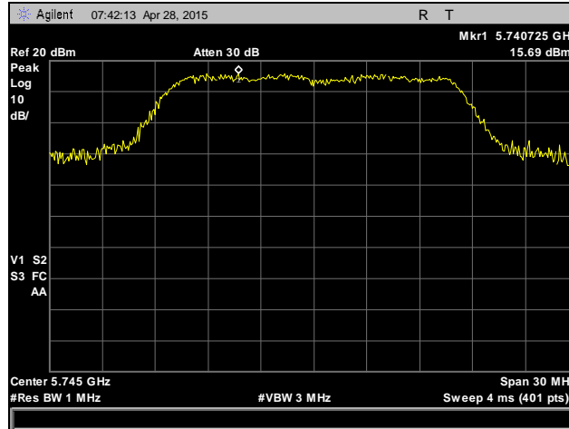
Plot 55. Peak Power Spectral Density, 802.11a, Low Channel, 5745 MHz, Antenna 0
