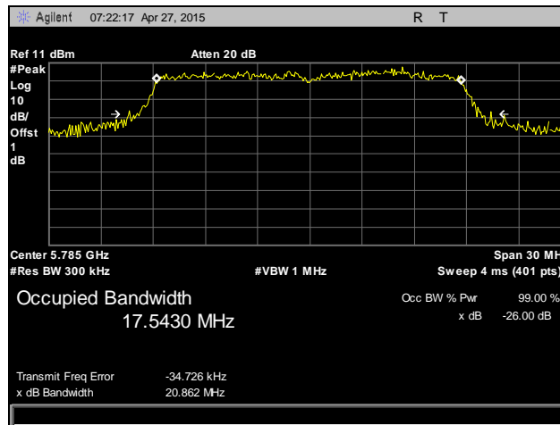
Plot 14. Occupied Bandwidth, 802.11n 20 MHz, Mid Channel, 5785 MHz, Antenna 1
