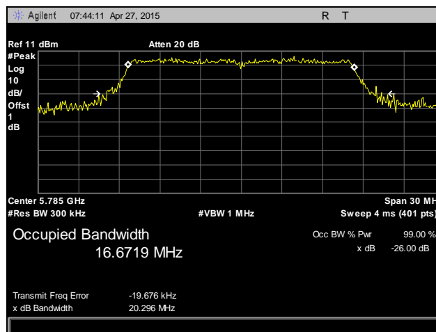
Plot 8. Occupied Bandwidth, 802.11a, Mid Channel, 5785 MHz, Antenna 2
