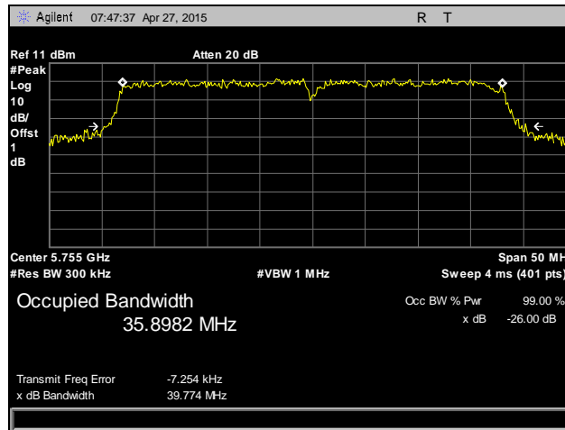
Plot 133. Occupied Bandwidth, 802.11n 40 MHz, Low Channel, 5755 MHz, Antenna 2
