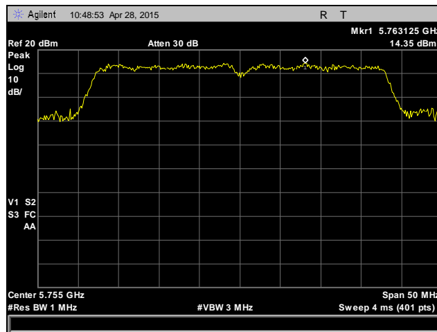
Plot 73. Peak Power Spectral Density, 802.11n 40 MHz, Low Channel, 5755 MHz, Antenna 0
