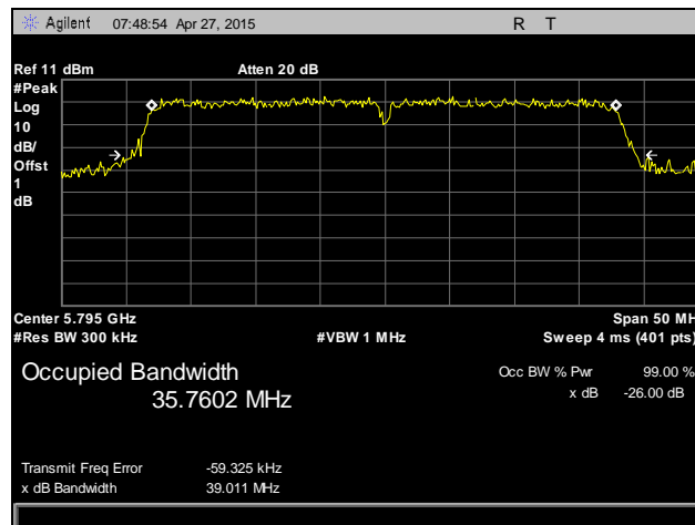
Plot 27. Occupied Bandwidth, 802.11n 40 MHz, High Channel, 5795 MHz, Antenna 2
