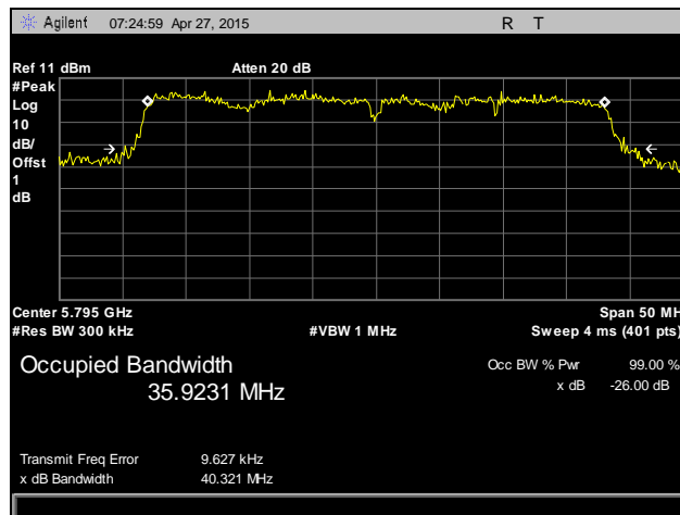
Plot 132. Occupied Bandwidth, 802.11n 40 MHz, High Channel, 5795 MHz, Antenna 1
