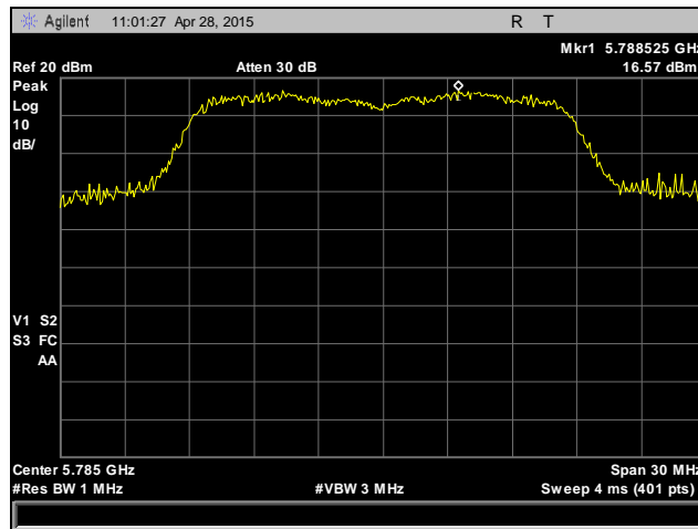
Plot 68. Peak Power Spectral Density, 802.11n 20 MHz, Mid Channel, 5785 MHz, Antenna 1
