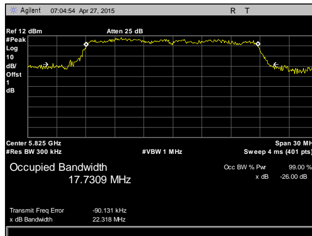
Plot 120. Occupied Bandwidth, 802.11n 20 MHz, High Channel, 5825 MHz, Antenna 0
