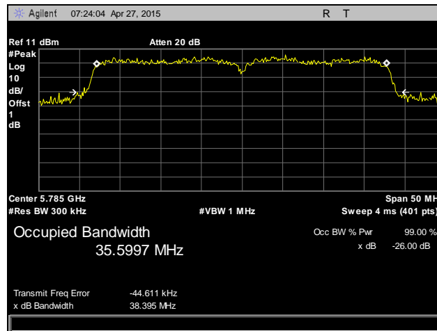
Plot 23. Occupied Bandwidth, 802.11n 40 MHz, Mid Channel, 5785 MHz, Antenna 1
