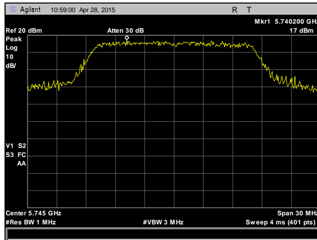
Plot 58. Peak Power Spectral Density, 802.11a, Low Channel, 5745 MHz, Antenna 1
