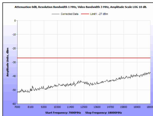
Plot 90. Radiated Spurious Emissions, 5825 MHz, 802.11a 20 MHz, 7 GHz – 18 GHz
