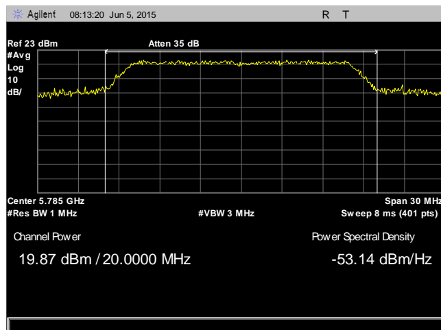
Plot 35. RF Output Power, 802.11a, Mid Channel, 5785 MHz, Antenna 2
