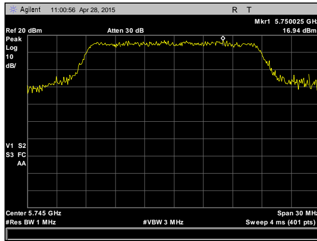
Plot 67. Peak Power Spectral Density, 802.11n 20 MHz, Low Channel, 5745 MHz, Antenna 1
