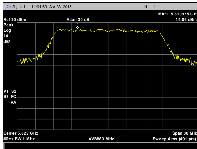
Plot 69. Peak Power Spectral Density, 802.11n 20 MHz, High Channel, 5825 MHz, Antenna 1
