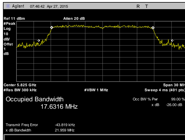
Plot 126. Occupied Bandwidth, 802.11n 20 MHz, High Channel, 5825 MHz, Antenna 2
