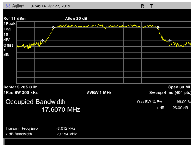
Plot 17. Occupied Bandwidth, 802.11n 20 MHz, Mid Channel, 5785 MHz, Antenna 2
