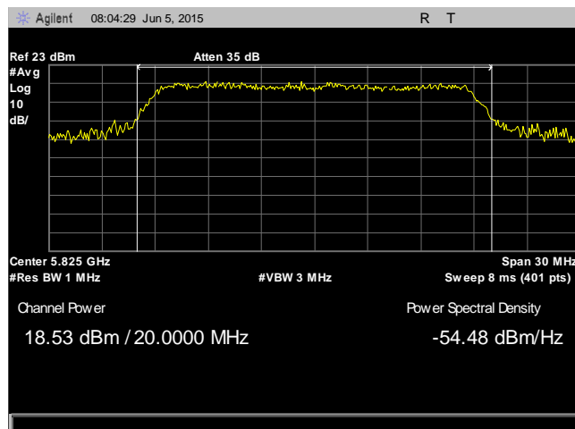
Plot 42. RF Output Power, 802.11n 20 MHz, High Channel, 5825 MHz, Antenna 1
