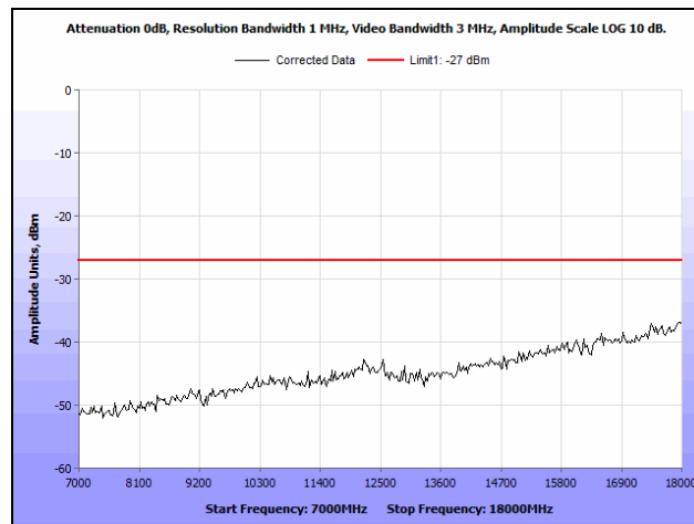
Plot 99. Radiated Spurious Emissions, 5825 MHz, 802.11n 20 MHz, 7 GHz – 18 GHz
