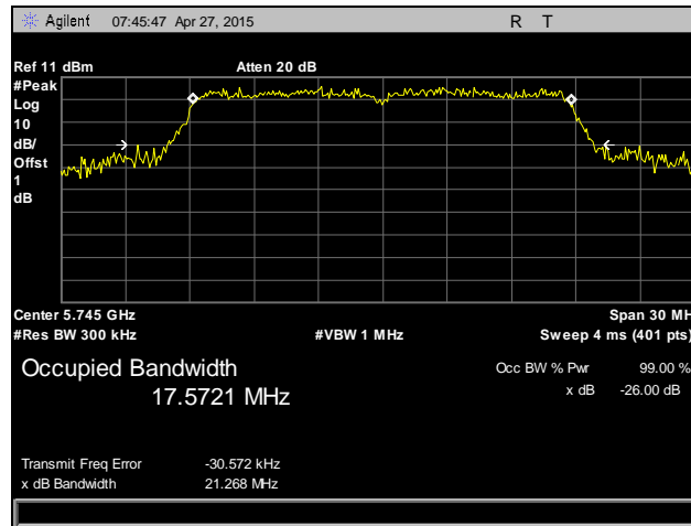
Plot 124. Occupied Bandwidth, 802.11n 20 MHz, Low Channel, 5745 MHz, Antenna 2
