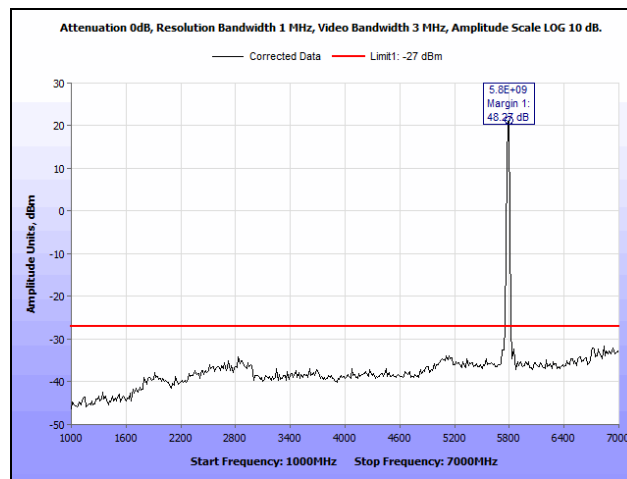
Plot 86. Radiated Spurious Emissions, 5785 MHz, 802.11a 20 MHz, 1 GHz – 7 GHz
