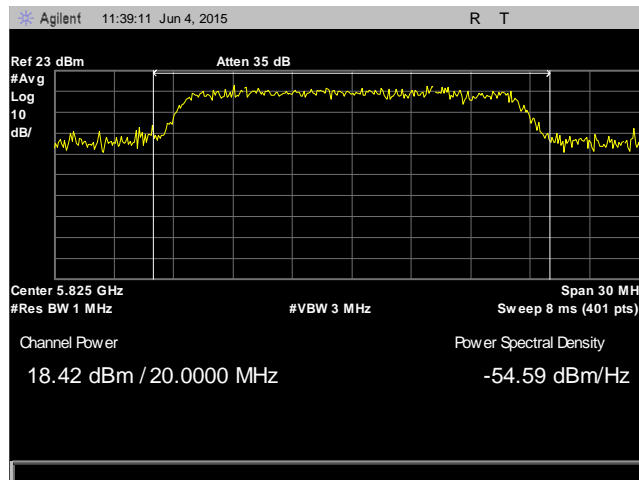
Plot 30. RF Output Power, 802.11a, High Channel, 5825 MHz, Antenna 0
