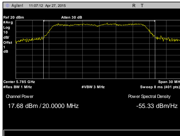
Plot 56. Peak Power Spectral Density, 802.11a, Mid Channel, 5785 MHz, Antenna 0
