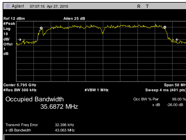
Plot 21. Occupied Bandwidth, 802.11n 40 MHz, High Channel, 5795 MHz, Antenna 0
