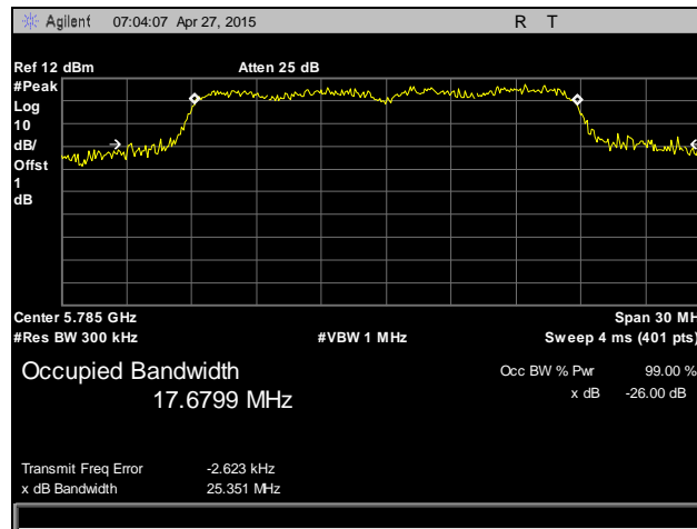
Plot 119. Occupied Bandwidth, 802.11n 20 MHz, Mid Channel, 5785 MHz, Antenna 0
