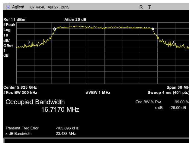
Plot 9. Occupied Bandwidth, 802.11a, High Channel, 5825 MHz, Antenna 2
