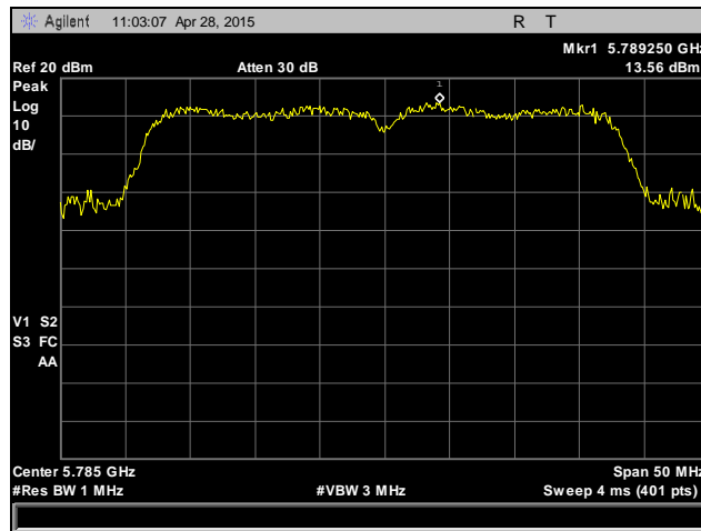
Plot 77. Peak Power Spectral Density, 802.11n 40 MHz, Mid Channel, 5785 MHz, Antenna 1
