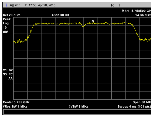
Plot 79. Peak Power Spectral Density, 802.11n 40 MHz, Low Channel, 5755 MHz, Antenna 2
