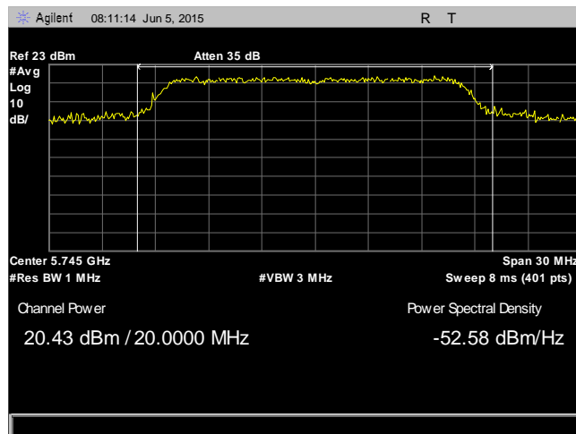
Plot 34. RF Output Power, 802.11a, Low Channel, 5745 MHz, Antenna 2
