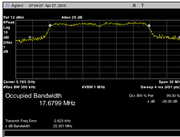
Plot 11. Occupied Bandwidth, 802.11n 20 MHz, Mid Channel, 5785 MHz, Antenna 0
