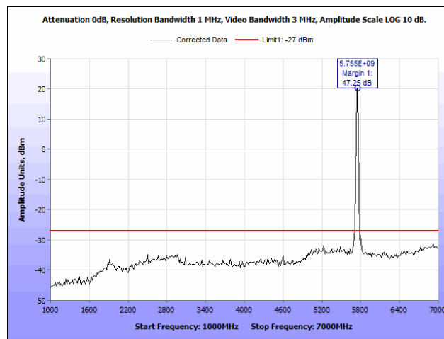
Plot 92. Radiated Spurious Emissions, 5745 MHz, 802.11n 20 MHz, 1 GHz – 7 GHz
