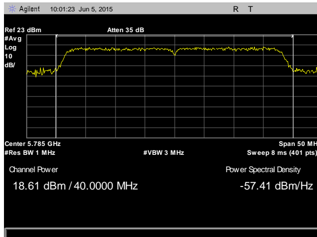
Plot 53. RF Output Power, 802.11n 40 MHz, Mid Channel, 5785 MHz, Antenna 2
