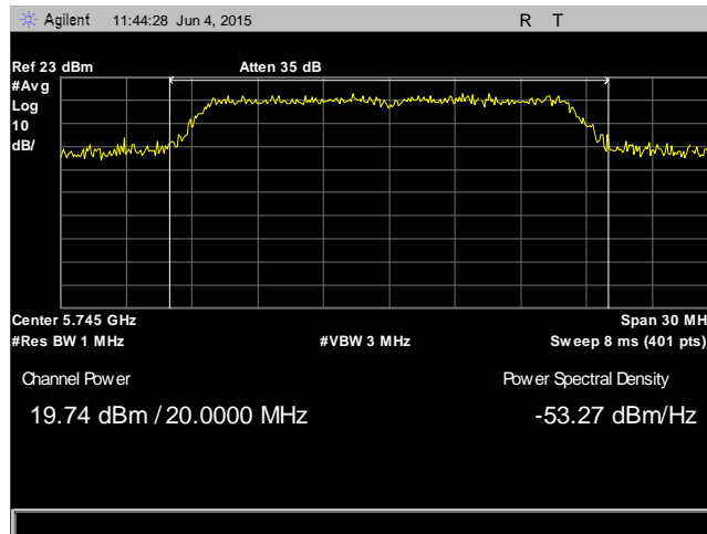
Plot 28. RF Output Power, 802.11a, Low Channel, 5745 MHz, Antenna 0
