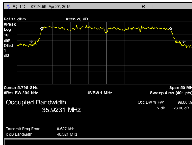
Plot 24. Occupied Bandwidth, 802.11n 40 MHz, High Channel, 5795 MHz, Antenna 1
