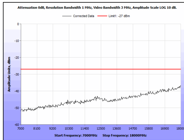
Plot 108. Radiated Spurious Emissions, 5795 MHz, 802.11n 40 MHz, 7 GHz – 18 GHz
