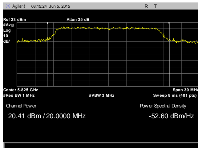
Plot 36. RF Output Power, 802.11a, High Channel, 5825 MHz, Antenna 2
