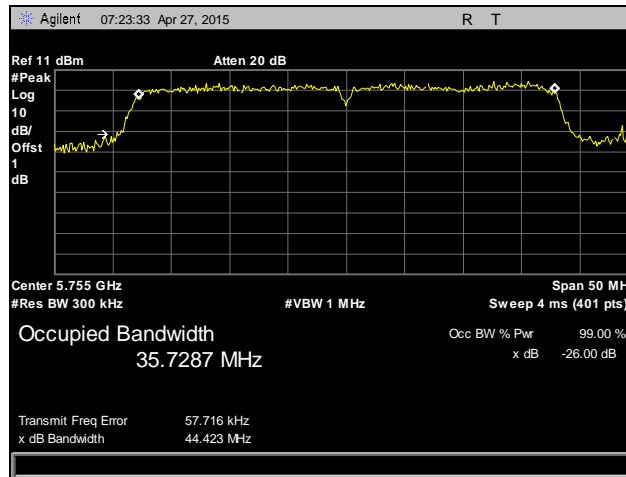
Plot 130. Occupied Bandwidth, 802.11n 40 MHz, Low Channel, 5755 MHz, Antenna 1
