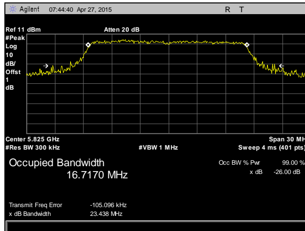
Plot 117. Occupied Bandwidth, 802.11a, High Channel, 5825 MHz, Antenna 2
