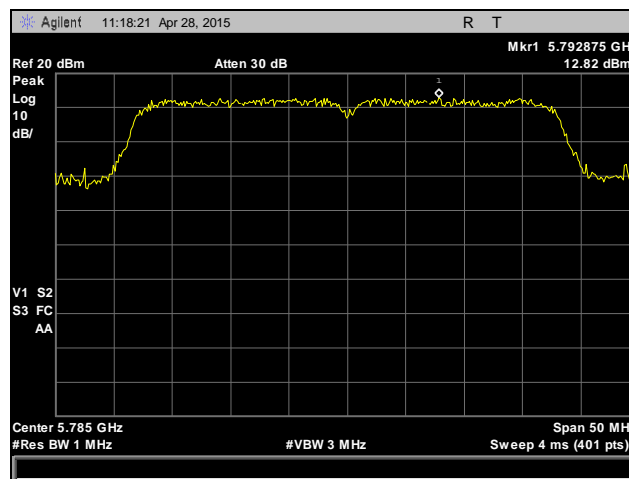
Plot 80. Peak Power Spectral Density, 802.11n 40 MHz, Mid Channel, 5785 MHz, Antenna 2
