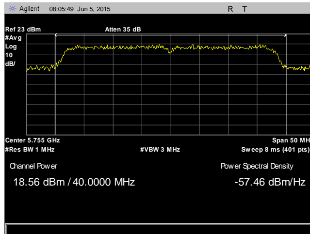
Plot 49. RF Output Power, 802.11n 40 MHz, Low Channel, 5755 MHz, Antenna 1
