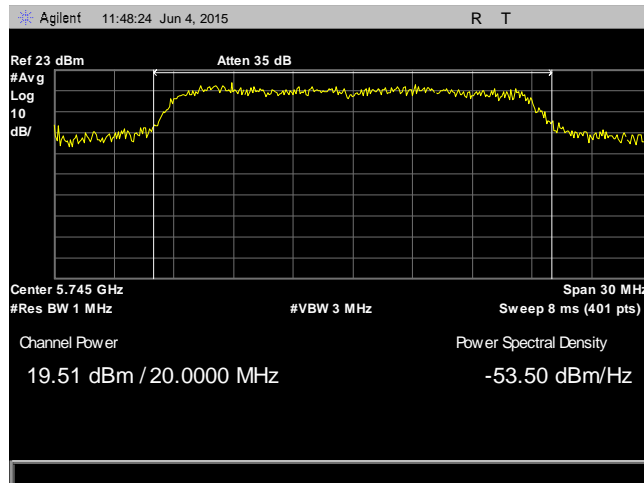
Plot 37. RF Output Power, 802.11n 20 MHz, Low Channel, 5745 MHz, Antenna 0
