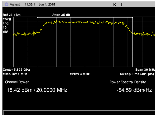
Plot 39. RF Output Power, 802.11n 20 MHz, High Channel, 5825 MHz, Antenna 0
