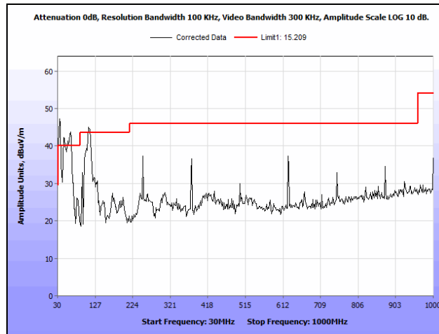
Plot 82. Radiated Spurious Emissions, 5745 MHz, 802.11a 20 MHz, 30 MHz – 1 GHz
