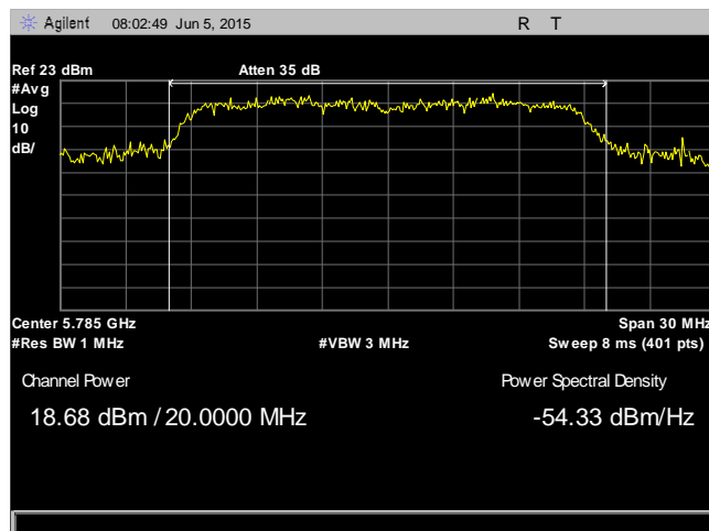
Plot 41. RF Output Power, 802.11n 20 MHz, Mid Channel, 5785 MHz, Antenna 1
