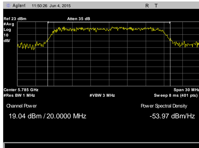
Plot 38. RF Output Power, 802.11n 20 MHz, Mid Channel, 5785 MHz, Antenna 0
