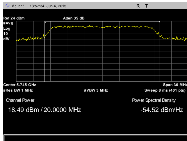
Plot 40. RF Output Power, 802.11n 20 MHz, Low Channel, 5745 MHz, Antenna 1
