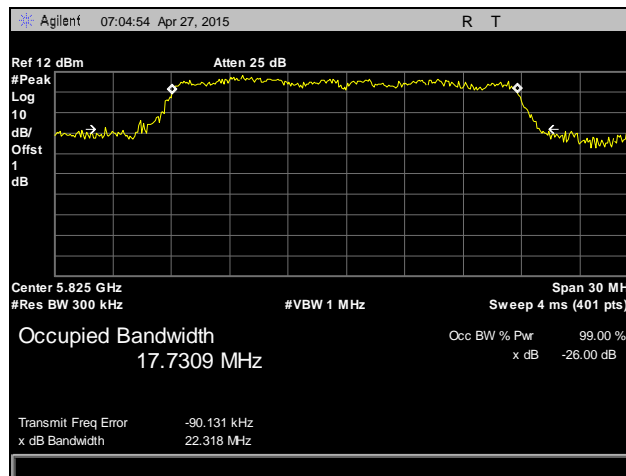
Plot 12. Occupied Bandwidth, 802.11n 20 MHz, High Channel, 5825 MHz, Antenna 0
