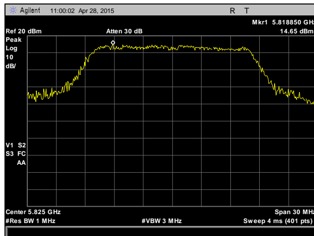
Plot 60. Peak Power Spectral Density, 802.11a, High Channel, 5825 MHz, Antenna 1
