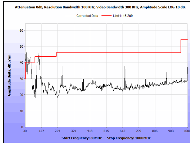
Plot 106. Radiated Spurious Emissions, 5795 MHz, 802.11n 40 MHz, 30 MHz – 1 GHz
