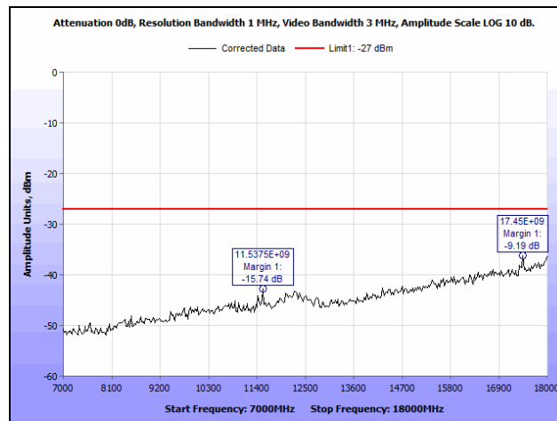
Plot 102. Radiated Spurious Emissions, 5755 MHz, 802.11n 40 MHz, 7 GHz – 18 GHz
