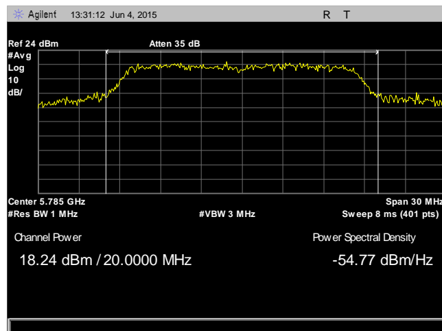
Plot 32. RF Output Power, 802.11a, Mid Channel, 5785 MHz, Antenna 1
