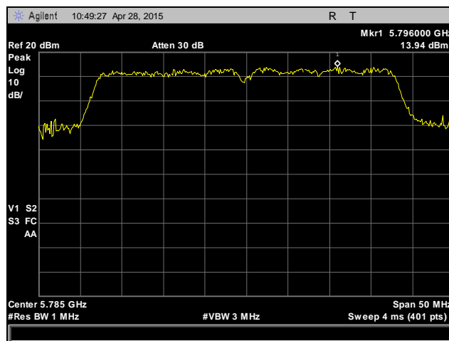
Plot 74. Peak Power Spectral Density, 802.11n 40 MHz, Mid Channel, 5785 MHz, Antenna 0
