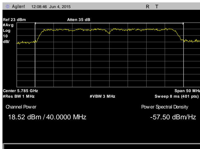
Plot 47. RF Output Power, 802.11n 40 MHz, Mid Channel, 5785 MHz, Antenna 0
