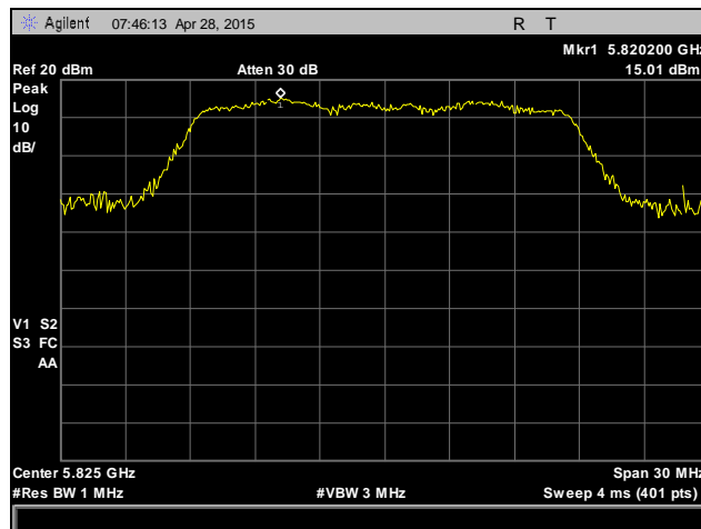
Plot 66. Peak Power Spectral Density, 802.11n 20 MHz, High Channel, 5825 MHz, Antenna 0
