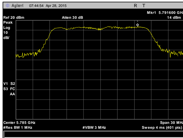
Plot 65. Peak Power Spectral Density, 802.11n 20 MHz, Mid Channel, 5785 MHz, Antenna 0
