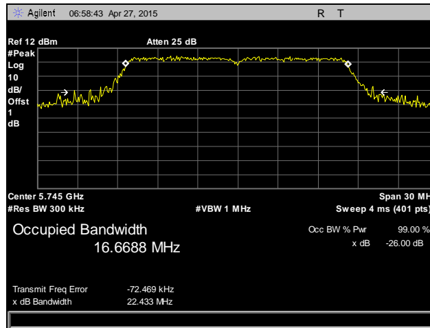
Plot 1. Occupied Bandwidth, 802.11a, Low Channel, 5745 MHz, Antenna 0
