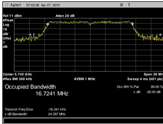
Plot 115. Occupied Bandwidth, 802.11a, Low Channel, 5745 MHz, Antenna 2
