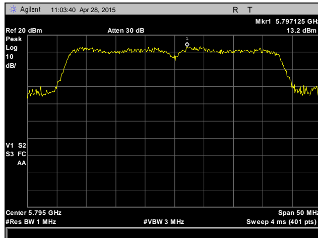
Plot 78. Peak Power Spectral Density, 802.11n 40 MHz, High Channel, 5795 MHz, Antenna 1
