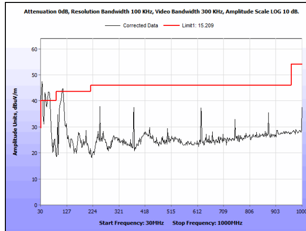
Plot 85. Radiated Spurious Emissions, 5785 MHz, 802.11a 20 MHz, 30 MHz – 1 GHz
