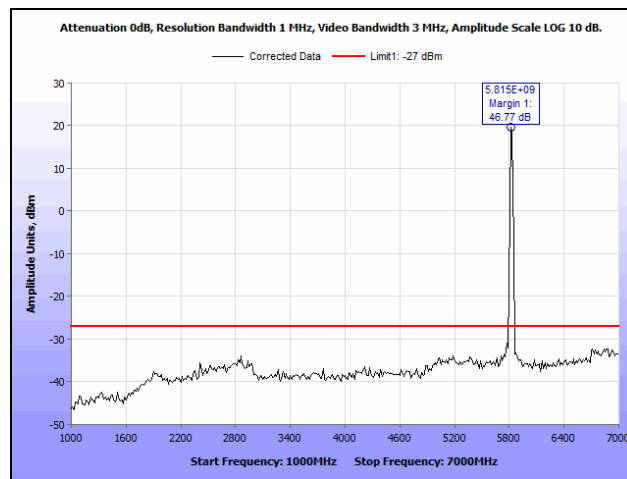
Plot 89. Radiated Spurious Emissions, 5825 MHz, 802.11a 20 MHz, 1 GHz – 7 GHz
