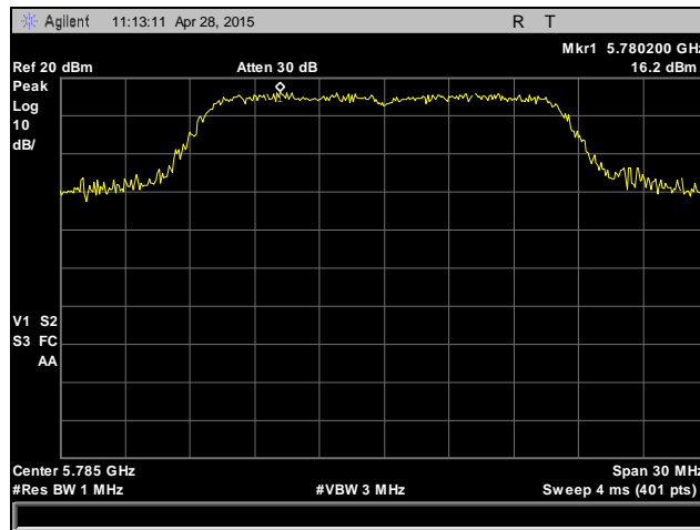
Plot 62. Peak Power Spectral Density, 802.11a, Mid Channel, 5785 MHz, Antenna 2
