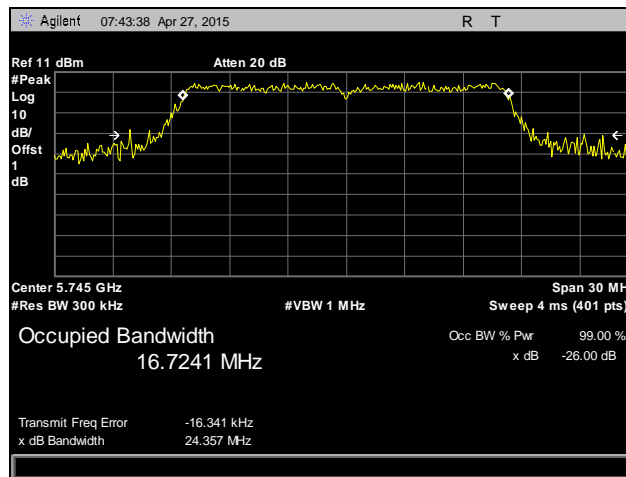
Plot 7. Occupied Bandwidth, 802.11a, Low Channel, 5745 MHz, Antenna 2
