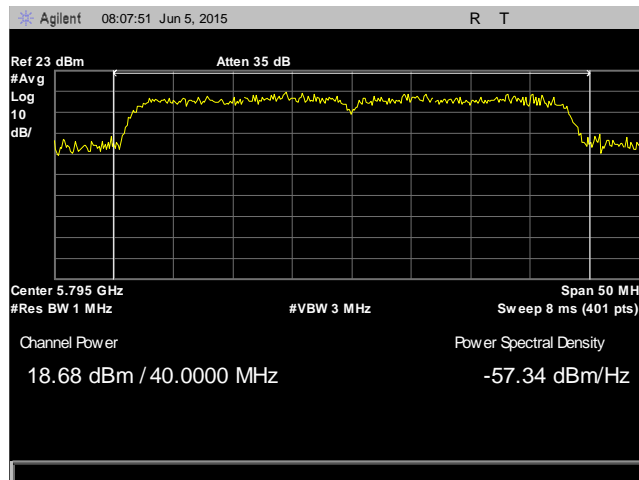
Plot 51. RF Output Power, 802.11n 40 MHz, High Channel, 5795 MHz, Antenna 1
