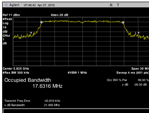
Plot 18. Occupied Bandwidth, 802.11n 20 MHz, High Channel, 5825 MHz, Antenna 2
