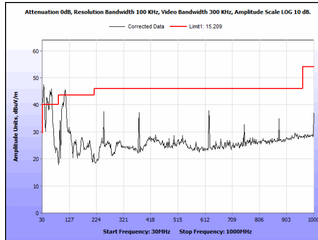
Plot 88. Radiated Spurious Emissions, 5825 MHz, 802.11a 20 MHz, 30 MHz – 1 GHz
