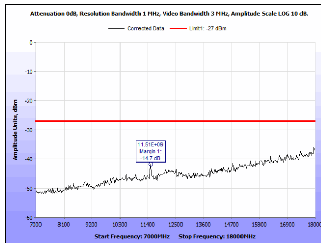
Plot 84. Radiated Spurious Emissions, 5745 MHz, 802.11a 20 MHz, 7 GHz – 18 GHz
