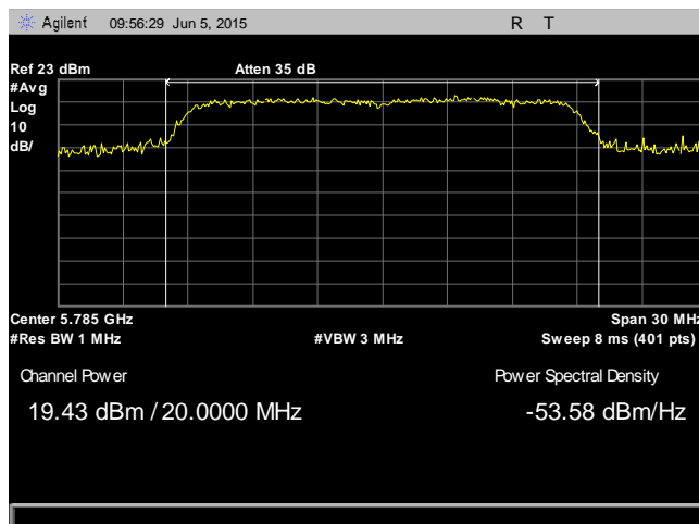
Plot 44. RF Output Power, 802.11n 20 MHz, Mid Channel, 5785 MHz, Antenna 2
