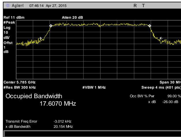
Plot 125. Occupied Bandwidth, 802.11n 20 MHz, Mid Channel, 5785 MHz, Antenna 2
