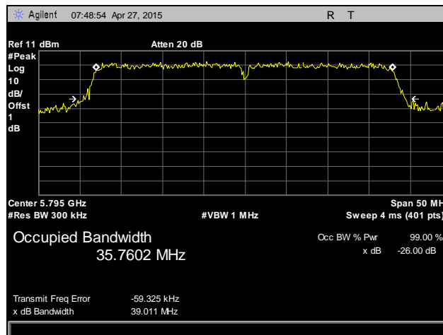
Plot 135. Occupied Bandwidth, 802.11n 40 MHz, High Channel, 5795 MHz, Antenna 2
