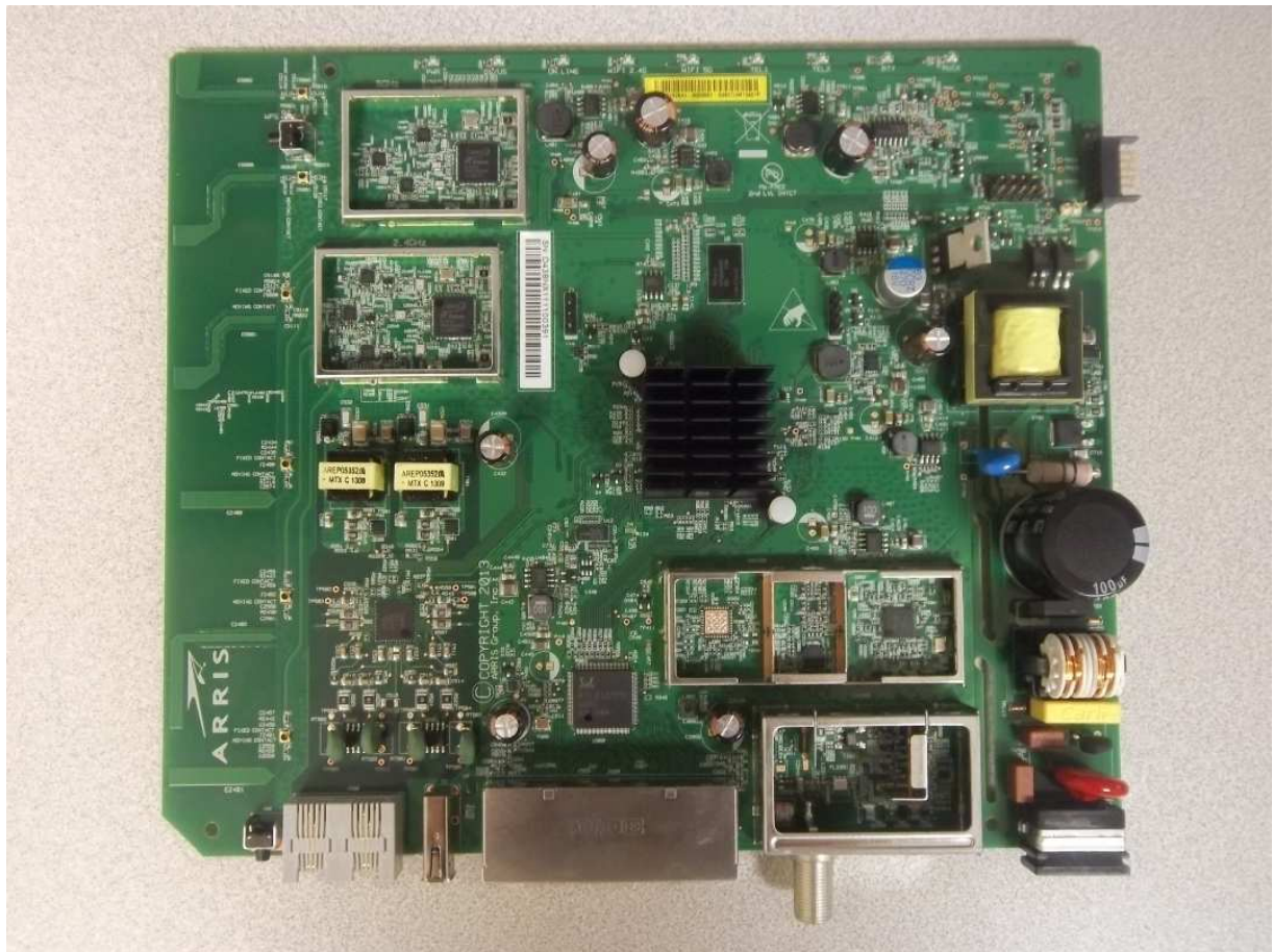
Figure 4: Internal Photo – TG1662G –Shields Removed
