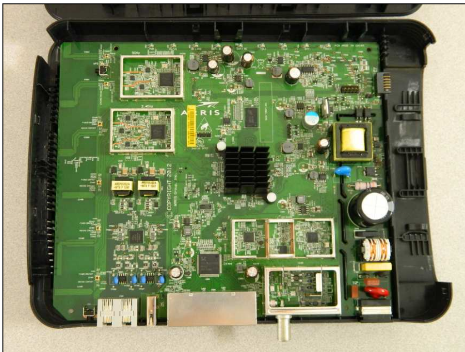
Figure 3: Internal Photo – TG1672G – Shields Removed
