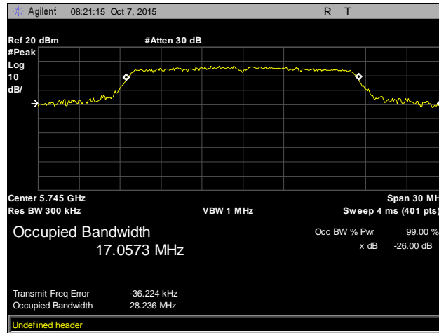
Plot 1. Occupied Bandwidth, Low Channel, 802.11a 20 MHz
