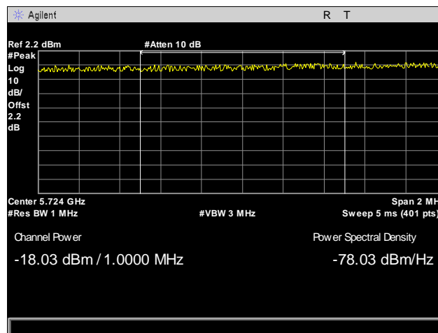
Plot 95. Radiated Band Edge, Channel 149, 802.11a 20 MHz, Integration at 5725 MHz
