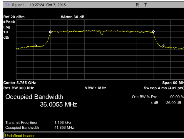
Plot 13. Occupied Bandwidth, Low Channel, 802.11n 40 MHz
