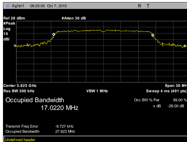
Plot 3. Occupied Bandwidth, High Channel, 802.11a 20 MHz
