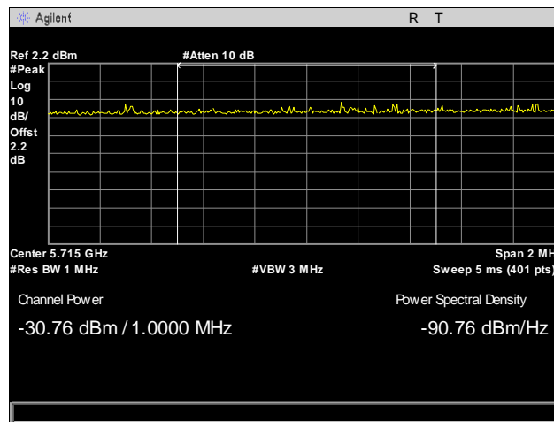
Plot 93. Radiated Band Edge, Channel 149, 802.11a 20 MHz, Integration at 5715 MHz
