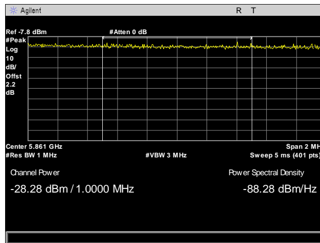
Plot 92. Radiated Band Edge, Channel 165, 802.11a 20 MHz, Integration at 5860 MHz
