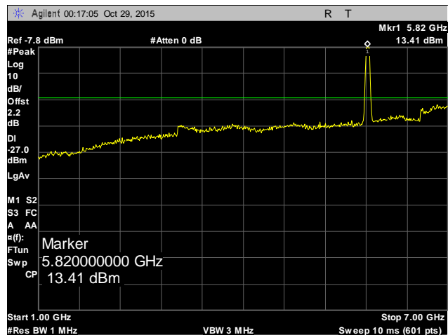
Plot 75. Radiated Spurious Emissions, Above 1 GHz, High Channel, 802.11a
