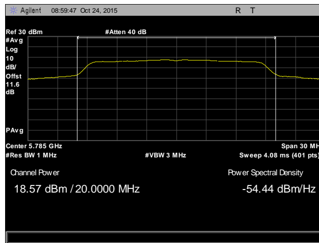
Plot 37. Conducted Output Power, Mid Channel, 802.11n 20 MHz, Antenna 1
