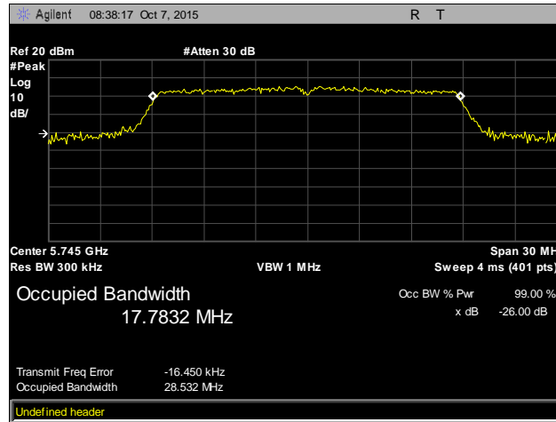
Plot 4. Occupied Bandwidth, Low Channel, 802.11ac 20 MHz
