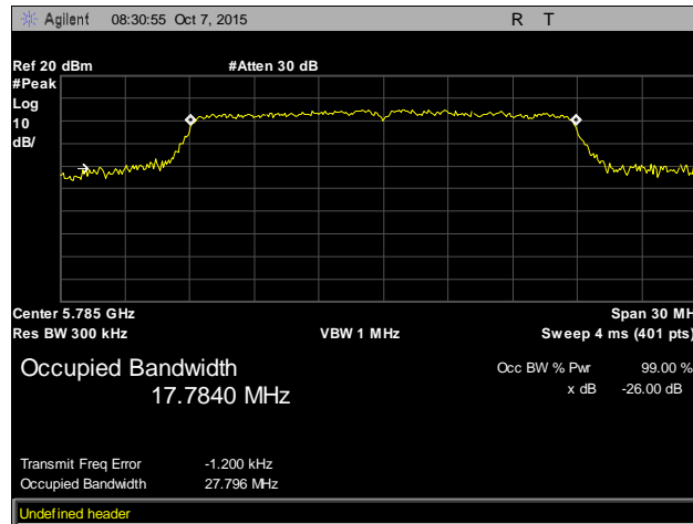
Plot 11. Occupied Bandwidth, Mid Channel, 802.11n 20 MHz
