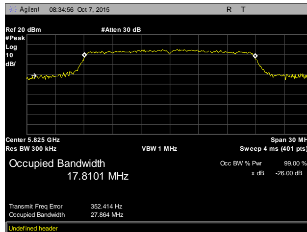
Plot 6. Occupied Bandwidth, High Channel, 802.11ac 20 MHz
