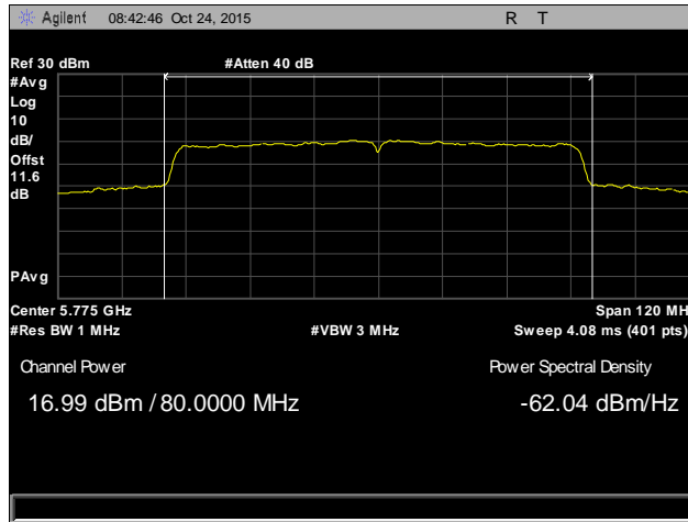
Plot 31. Conducted Output Power, 802.11ac 80 MHz, Antenna 0
