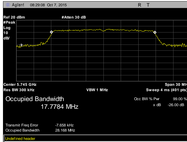
Plot 10. Occupied Bandwidth, Low Channel, 802.11n 20 MHz
