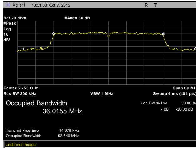
Plot 7. Occupied Bandwidth, Low Channel, 802.11ac 40 MHz
