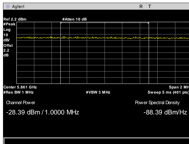
Plot 101. Radiated Band Edge, Channel 165, 802.11ac 20 MHz, Integration at 5860 MHz
