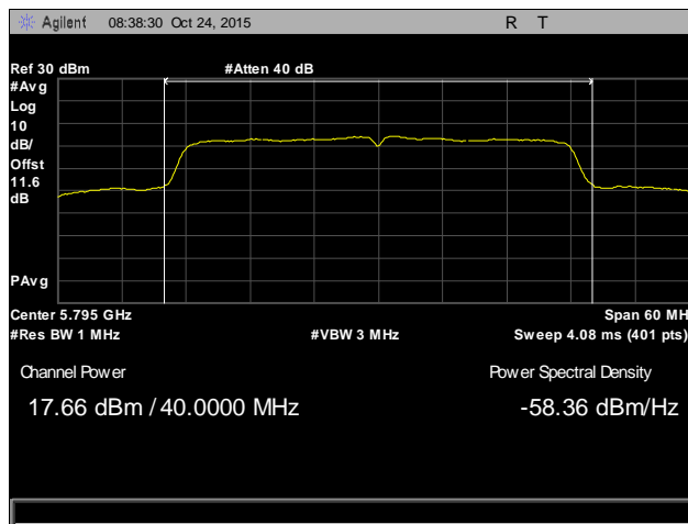
Plot 28. Conducted Output Power, High Channel, 802.11ac 40 MHz, Antenna 0
