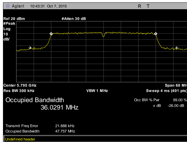
Plot 14. Occupied Bandwidth, High Channel, 802.11n 40 MHz
