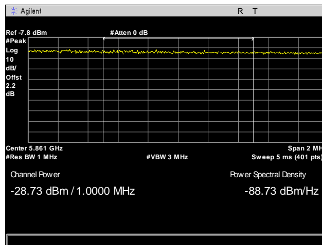
Plot 120. Radiated Band Edge, Channel 165, 802.11n 20 MHz, Integration at 5860 MHz
