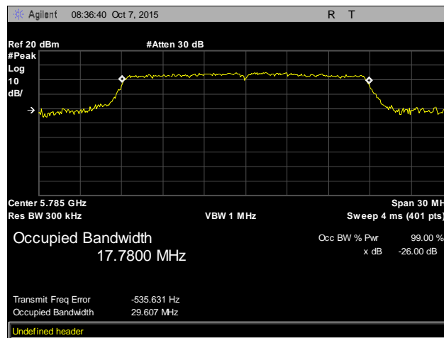
Plot 5. Occupied Bandwidth, Mid Channel, 802.11ac 20 MHz
