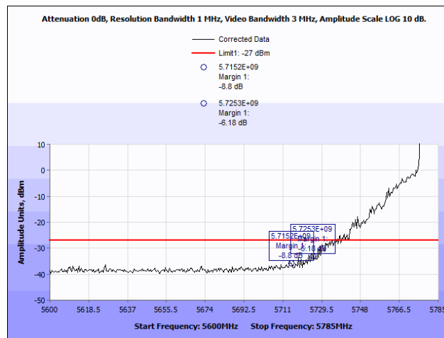
Plot 98. Radiated Band Edge, Mid Channel, 802.11ac 20 MHz
