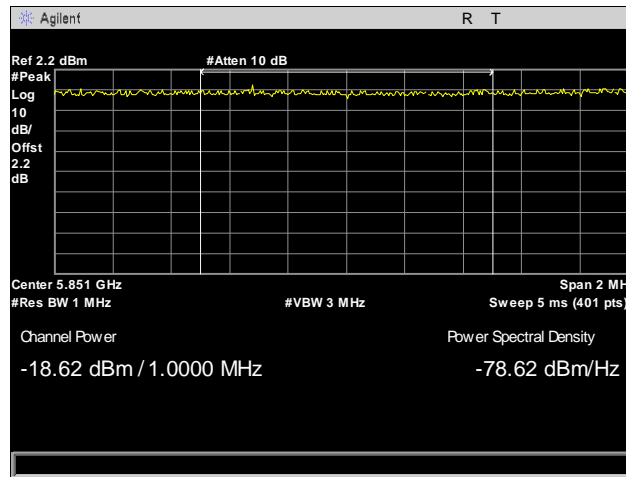
Plot 91. Radiated Band Edge, Channel 165, 802.11a, Integration at 5850 MHz
