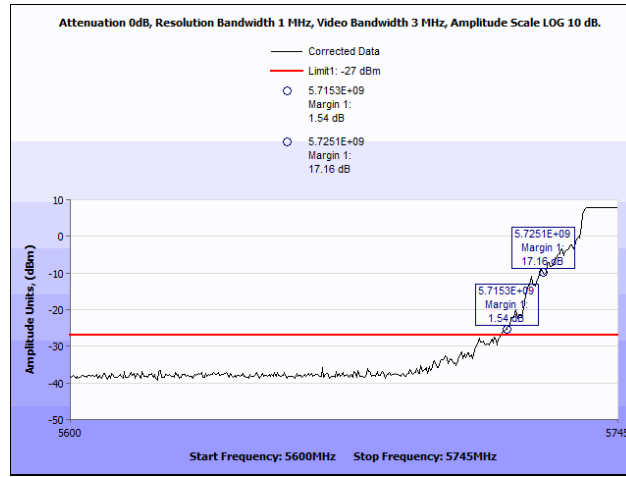
Plot 116. Radiated Band Edge, Low Channel, 802.11n 20 MHz
