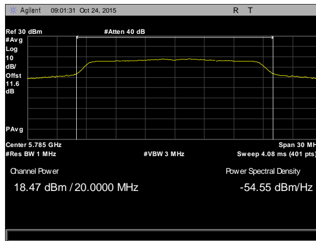
Plot 25. Conducted Output Power, Mid Channel, 802.11ac 20 MHz, Antenna 1
