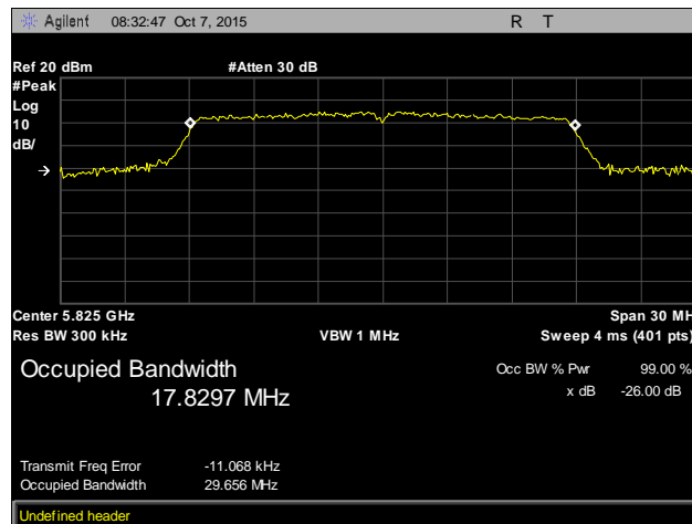
Plot 12. Occupied Bandwidth, High Channel, 802.11n 20 MHz
