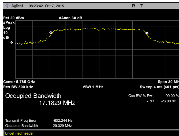
Plot 2. Occupied Bandwidth, Mid Channel, 802.11a 20 MHz
