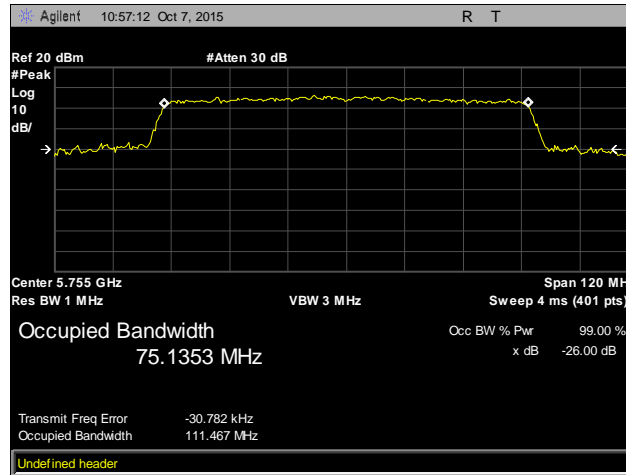
Plot 9. Occupied Bandwidth, 802.11ac 80 MHz
