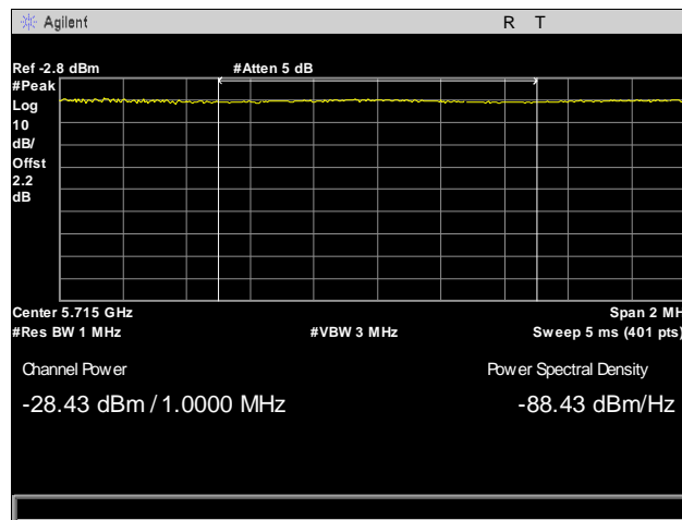
Plot 114. Radiated Band Edge, Channel 155, 802.11ac 40 MHz, Integration at 5715 MHz
