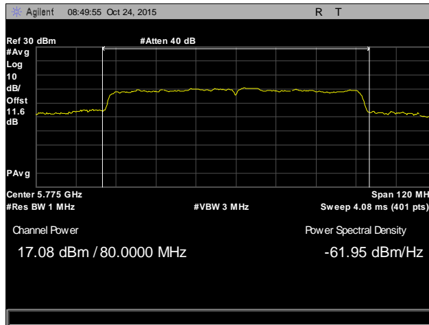
Plot 32. Conducted Output Power, 802.11ac 80 MHz, Antenna 1
