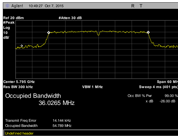
Plot 8. Occupied Bandwidth, High Channel, 802.11ac 40 MHz
