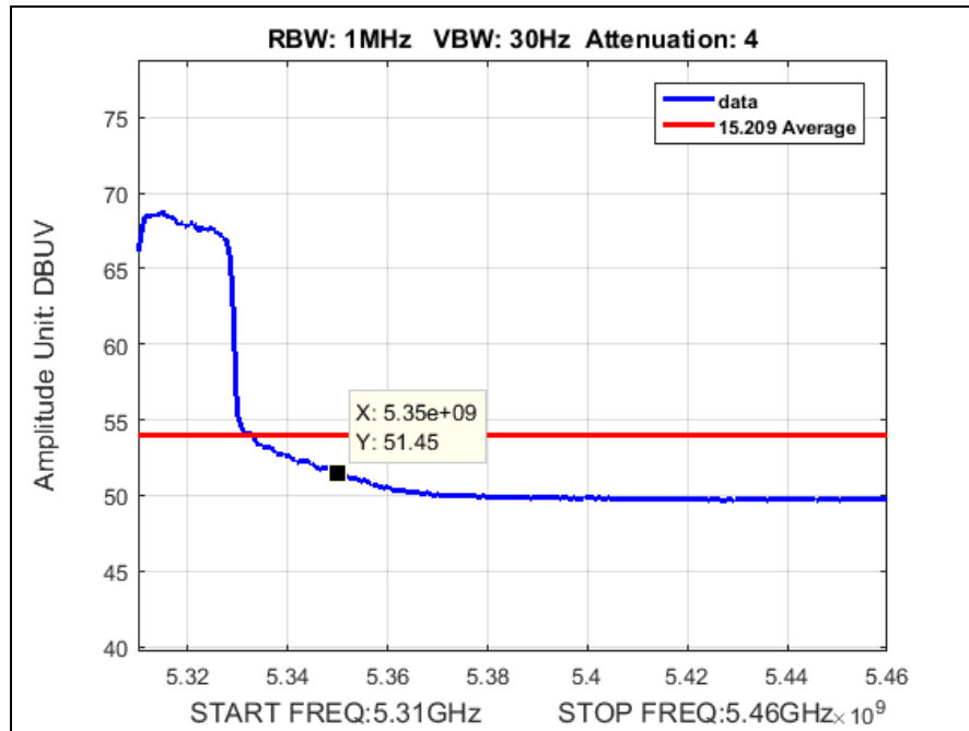
Plot 175. Radiated Band Edge, 5310 MHz, 802.1n 40 MHz, Average
