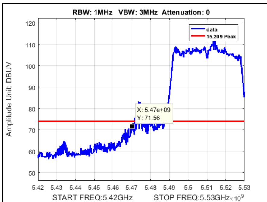
Plot 159. Radiated Band Edge, 5510 MHz, 802.11ac 40 MHz, Peak
