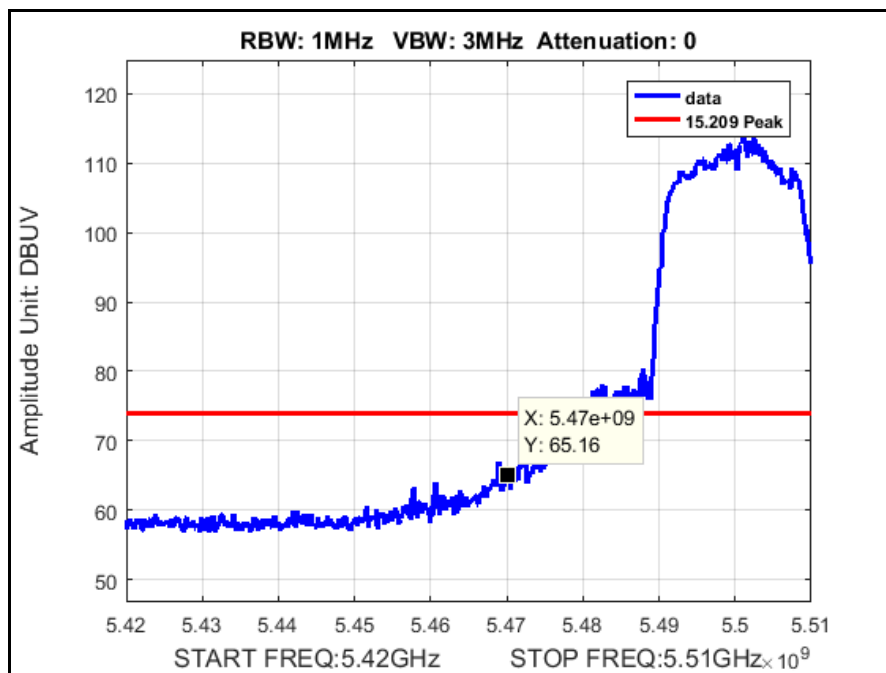
Plot 152. Radiated Band Edge, 5500 MHz, 802.11ac 20 MHz, Peak
