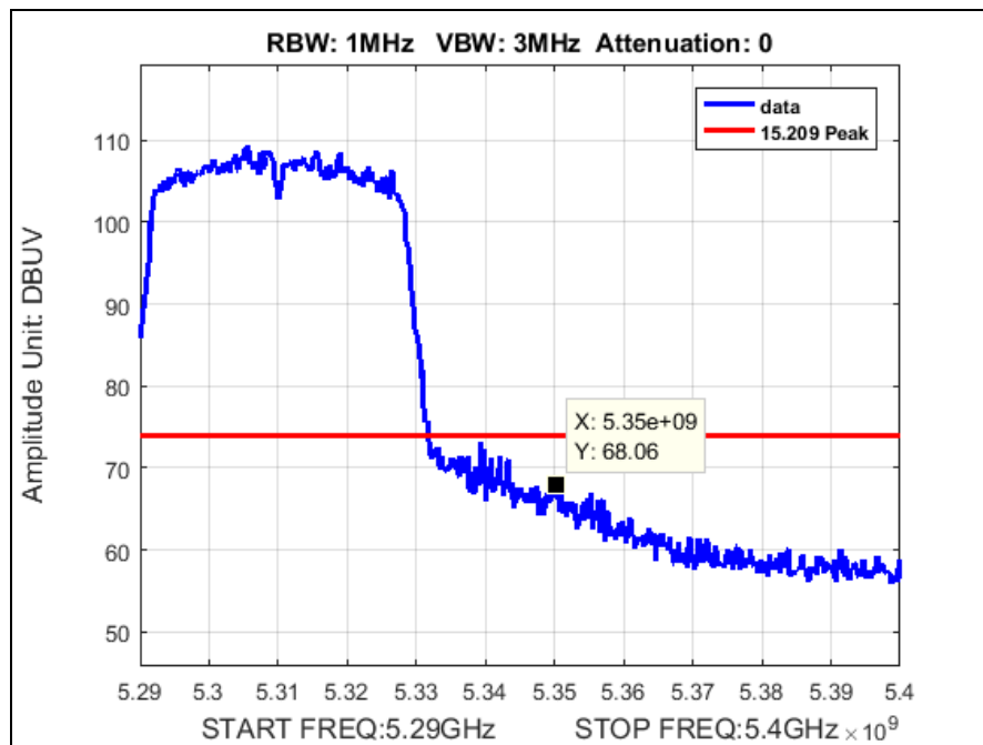
Plot 176. Radiated Band Edge, 5310 MHz, 802.1n 40 MHz, Peak
