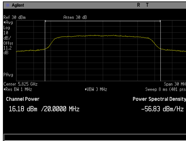
Plot 7. Maximum Conducted Output Power, BW 20M, Ch 5825M, 80211a MSC0 P3230, CH0
