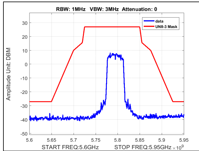
Plot 52. Band Edge, BW 40M, Ch 5795M, 80211n, MCS24, P3230
