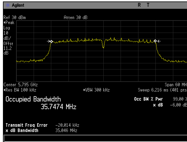
Plot 68. 6 dB Bandwidth, BW 40M, Ch 5795M, 80211n, MCS16, P3230, CH0
