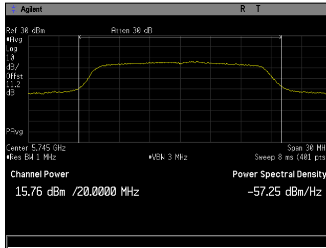
Plot 1. Maximum Conducted Output Power, BW 20M, Ch 5745M, 80211a, MSC0, P3230, CH0
