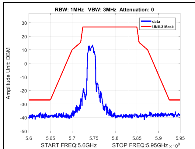
Plot 44. Band Edge, BW 20M, Ch 5745M, 80211ac, MCS24, P3230
