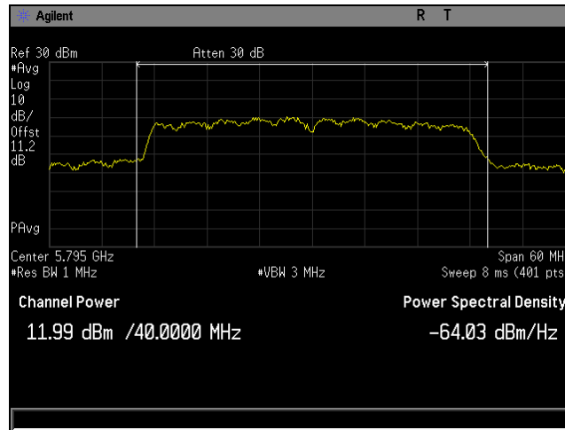
Plot 13. Maximum Conducted Output Power, BW 40M, Ch 5795M, 80211n, MSC24, P3230, CH0
