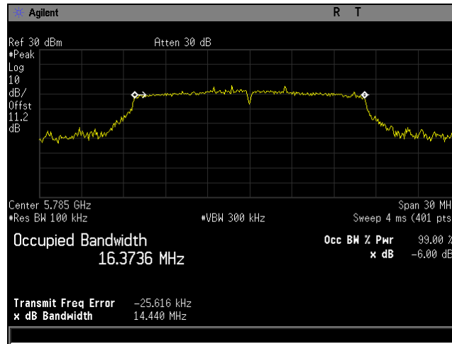
Plot 59. 6 dB Bandwidth, BW 20M, Ch 5785M, 80211a, MCS0, P3230, CH0
