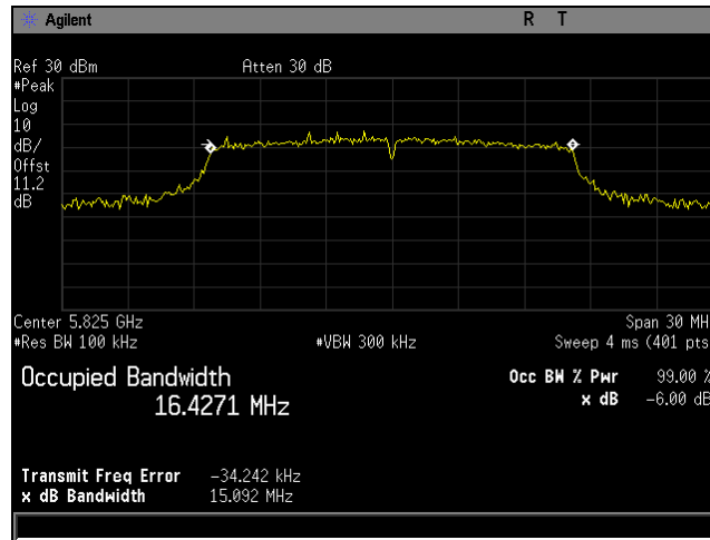
Plot 62. 6 dB Bandwidth, BW 20M, Ch 5825M, 80211a, MCS0, P3230, CH0
