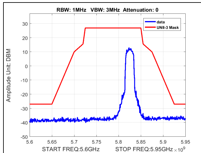
Plot 47. Band Edge, BW 20M, Ch 5825M, 80211ac, MCS24, P3230
