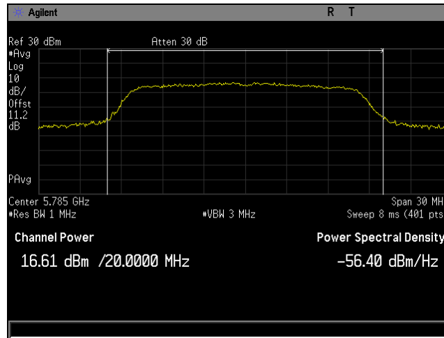
Plot 4. Maximum Conducted Output Power, BW 20M, Ch 5785M, 80211a, MSC0, P3230, CH0
