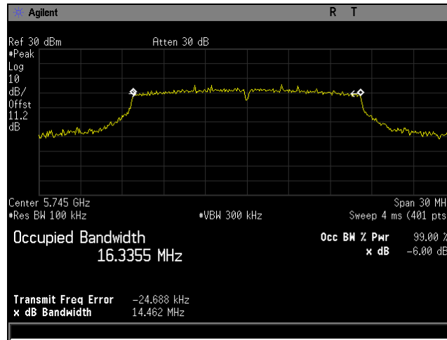
Plot 56. 6 dB Bandwidth, BW 20M, Ch 5745M, 80211a, MCS0, P3230, CH0
