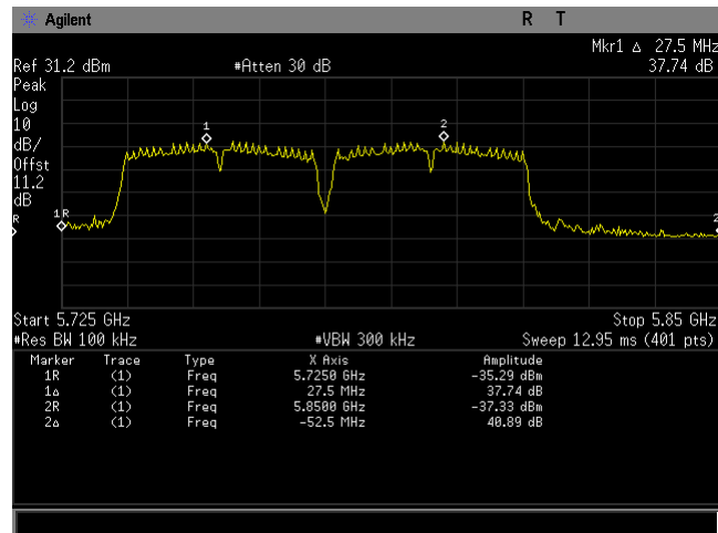
Plot 74. Frequency Stability, 80211ac BW 40MHz
