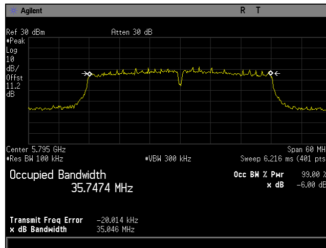
Plot 67. 6 dB Bandwidth, BW 40M, Ch 5795M, 80211ac, MCS24, P3230, CH0
