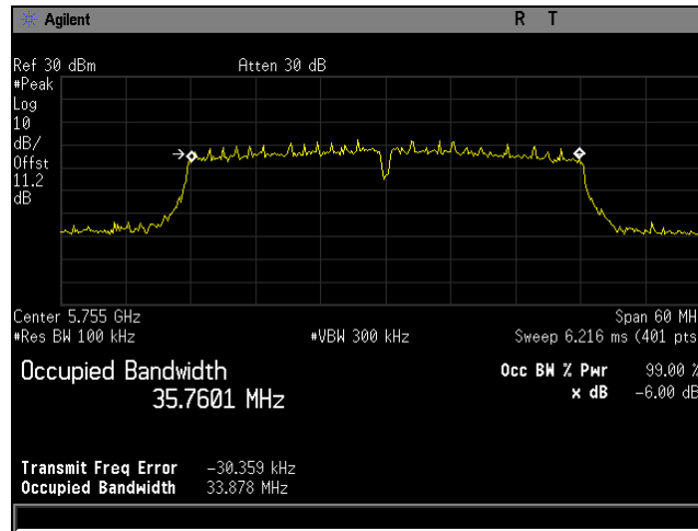
Plot 65. 6 dB Bandwidth, BW 40M, Ch 5755M, 80211ac, MCS24, P3230, CH0
