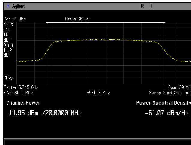
Plot 3. Maximum Conducted Output Power, BW 20M, Ch 5745M, 80211n, MSC24, P3230, CH0
