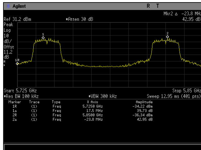
Plot 84. Frequency Stability, 80211n BW 20MHz
