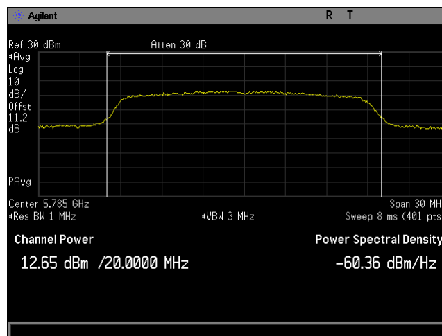
Plot 6. Maximum Conducted Output Power, BW 20M, Ch 5785M, 80211n, MSC24, P3230, CH0
