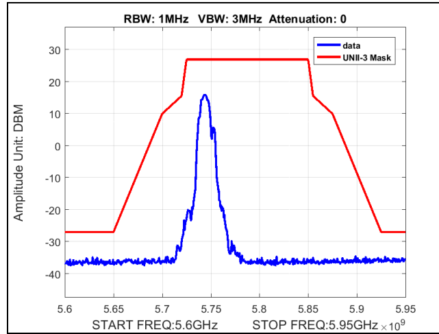
Plot 43. Band Edge, BW 20M, Ch 5745M, 80211a, MCS0, P3230
