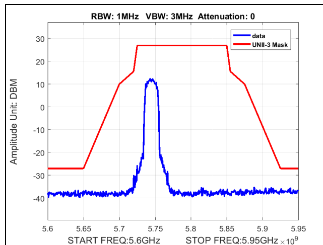
Plot 45. Band Edge, BW 20M, Ch 5745M, 80211n, MCS24, P3230
