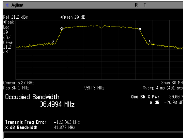
Plot 27. 26 dB Occupied Bandwidth, 5270 MHz, 802.11n 40 MHz
