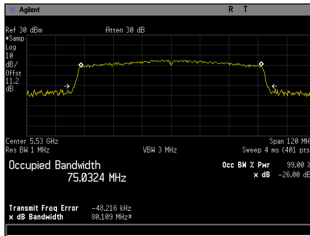
Plot 19. 26 dB Occupied Bandwidth, 5530 MHz, 802.11ac 80 MHz
