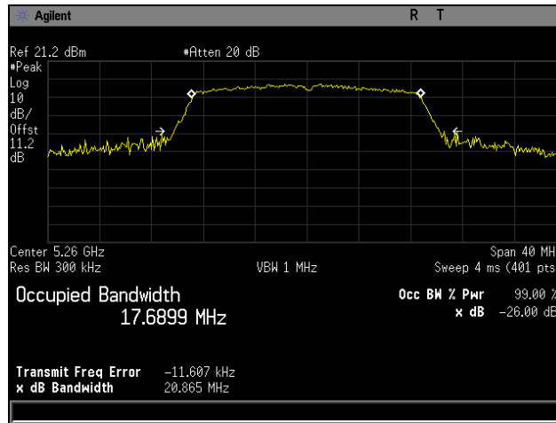
Plot 21. 26 dB Occupied Bandwidth, 5260 MHz, 802.11n 20 MHz
