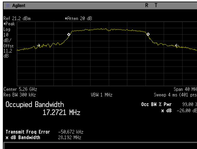
Plot 1. 26 dB Occupied Bandwidth, 5260 MHz, 802.11a
