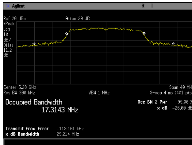
Plot 2. 26 dB Occupied Bandwidth, 5280 MHz, 802.11a
