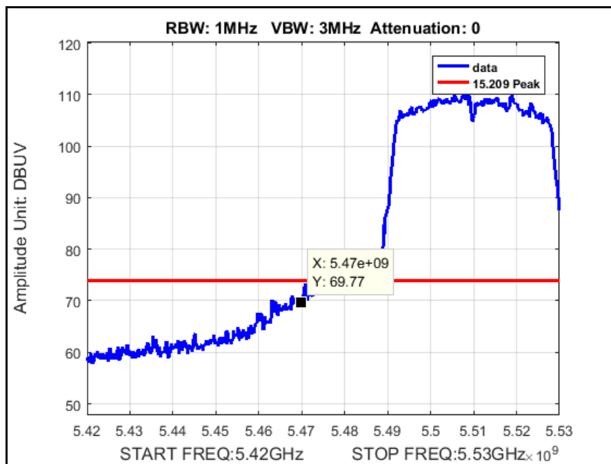
Plot 178. Radiated Band Edge, 5510 MHz, 802.11n 40 MHz, Peak
