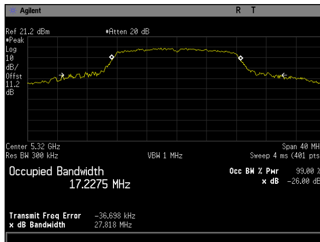
Plot 3. 26 dB Occupied Bandwidth, 5320 MHz, 802.11a
