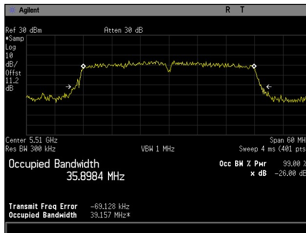
Plot 29. 26 dB Occupied Bandwidth, 5510 MHz, 802.11n 40 MHz
