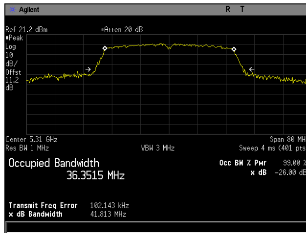
Plot 28. 26 dB Occupied Bandwidth, 5310 MHz, 802.11n 40 MHz
