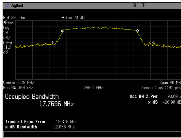
Plot 22. 26 dB Occupied Bandwidth, 5280 MHz, 802.11n 20 MHz
