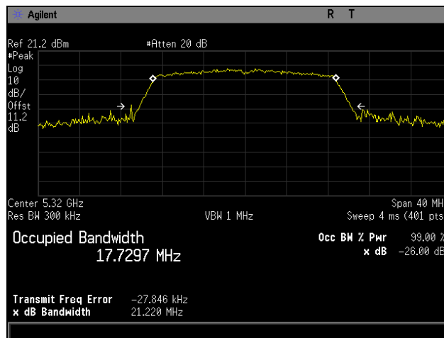
Plot 9. 26 dB Occupied Bandwidth, 5320 MHz, 802.11ac 20 MHz
