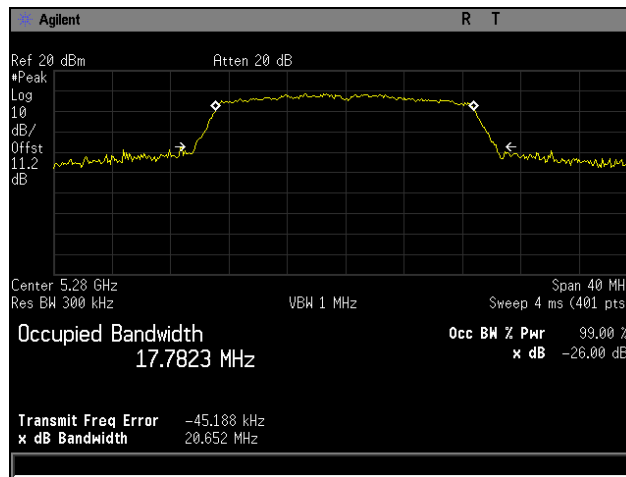
Plot 8. 26 dB Occupied Bandwidth, 5280 MHz, 802.11ac 20 MHz
