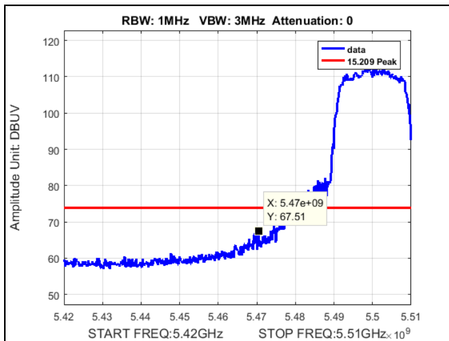
Plot 171. Radiated Band Edge, 5500 MHz, 802.11n 20 MHz, Peak
