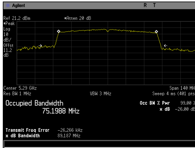
Plot 18. 26 dB Occupied Bandwidth, 5290 MHz, 802.11ac 80 MHz
