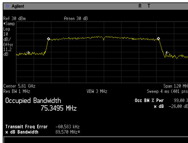
Plot 20. 26 dB Occupied Bandwidth, 5610 MHz, 802.11ac 80 MHz
