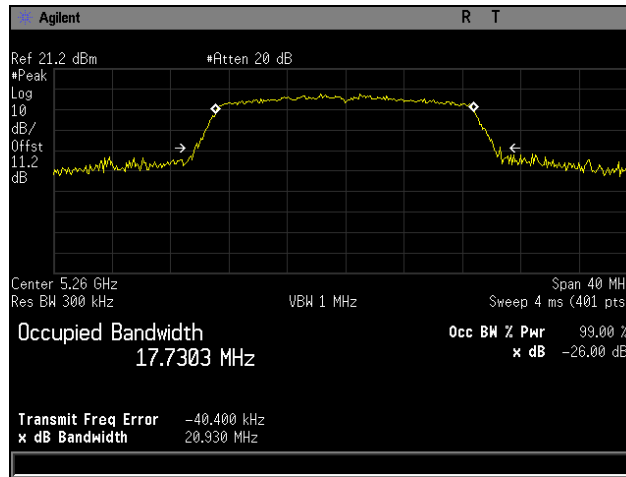
Plot 7. 26 dB Occupied Bandwidth, 5260 MHz, 802.11ac 20 MHz
