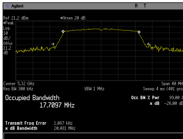
Plot 23. 26 dB Occupied Bandwidth, 5320 MHz, 802.11n 20 MHz
