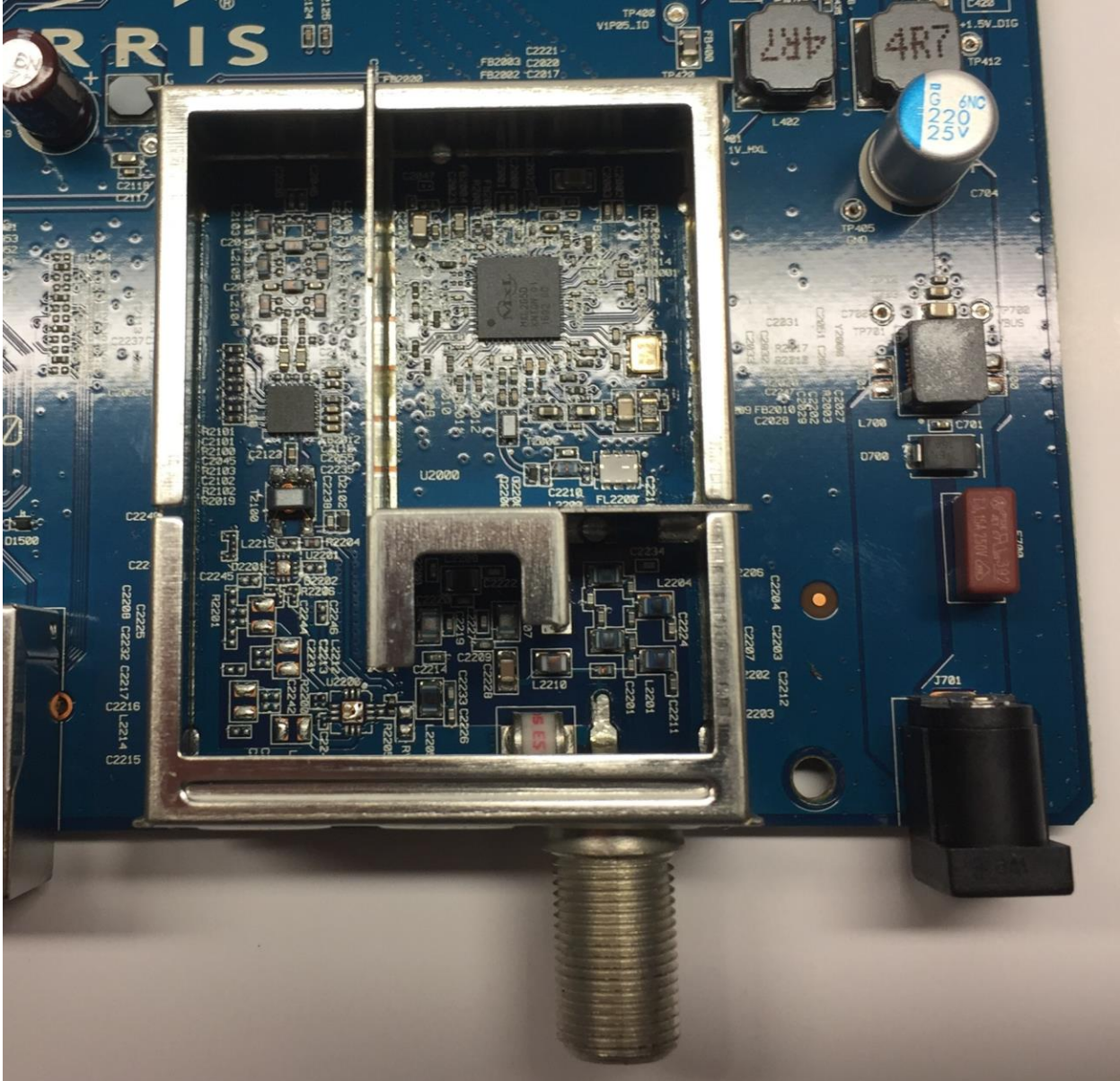
Photograph 4. RF can cover removed
