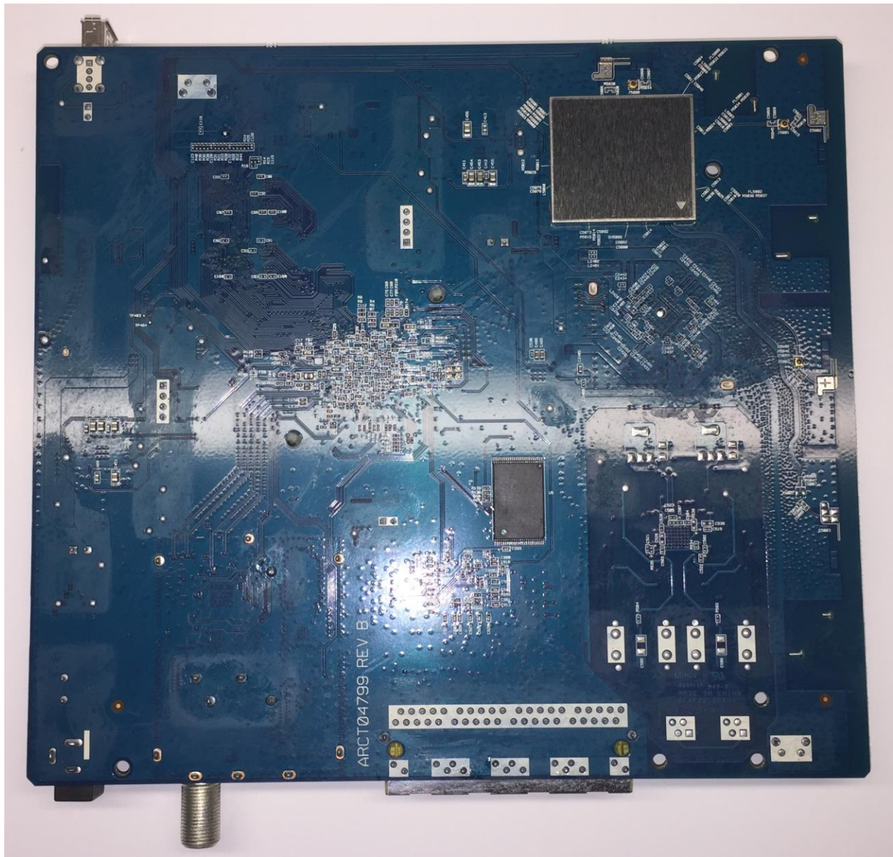
Photograph 3. PWB Bottom view
