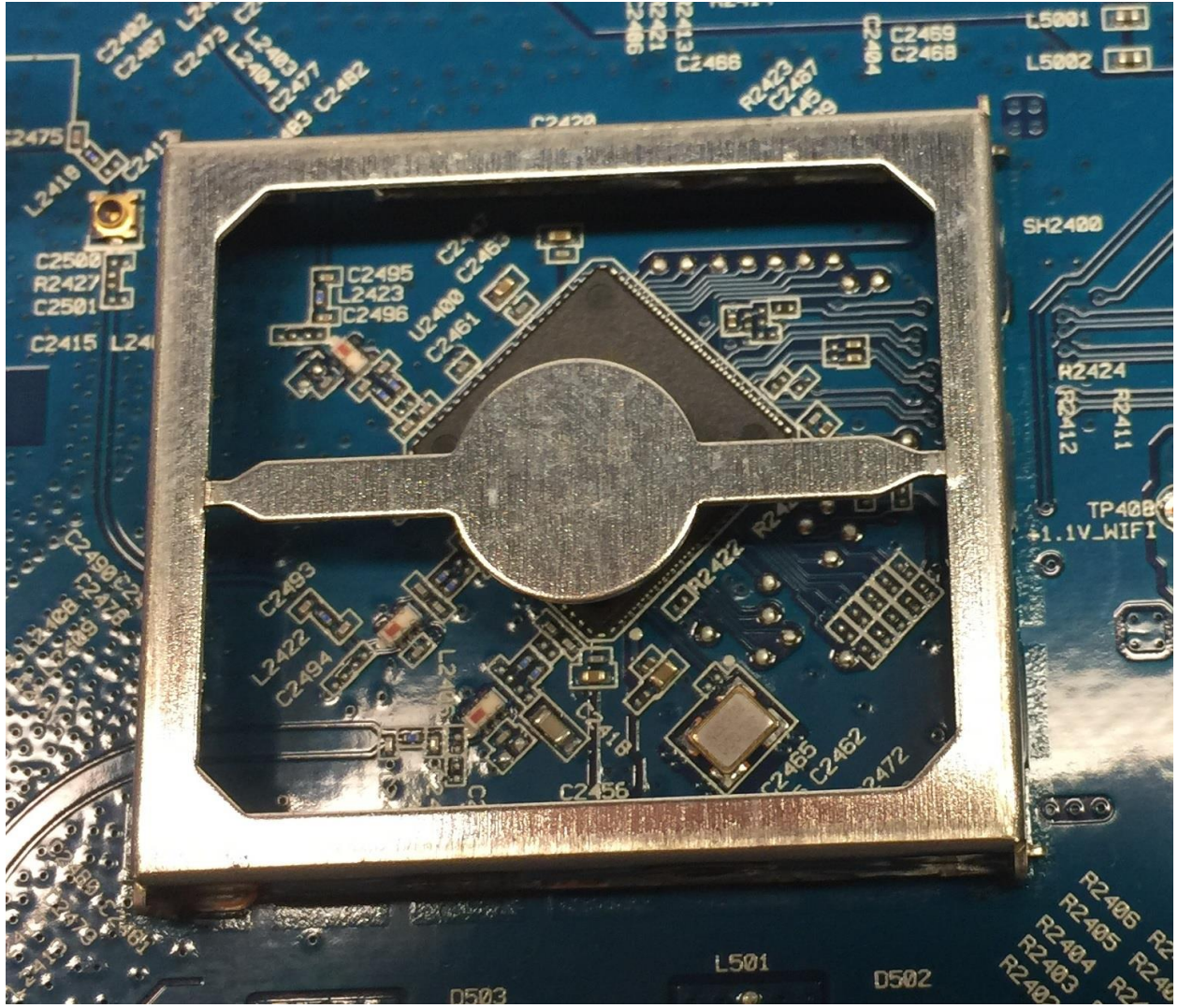
Photograph 1. 2.4GHz Chip can cover removed
