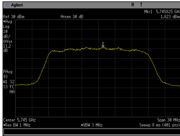
Plot 24. Maximum Power Spectral Density, Low Channel, 802.11n 20 MHz, Channel 0
