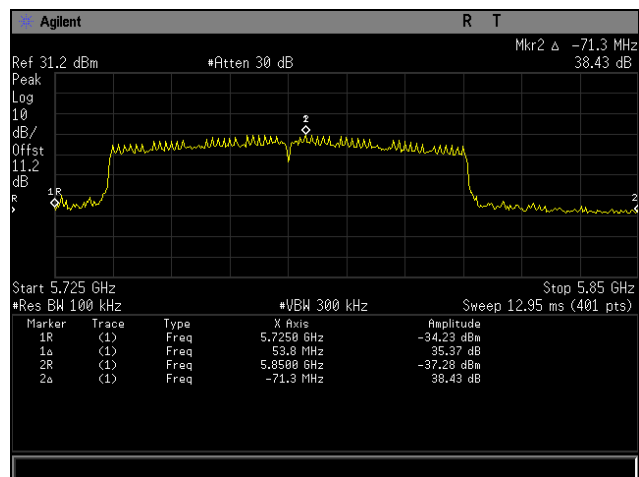
Plot 73. Frequency Stability, 80211ac 80MHz, -20°C 97VAC
