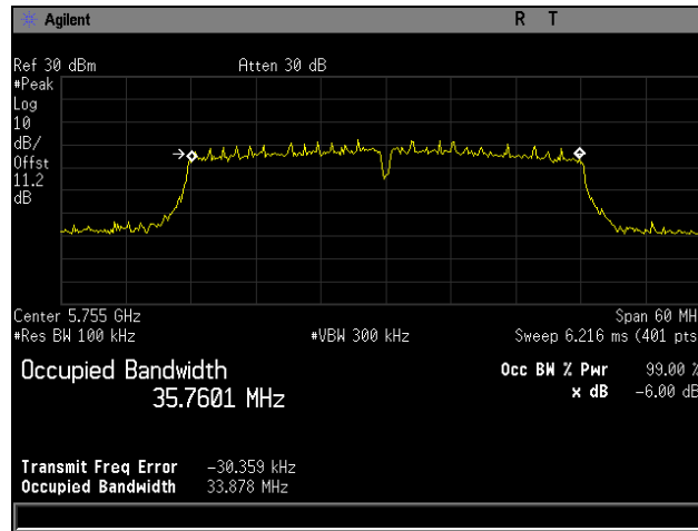
Plot 60. 6 dB Occupied Bandwidth, Low Channel, 802.11ac 40 MHz
