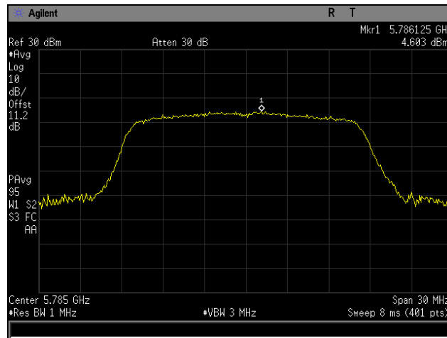
Plot 16. Maximum Power Spectral Density, Mid Channel, 802.11a, Channel 0
