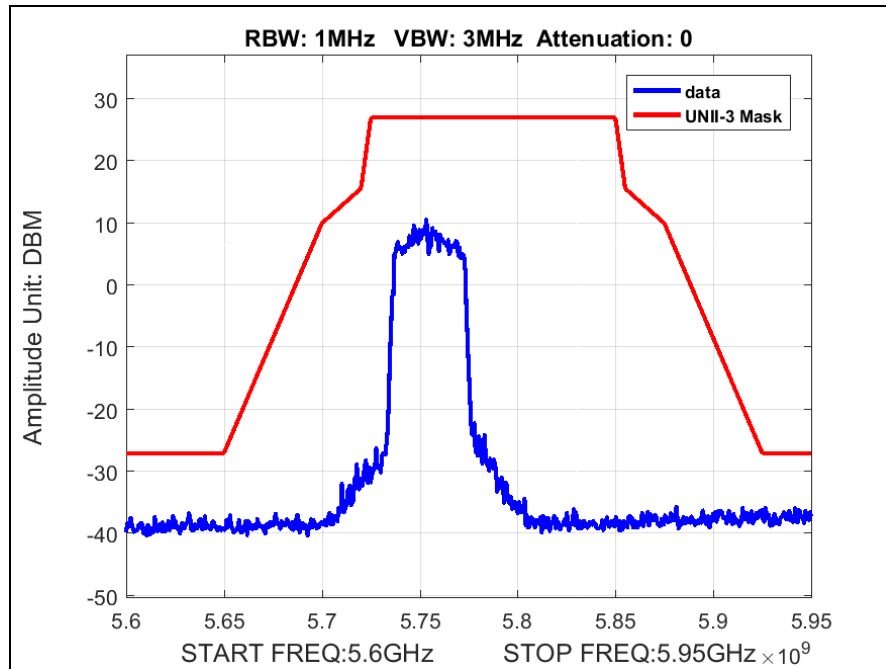
Plot 45. Radiated Band Edge, Low Channel, 802.11ac 40 MHz
