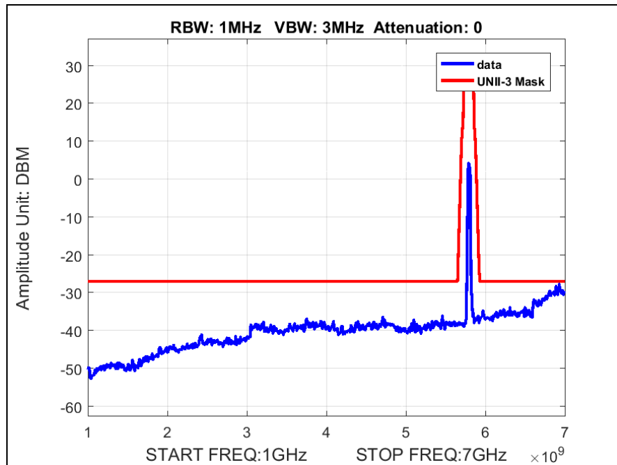
Plot 35. Radiated Spurious Emissions, High Channel, 802.11ac 40 MHz, 1 GHz – 7 GHz
