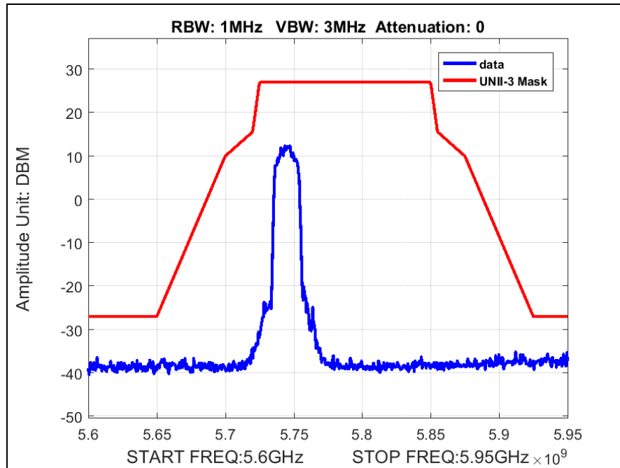
Plot 43. Radiated Band Edge, Low Channel, 802.11ac 20 MHz
