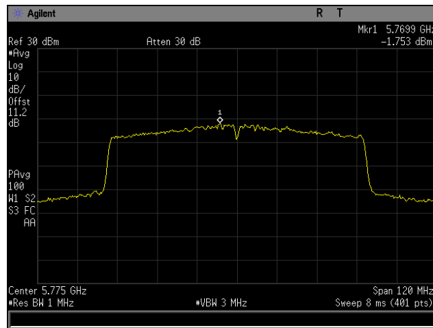
Plot 23. Maximum Power Spectral Density, 802.11ac 80 MHz, Channel 0
