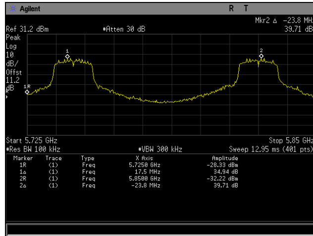
Plot 74. Frequency Stability, 80211a 20 MHz, 20°C 115VAC
