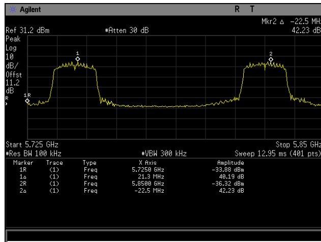
Plot 69. Frequency Stability, 80211ac 20 MHz, -20°C 97VAC
