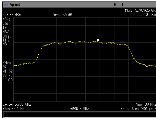
Plot 25. Maximum Power Spectral Density, Mid Channel, 802.11n 20 MHz, Channel 0
