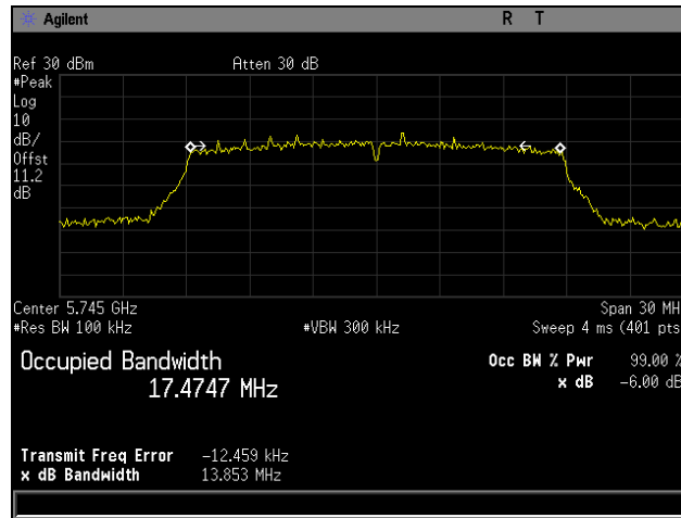
Plot 57. 6 dB Occupied Bandwidth, Low Channel, 802.11ac 20 MHz
