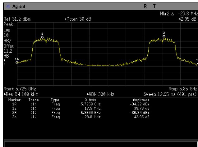
Plot 82. Frequency Stability, 80211n 20 MHz, 40°C 133VAC
