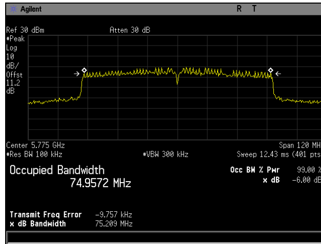
Plot 62. 6 dB Occupied Bandwidth, 802.11ac 80 MHz
