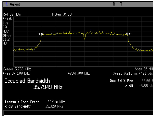
Plot 66. 6 dB Occupied Bandwidth, Low Channel, 802.11n 40 MHz
