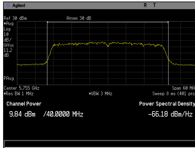
Plot 7. Maximum Conducted Output Power, Low Channel, 802.11ac 40 MHz, Channel 0
