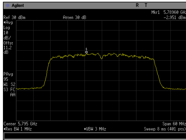
Plot 22. Maximum Power Spectral Density, High Channel, 802.11ac 40 MHz, Channel 0
