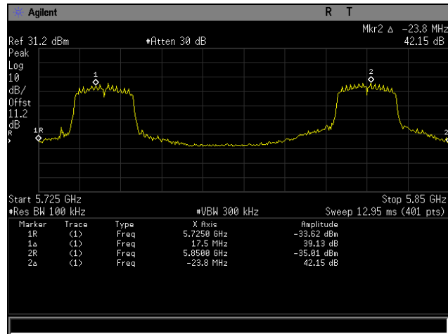
Plot 81. Frequency Stability, 80211ac 20 MHz, 40°C 133VAC
