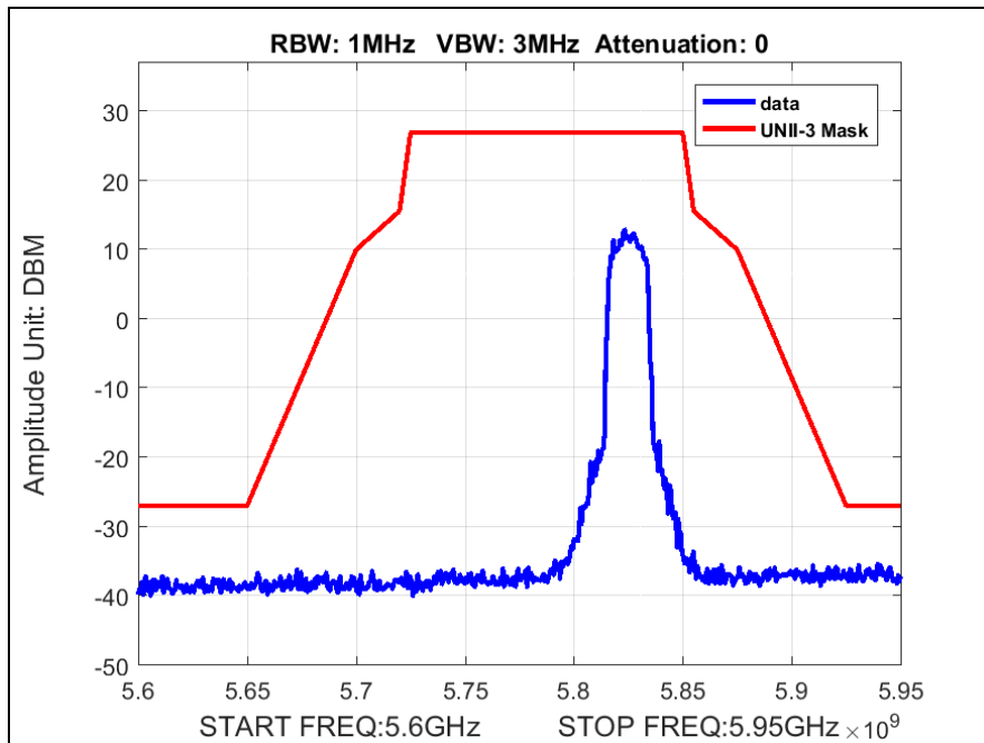
Plot 49. Radiated Band Edge, High Channel, 802.11n 20 MHz
