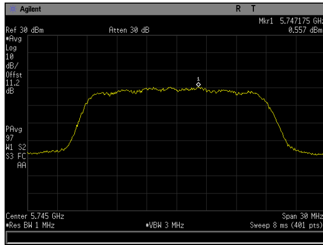
Plot 18. Maximum Power Spectral Density, Low Channel, 802.11ac 20 MHz, Channel 0
