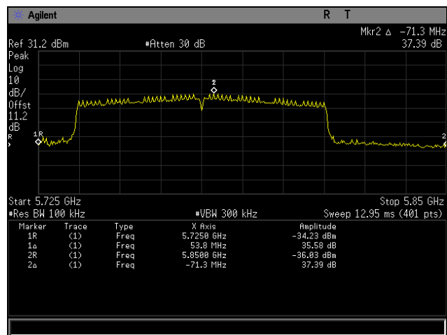
Plot 79. Frequency Stability, 80211ac 80 MHz, 20°C 115VAC
