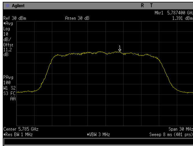
Plot 19. Maximum Power Spectral Density, Mid Channel, 802.11ac 20 MHz, Channel 0
