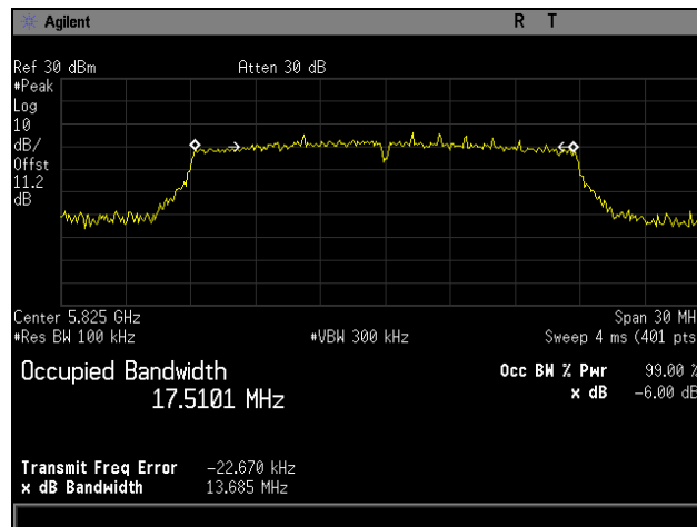
Plot 59. 6 dB Occupied Bandwidth, High Channel, 802.11ac 20 MHz
