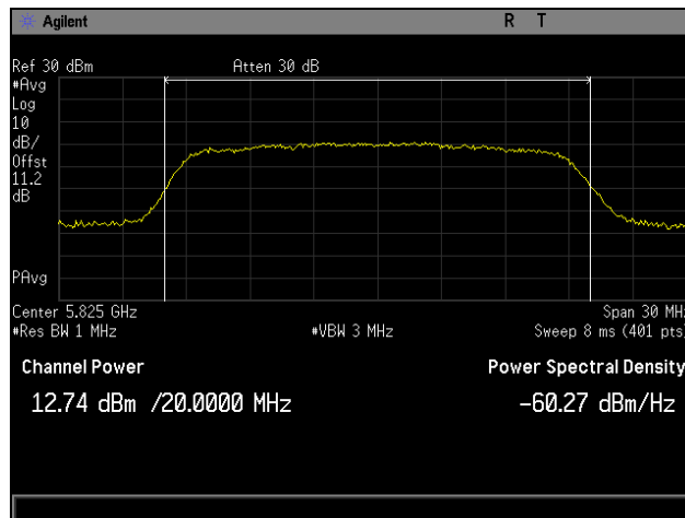
Plot 6. Maximum Conducted Output Power, High Channel, 802.11ac 20 MHz, Channel 0
