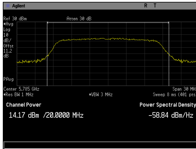
Plot 2. Maximum Conducted Output Power, Mid Channel, 802.11a, Channel 0
