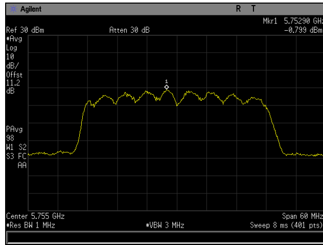
Plot 27. Maximum Power Spectral Density, Low Channel, 802.11n 40 MHz, Channel 0
