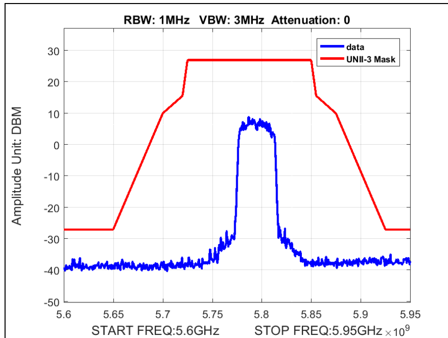
Plot 46. Radiated Band Edge, High Channel, 802.11ac 40 MHz
