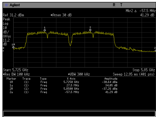
Plot 84. Frequency Stability, 80211ac 40 MHz, 40°C 133VAC
