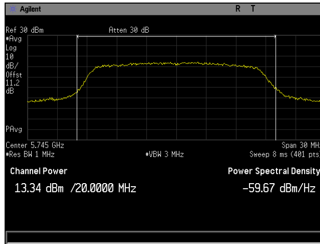
Plot 1. Maximum Conducted Output Power, Low Channel, 802.11a, Channel 0
