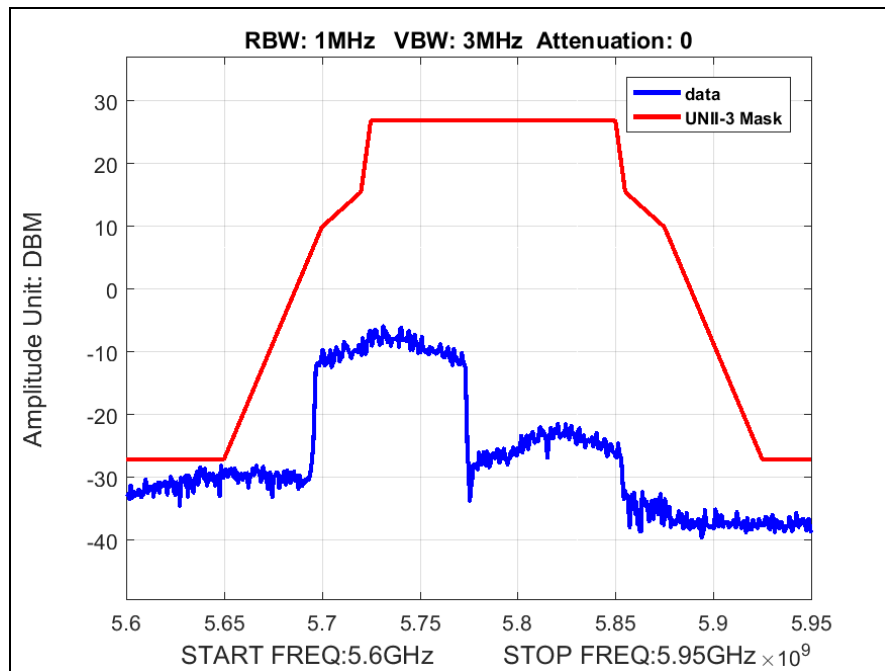
Plot 47. Radiated Band Edge, 802.11ac 80 MHz, P2321
