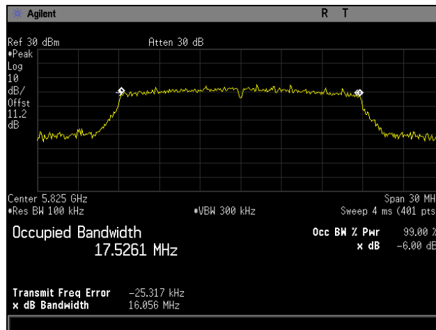
Plot 65. 6 dB Occupied Bandwidth, High Channel, 802.11n 20 MHz
