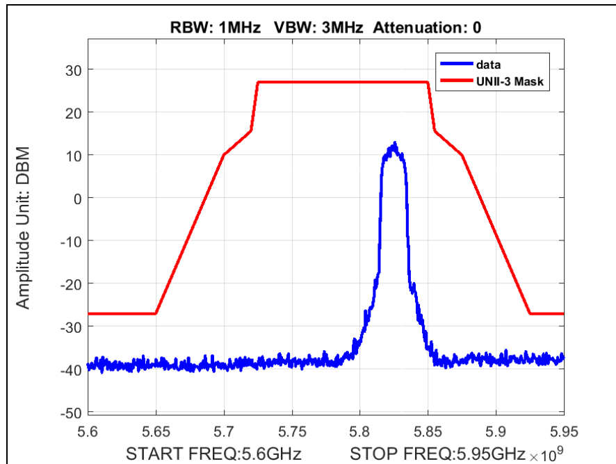
Plot 44. Radiated Band Edge, High Channel, 802.11ac 20 MHz
