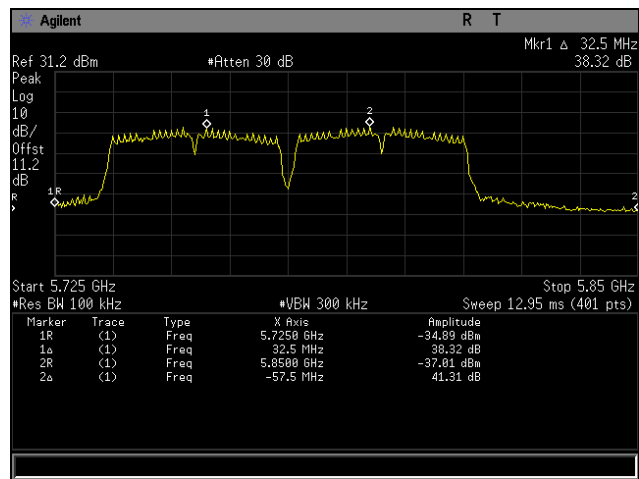
Plot 78. Frequency Stability, 80211ac 40 MHz, 20°C 115VAC
