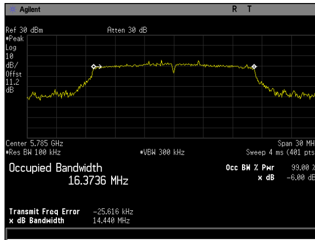
Plot 55. 6 dB Occupied Bandwidth, Mid Channel, 802.11a
