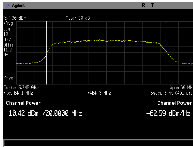
Plot 4. Maximum Conducted Output Power, Low Channel, 802.11ac 20 MHz, Channel 0
