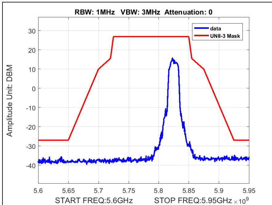
Plot 42. Radiated Band Edge, High Channel, 802.11a
