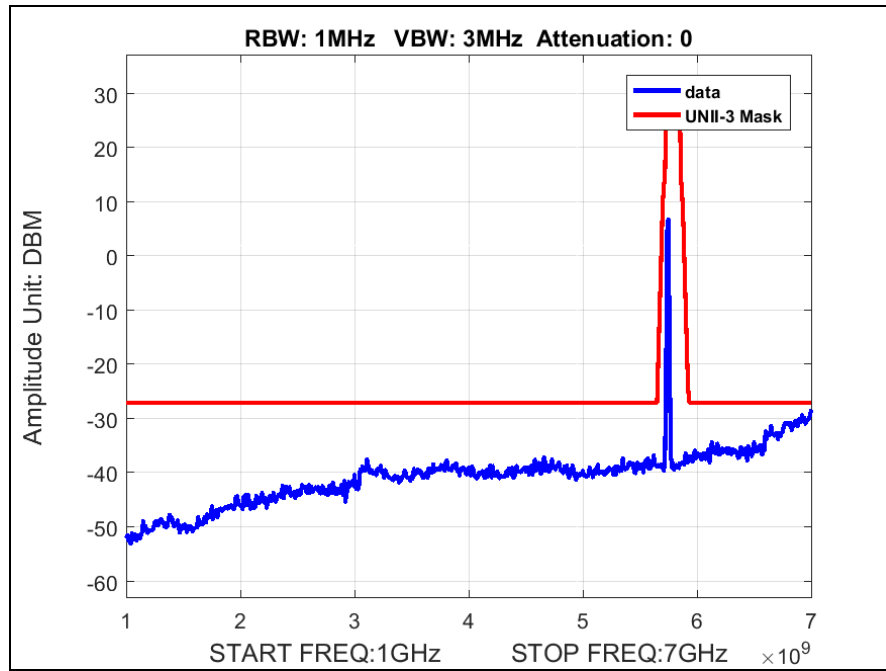
Plot 32. Radiated Spurious Emissions, Low Channel, 802.11ac 20 MHz, 1 GHz – 7 GHz
