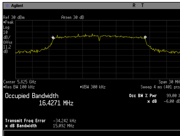
Plot 56. 6 dB Occupied Bandwidth, High Channel, 802.11a
