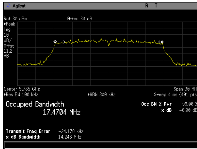
Plot 58. 6 dB Occupied Bandwidth, Mid Channel, 802.11ac 20 MHz
