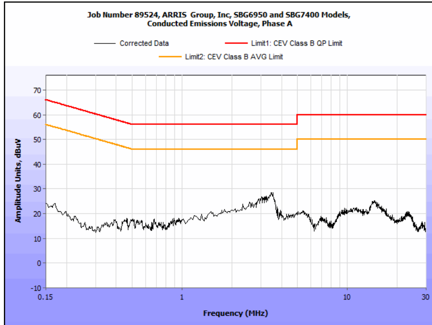
Plot 52. Conducted Emissions, 15.207(a), Phase Line
