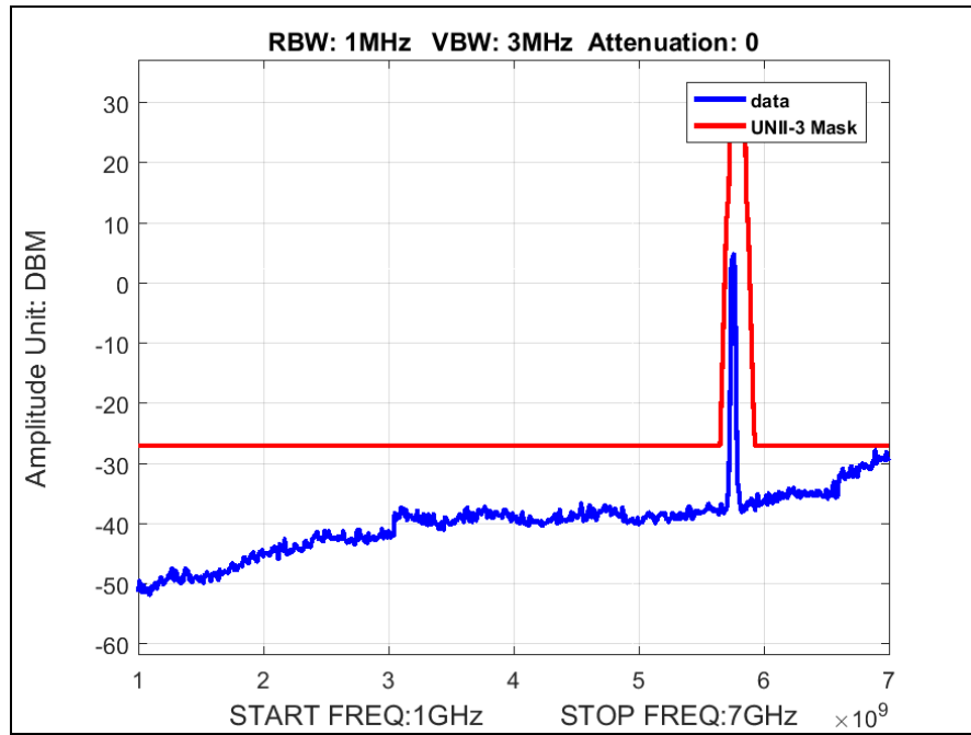
Plot 34. Radiated Spurious Emissions, Low Channel, 802.11ac 40 MHz, 1 GHz – 7 GHz
