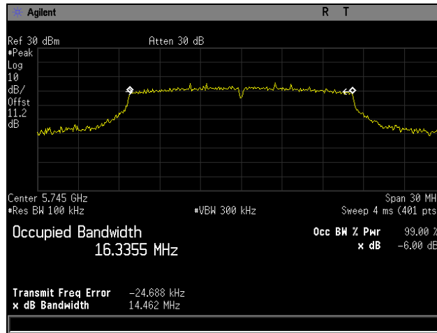
Plot 54. 6 dB Occupied Bandwidth, Low Channel, 802.11a
