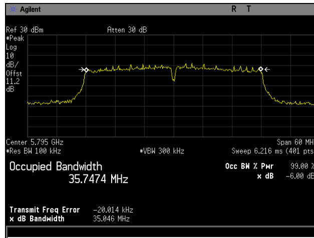
Plot 61. 6 dB Occupied Bandwidth, High Channel, 802.11ac 40 MHz
