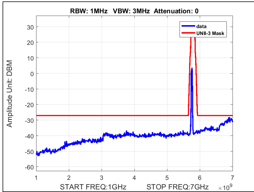
Plot 39. Radiated Spurious Emissions, Low Channel, 802.11n 40 MHz, 1 GHz – 7 GHz
