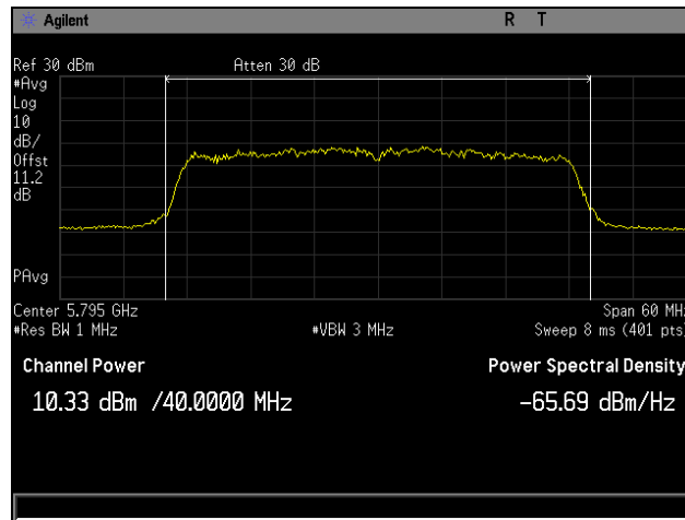
Plot 14. Maximum Conducted Output Power, High Channel, 802.11n 40 MHz, Channel 0
