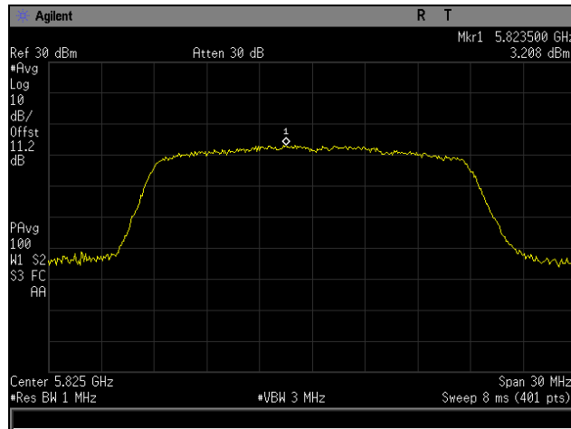
Plot 26. Maximum Power Spectral Density, High Channel, 802.11n 20 MHz, Channel 0
