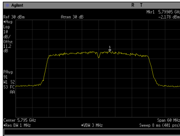
Plot 28. Maximum Power Spectral Density, High Channel, 802.11n 40 MHz, Channel 0
