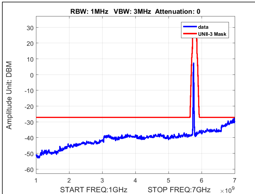
Plot 30. Radiated Spurious Emissions, Low Channel, 802.11a, 1 GHz – 7 GHz
