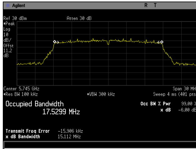
Plot 63. 6 dB Occupied Bandwidth, Low Channel, 802.11n 20 MHz
