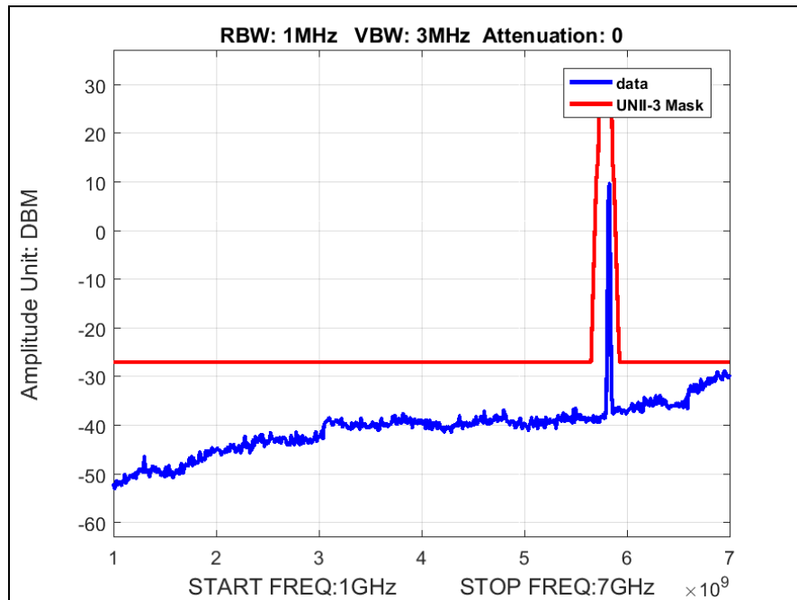
Plot 33. Radiated Spurious Emissions, High Channel, 802.11ac 20 MHz, 1 GHz – 7 GHz
