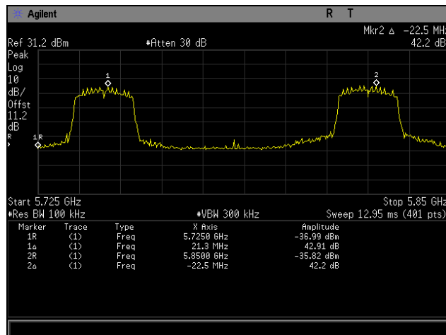
Plot 70. Frequency Stability, 80211n 20 MHz
