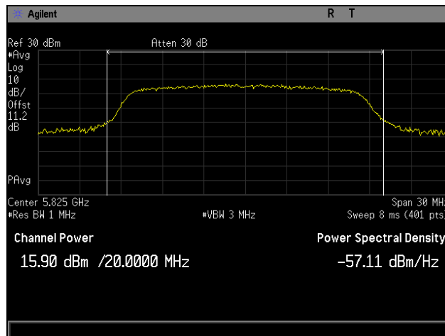
Plot 3. Maximum Conducted Output Power, High Channel, 802.11a, Channel 0
