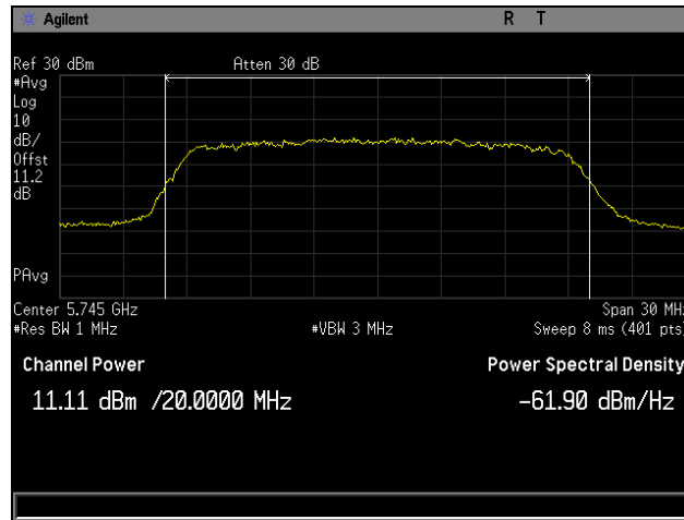
Plot 10. Maximum Conducted Output Power, Low Channel, 802.11n 20 MHz, Channel 0
