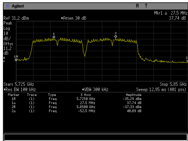
Plot 72. Frequency Stability, 80211ac 40 MHz, -20°C 97VAC
