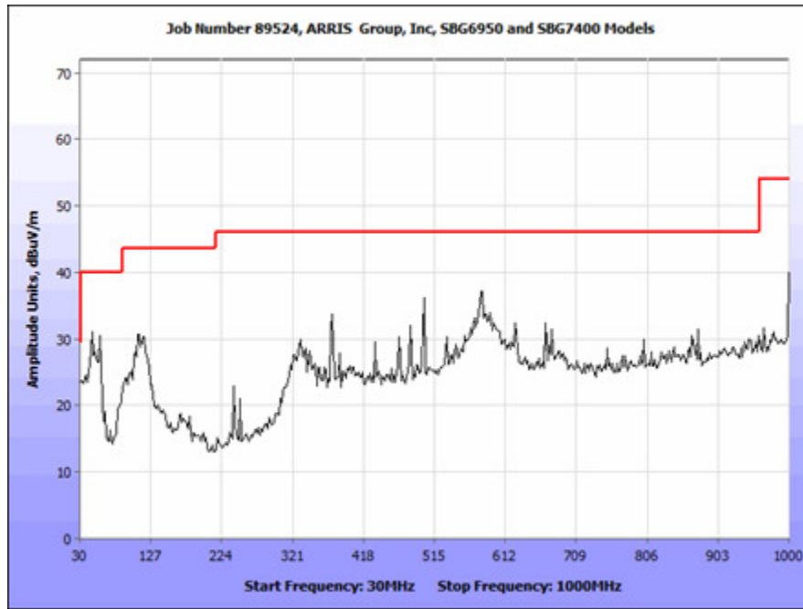
Plot 29. Radiated Spurious Emissions, Low Channel, 802.11a, 30 MHz – 1 GHz
