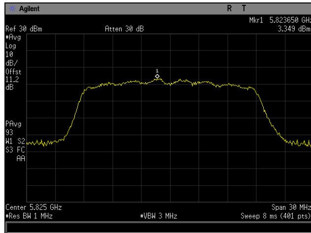
Plot 20. Maximum Power Spectral Density, High Channel, 802.11ac 20 MHz, Channel 0
