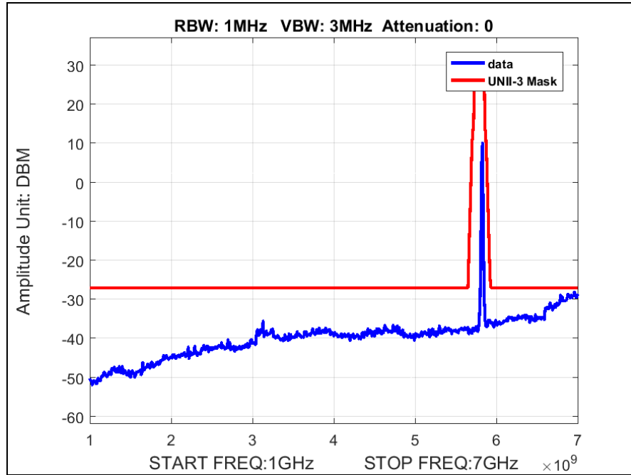
Plot 31. Radiated Spurious Emissions, High Channel, 802.11a, 1 GHz – 7 GHz
