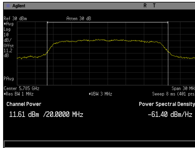
Plot 11. Maximum Conducted Output Power, Mid Channel, 802.11n 20 MHz, Channel 0
