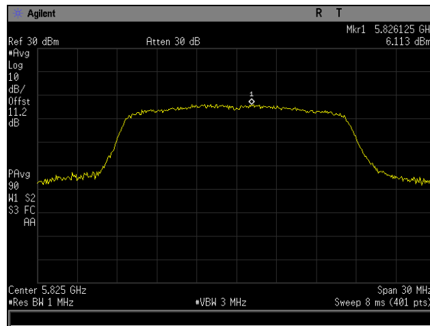
Plot 17. Maximum Power Spectral Density, High Channel, 802.11a, Channel 0
