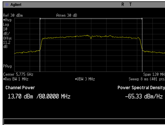
Plot 9. Maximum Conducted Output Power, 802.11ac 80 MHz, Channel 0
