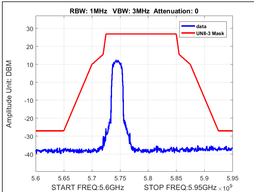
Plot 48. Radiated Band Edge, Low Channel, 802.11n 20 MHz
