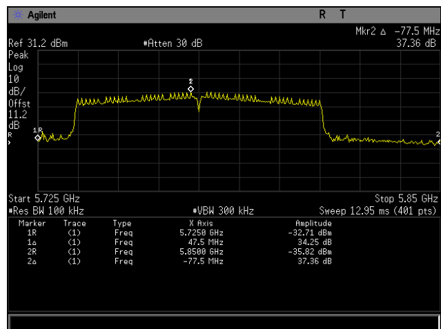
Plot 85. Frequency Stability, 80211ac 80 MHz, 40°C 133VAC
