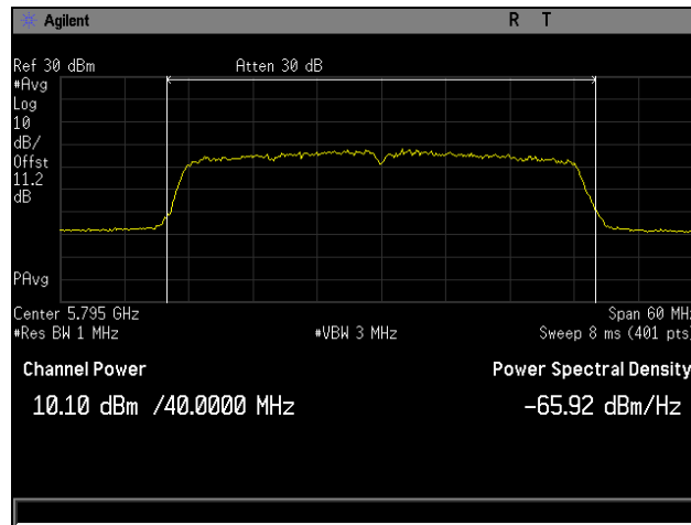
Plot 8. Maximum Conducted Output Power, High Channel, 802.11ac 40 MHz, Channel 0
