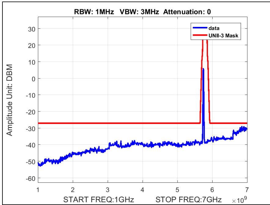
Plot 37. Radiated Spurious Emissions, Low Channel, 802.11n 20 MHz, 1 GHz – 7 GHz
