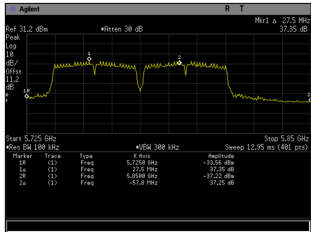
Plot 83. Frequency Stability, 80211n 40 MHz, 40°C 133VAC
