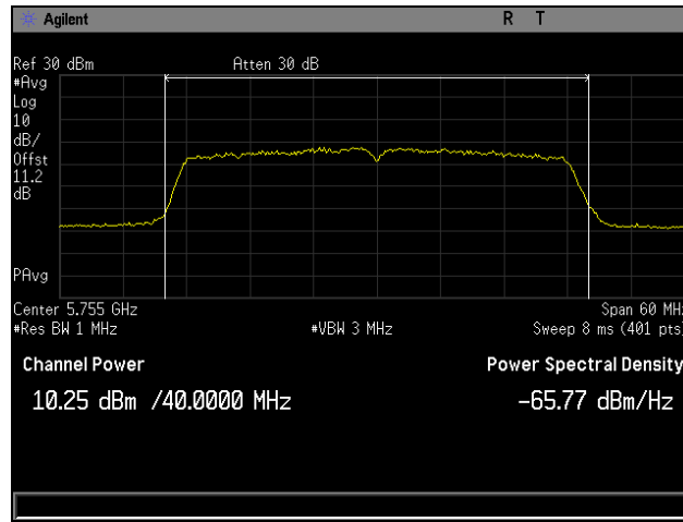
Plot 13. Maximum Conducted Output Power, Low Channel, 802.11n 40 MHz, Channel 0
