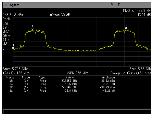
Plot 76. Frequency Stability, 80211n 20 MHz, 20°C 115VAC
