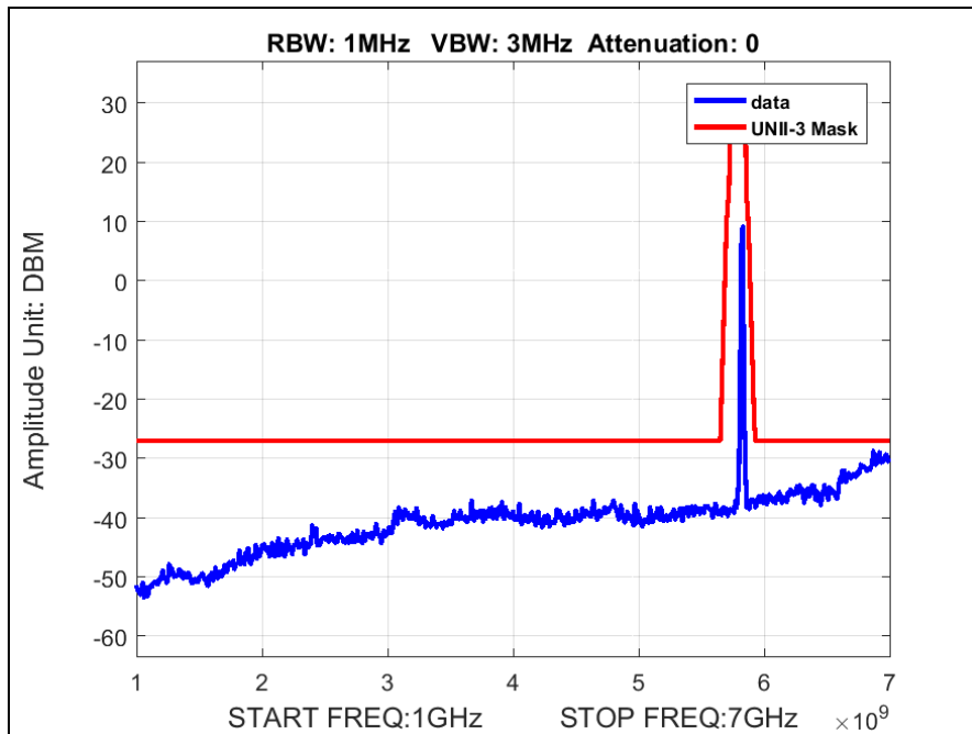
Plot 38. Radiated Spurious Emissions, High Channel, 802.11n 20 MHz, 1 GHz – 7 GHz
