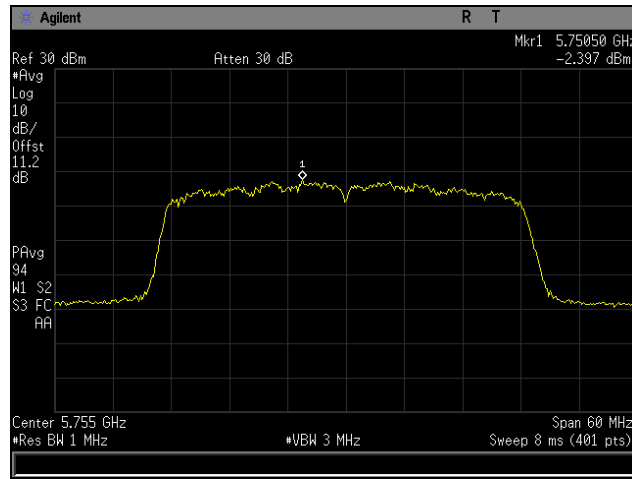
Plot 21. Maximum Power Spectral Density, Low Channel, 802.11ac 40 MHz, Channel 0
