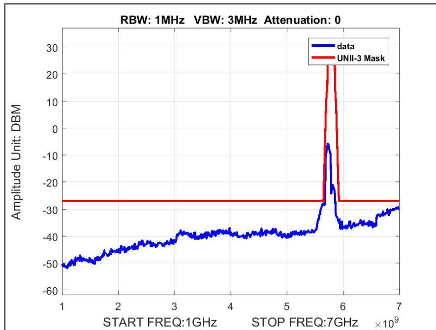
Plot 36. Radiated Spurious Emissions, 802.11ac 80 MHz, 1 GHz – 7 GHz
