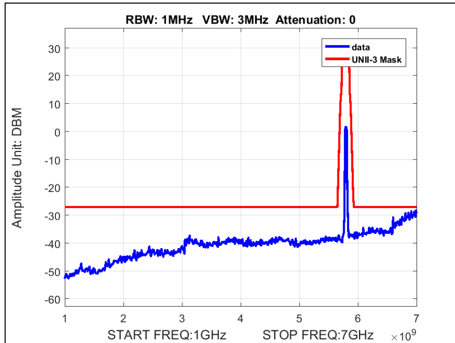
Plot 40. Radiated Spurious Emissions, High Channel, 802.11n 40 MHz, 1 GHz – 7 GHz
