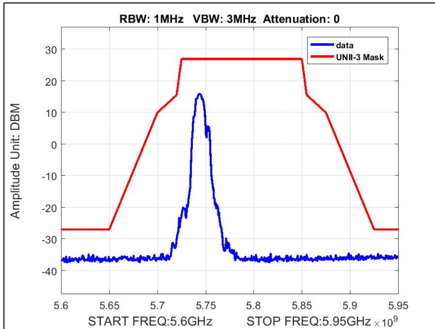
Plot 41. Radiated Band Edge, Low Channel, 802.11a
