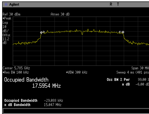
Plot 64. 6 dB Occupied Bandwidth, Mid Channel, 802.11n 20 MHz
