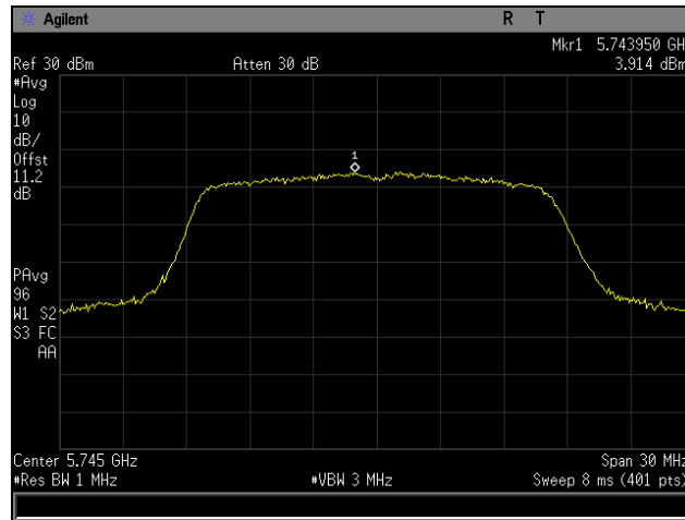
Plot 15. Maximum Power Spectral Density, Low Channel, 802.11a, Channel 0
