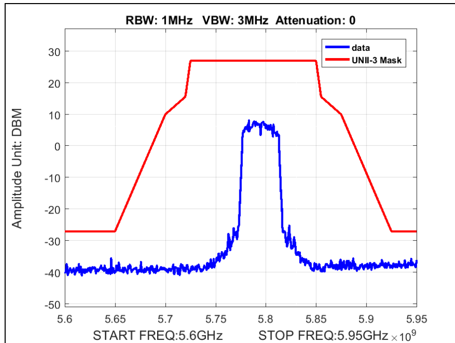
Plot 51. Radiated Band Edge, High Channel, 802.11n 40 MHz
