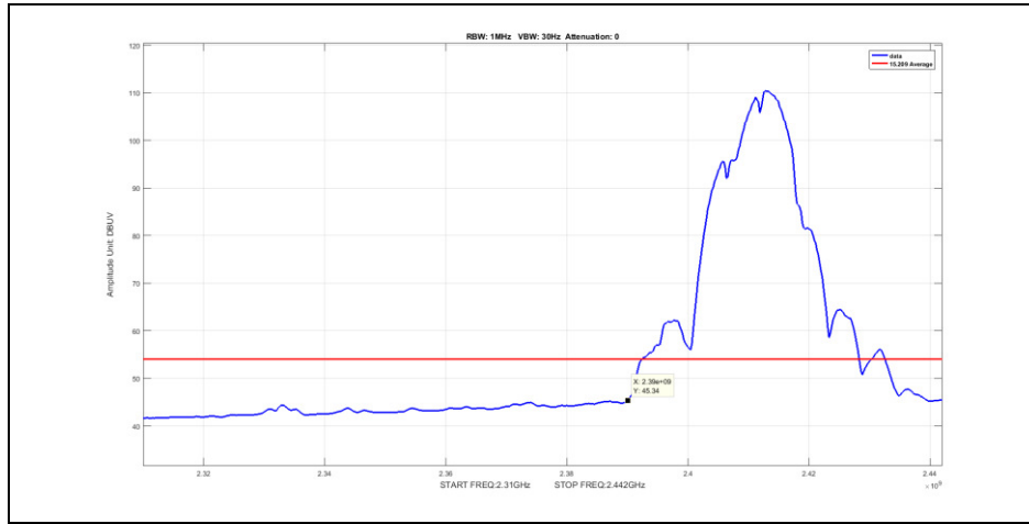
Plot 36. Radiated Restricted Band Edge, Average, Low Channel, 802.11b
