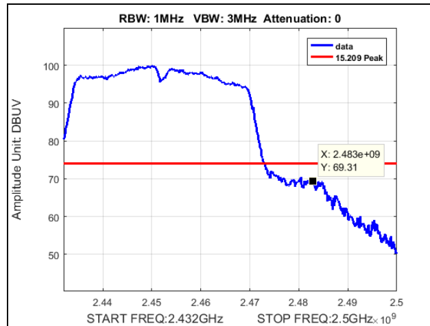
Plot 51. Radiated Restricted Band Edge, Peak, High Channel, 802.11n 40 MHz
