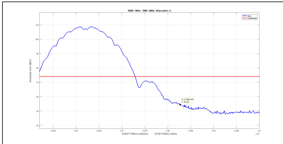
Plot 39. Radiated Restricted Band Edge, Peak, High Channel, 802.11b
