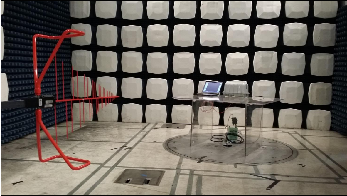
Photograph 1. Undesirable Emissions, 30 MHz – 1 GHz, Test Setup
