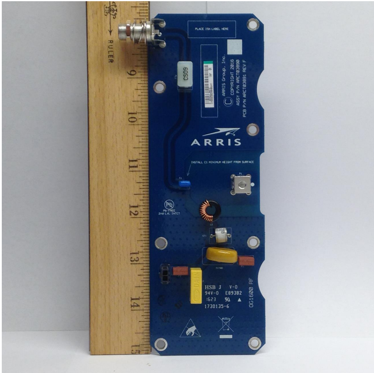
Photograph 3. RF Top
