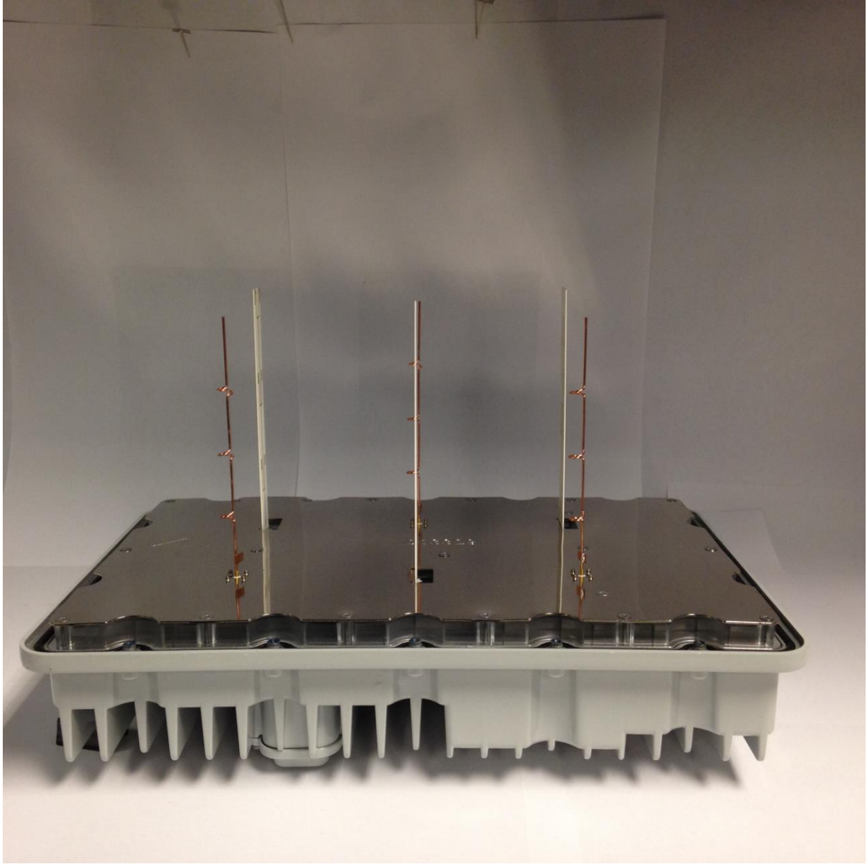
Photograph 11. Antenna Front
