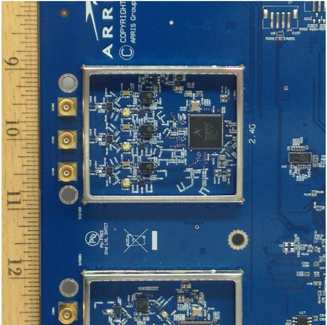
Photograph 9. 2.4G Radio Top
