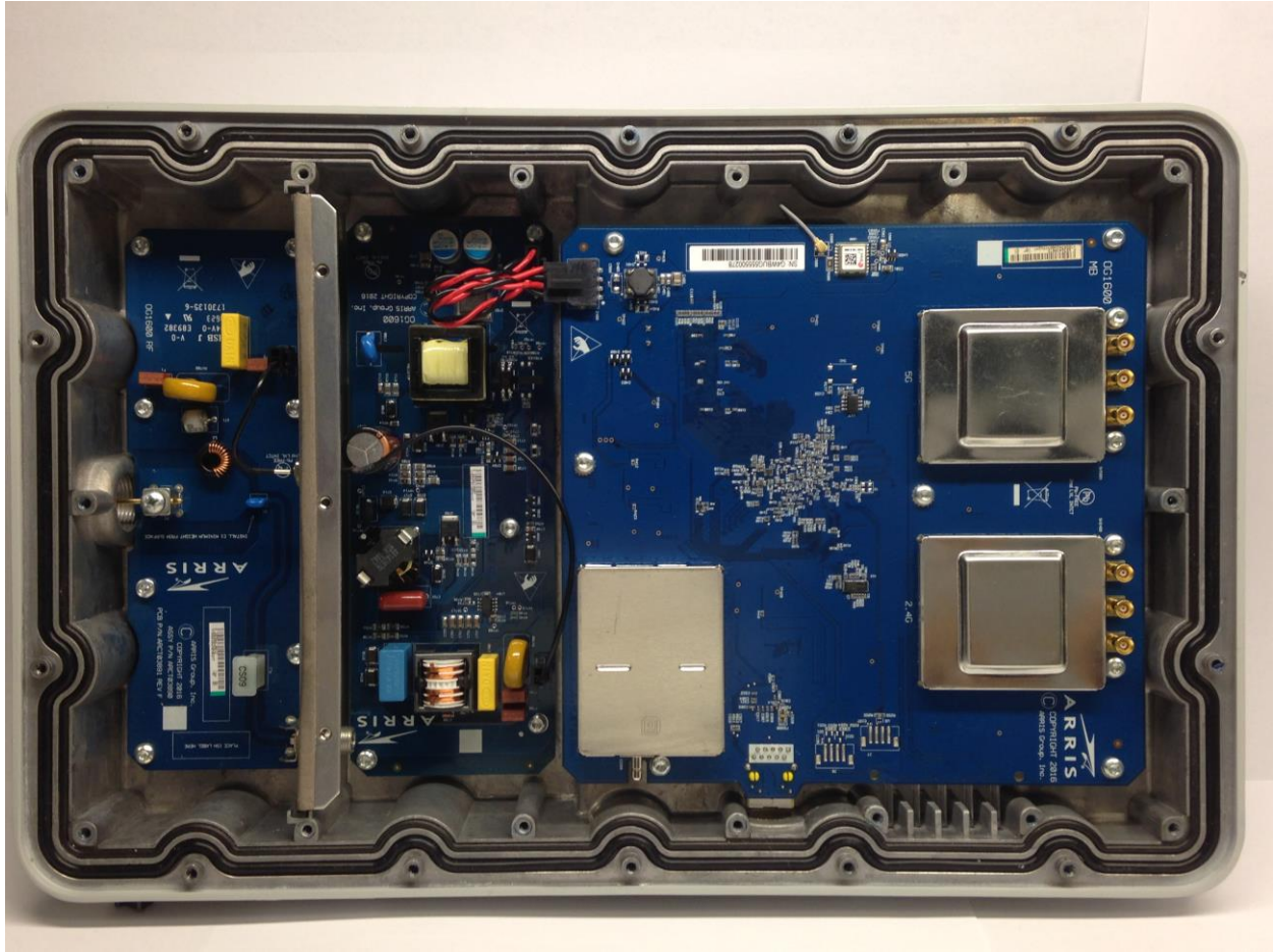
Photograph 2. OG1600 Encl MB PS IO
