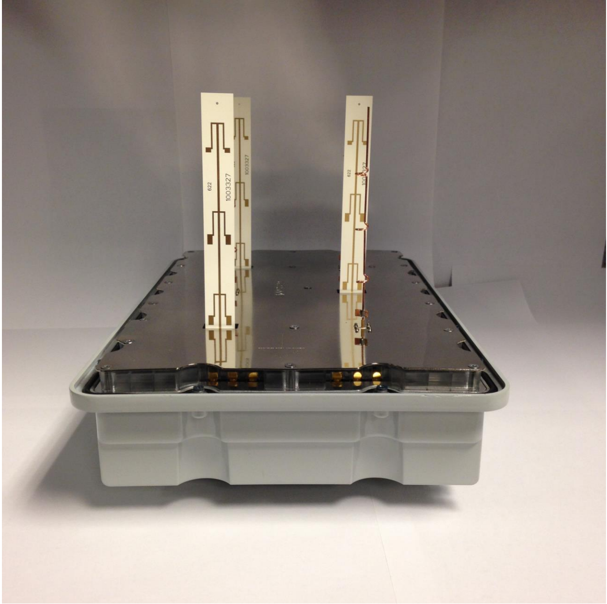
Photograph 12. Antenna Side
