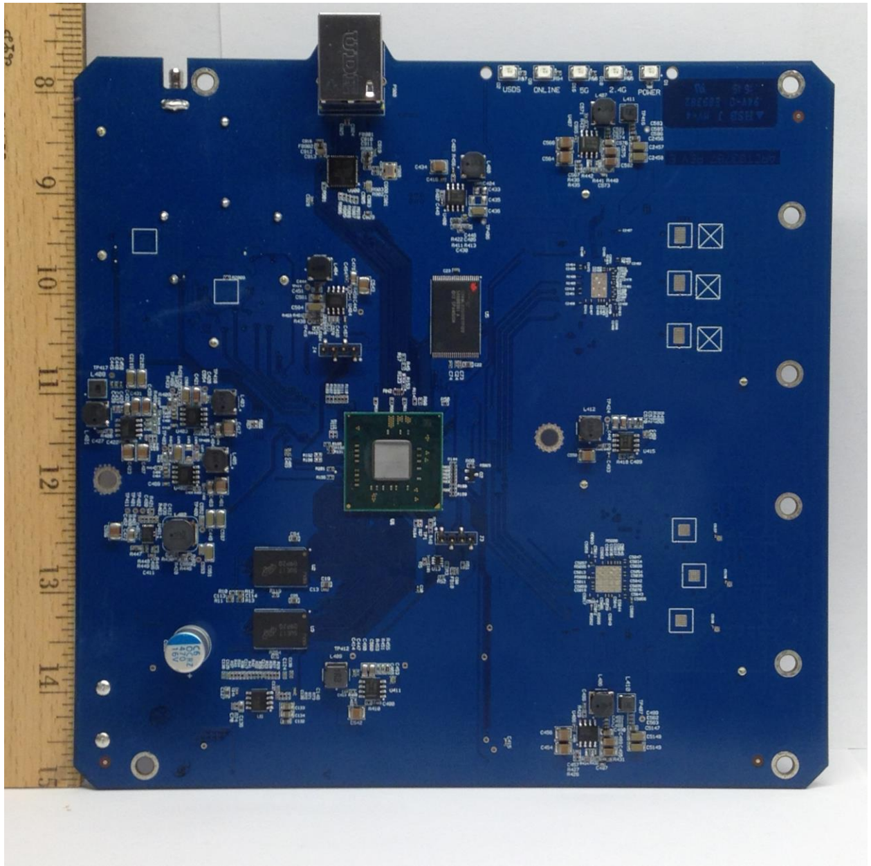
Photograph 8. MB Bottom
