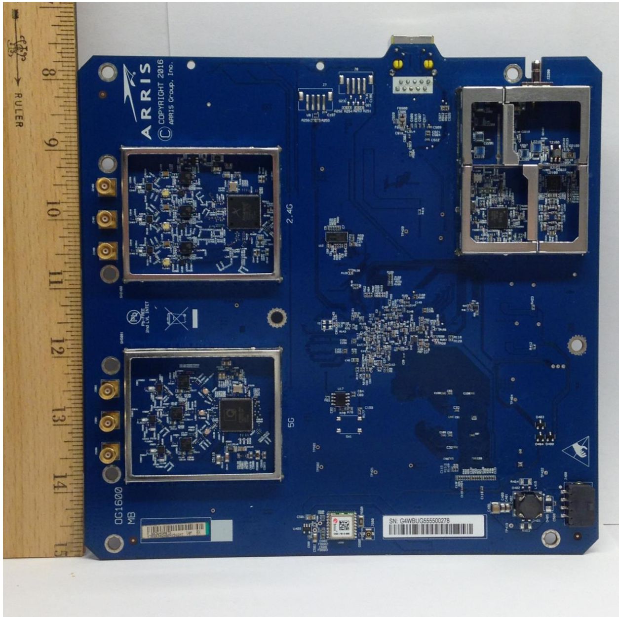
Photograph 7. MB Top
