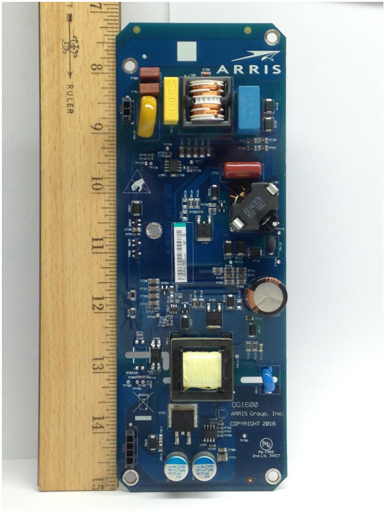
Photograph 5. PS Top
