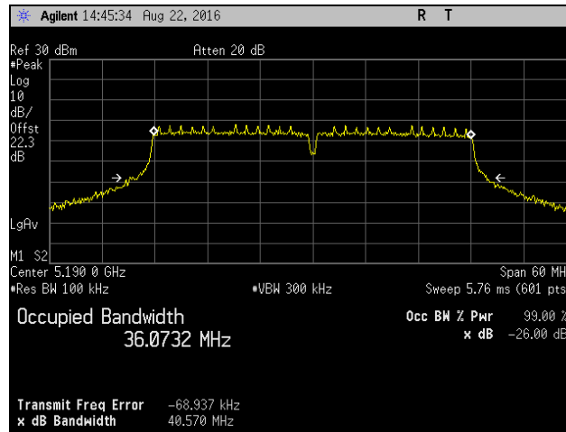
Plot 11. Occupied Bandwidth, Channel 5190 MHz, 802.11ac 40 MHz, vf0 TP12
