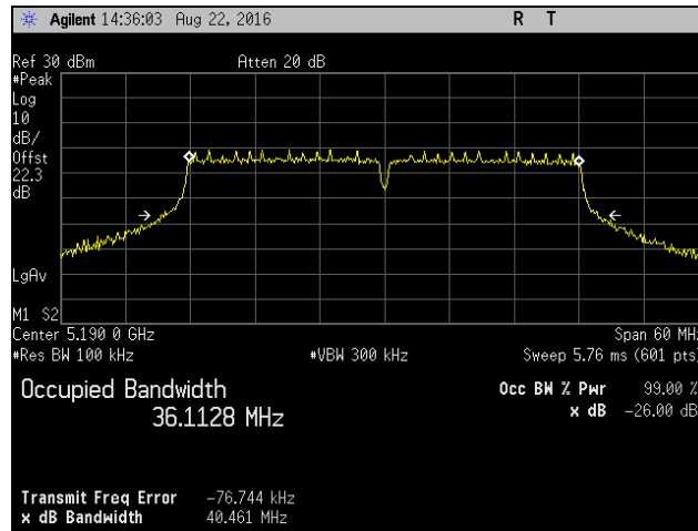
Plot 13. Occupied Bandwidth, Channel 5190 MHz, 802.11n 40 MHz, f0 TP13.5
