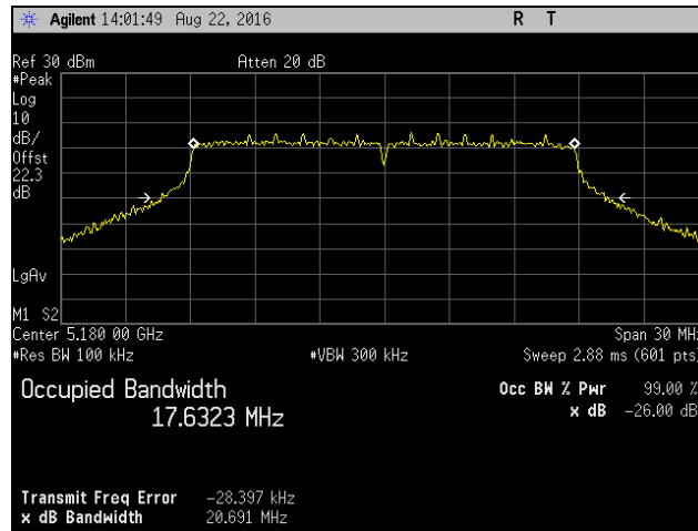
Plot 8. Occupied Bandwidth, Channel 5180 MHz, 802.11n 20 MHz, t0 TP16.5
