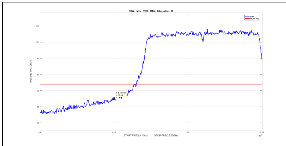
Plot 63. Radiated Band Edge, Channel 5210 MHz, 802.11ac 80 MHz, Peak
