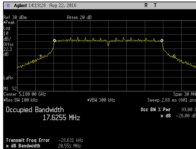
Plot 4. Occupied Bandwidth, Channel 5180 MHz, 802.11ac 20 MHz, vt0 TP16.5
