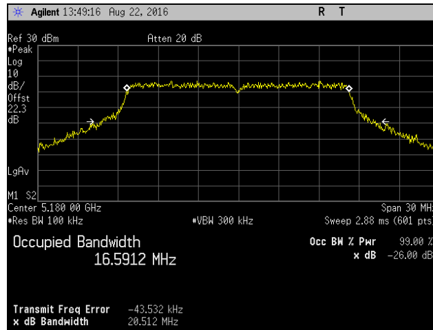
Plot 1. Occupied Bandwidth, Channel 5180 MHz, 802.11a 20 MHz, r6 TP16.5
