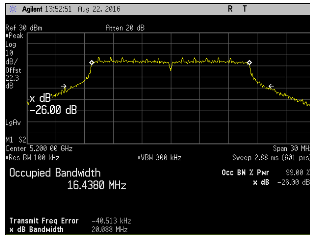
Plot 2. Occupied Bandwidth, Channel 5200 MHz, 802.11a 20 MHz, r6 TP18
