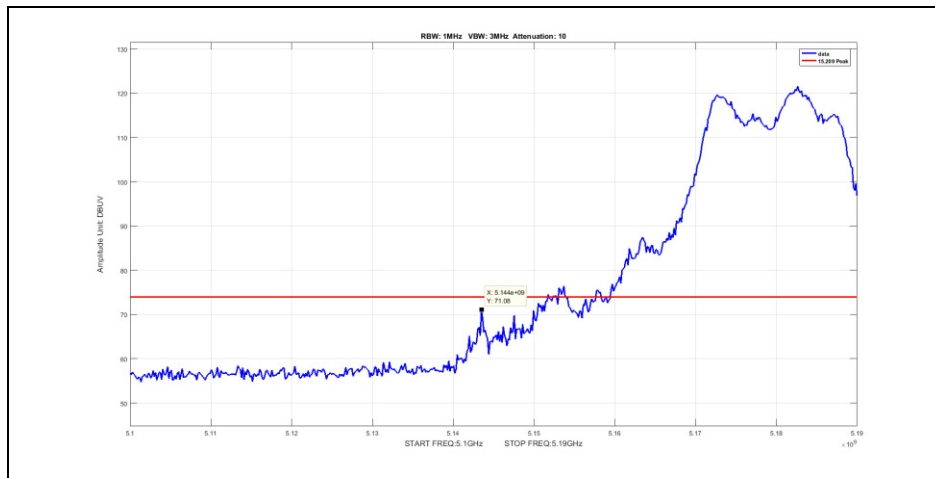
Plot 43. Radiated Band Edge, Channel 5180 MHz, 802.11a 20 MHz, r6 TP22.5, Peak
