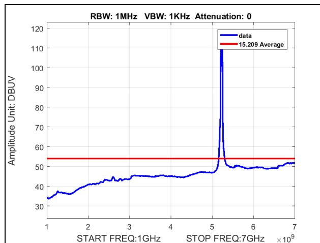
Plot 32. Radiated Spurious Emissions, Channel 5230 MHz, 802.11ac 40 MHz, 1 GHz – 7 GHz, vf0 TP22, Average
