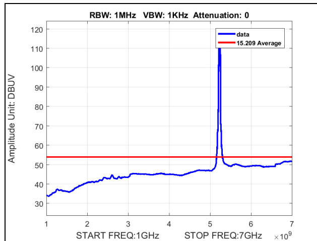
Plot 36. Radiated Spurious Emissions, Channel 5230 MHz, 802.11n 40 MHz, 1 GHz – 7 GHz, f0 TP21.5, Average
