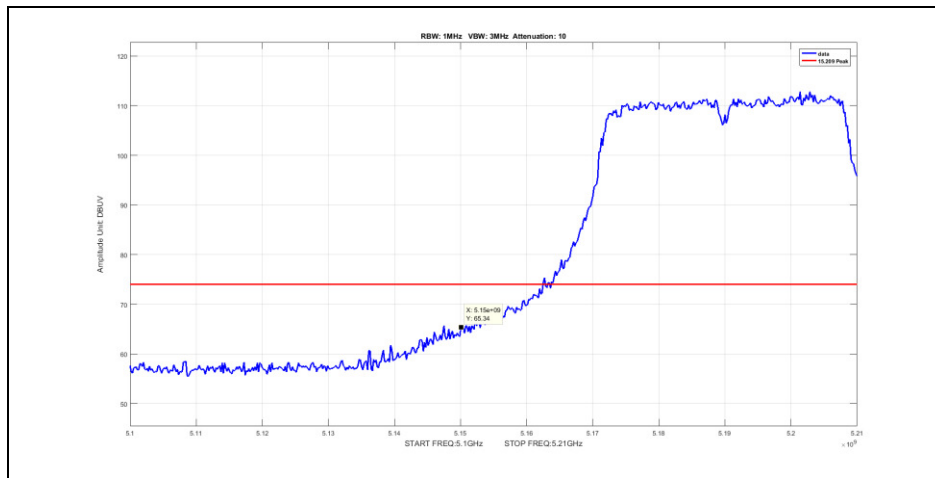
Plot 55. Radiated Band Edge, Channel 5190 MHz, 802.11ac 40 MHz, vf20 TP19, Peak
