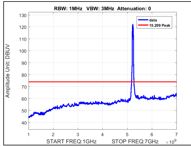
Plot 33. Radiated Spurious Emissions, Channel 5230 MHz, 802.11ac 40 MHz, 1 GHz – 7 GHz, v0 TP22, Peak
