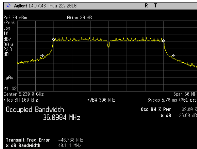
Plot 14. Occupied Bandwidth, Channel 5230 MHz, 802.11n 40 MHz, f0 TP20.5
