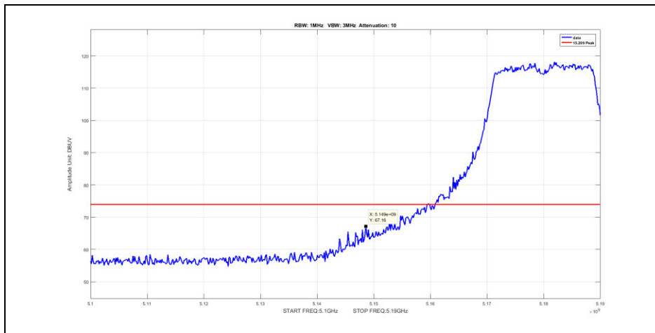
Plot 47. Radiated Band Edge, Integration Method, Channel 5180 MHz, 802.11ac 20 MHz, vt0 TP16.5, Peak
