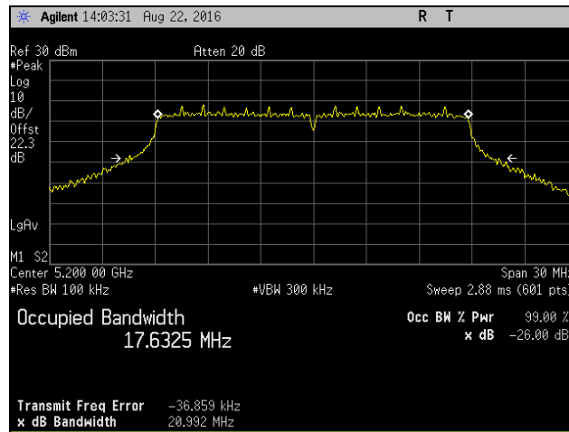
Plot 9. Occupied Bandwidth, Channel 5200 MHz, 802.11n 20 MHz, t0 TP18
