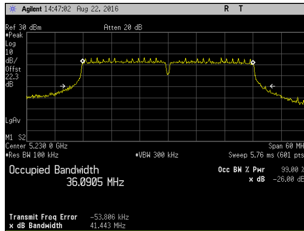
Plot 12. Occupied Bandwidth, Channel 5230 MHz, 802.11ac 40 MHz, vf0 TP20.5
