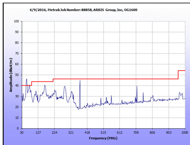
Plot 17. Radiated Spurious Emissions, 30 MHz – 1 GHz Radio On
