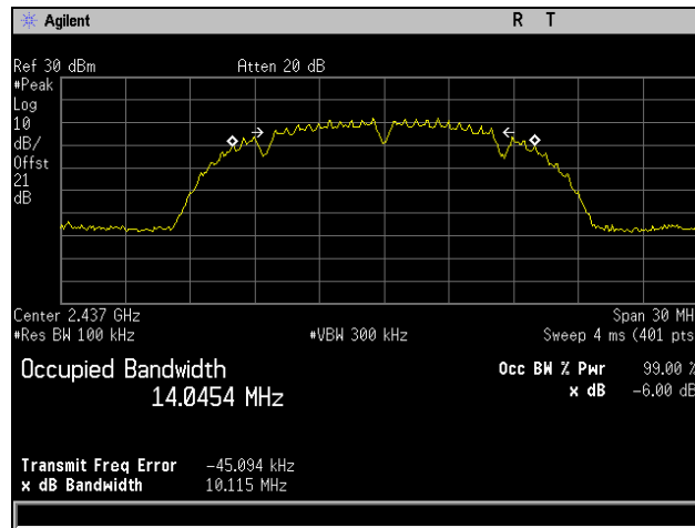
Plot 4. 6 dB Occupied Bandwidth, Mid Channel, 802.11b 20 MHz
