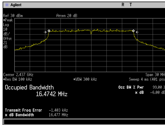
Plot 7. 6 dB Occupied Bandwidth, Mid Channel, 802.11g 20 MHz
