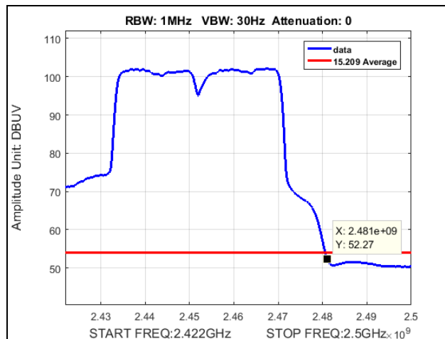
Plot 109. Radiated Restricted Band Edge, High Channel, 802.11n 40 MHz, Average
