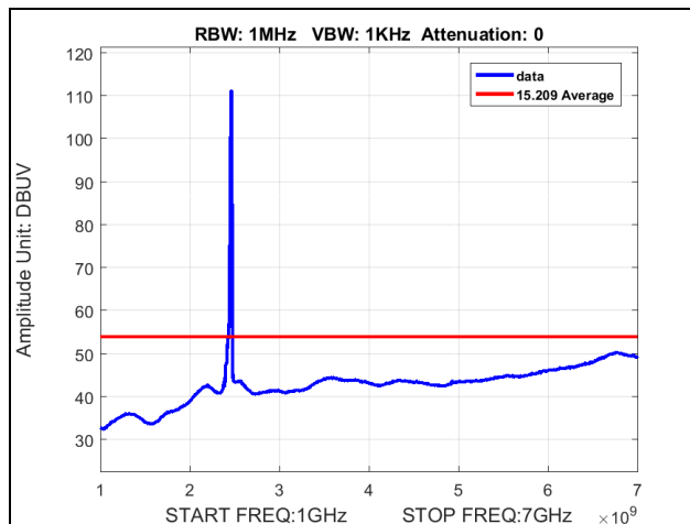
Plot 73. Radiated Spurious Emissions, Mid Channel, 802.11b 20 MHz, 1 GHz – 7 GHz, Average
