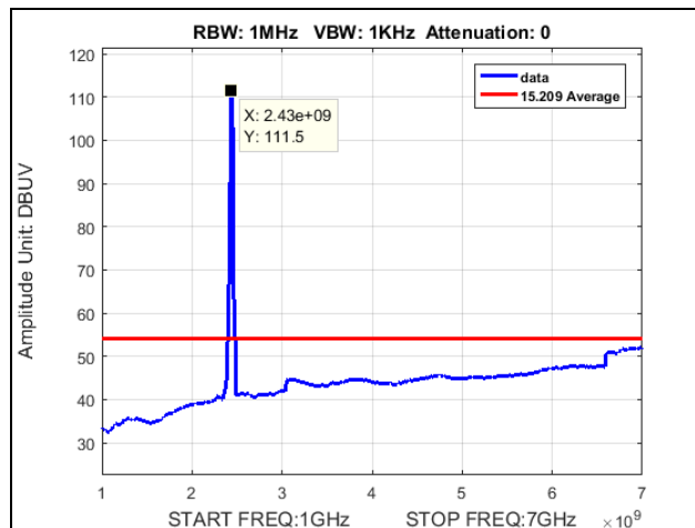
Plot 85. Radiated Spurious Emissions, Mid Channel, 802.11n 20 MHz, 1 GHz – 7 GHz, Average
