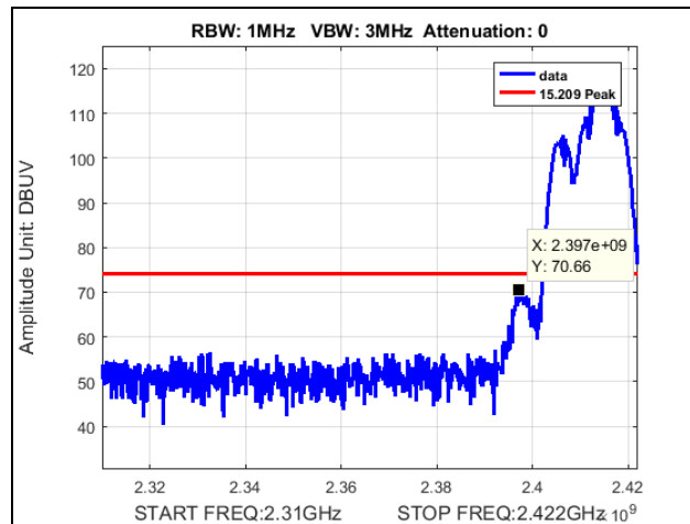
Plot 96. Radiated Restricted Band Edge, Low Channel, 802.11b 20 MHz, Peak
