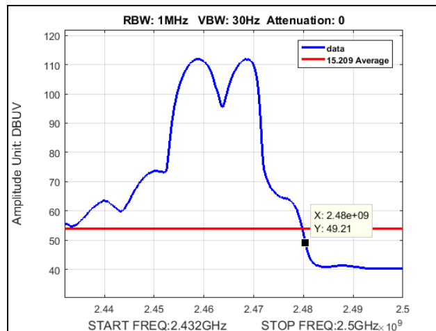
Plot 101. Radiated Restricted Band Edge, High Channel, 802.11g 20 MHz, Average
