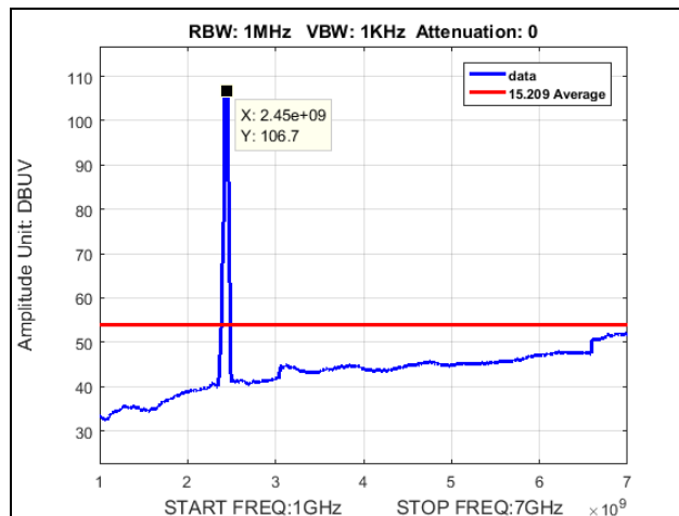
Plot 91. Radiated Spurious Emissions, Mid Channel, 802.11n 40 MHz, 1 GHz – 7 GHz, Average
