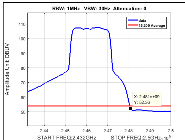
Plot 105. Radiated Restricted Band Edge, High Channel, 802.11n 20 MHz, Average
