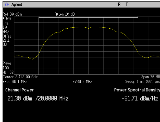
Plot 27. Peak Power Output, Low Channel, 802.11b 20 MHz, Port 2
