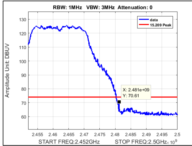
Plot 106. Radiated Restricted Band Edge, High Channel, 802.11n 20 MHz, Peak
