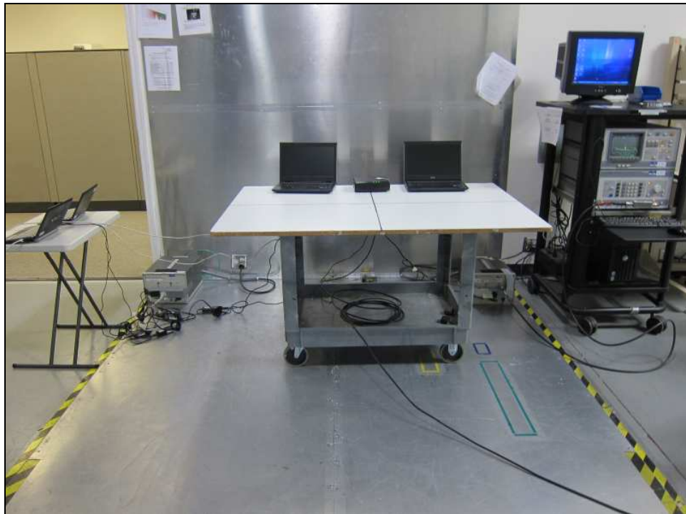
Figure 3: Radiated Emissions
