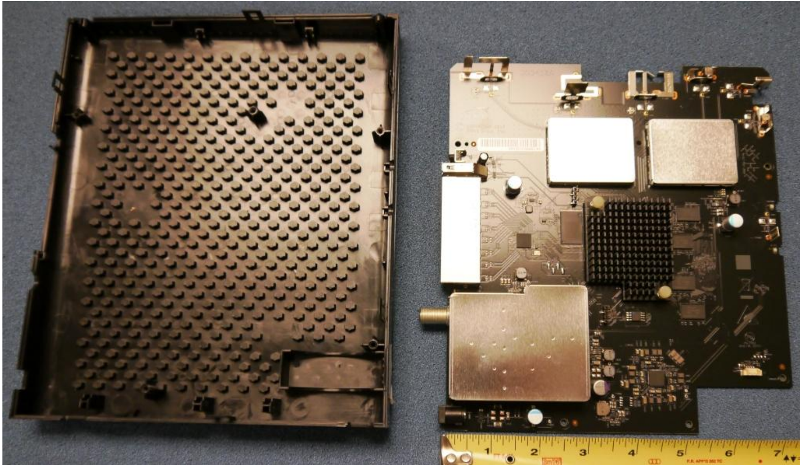
Open cover view –PCB Removed
