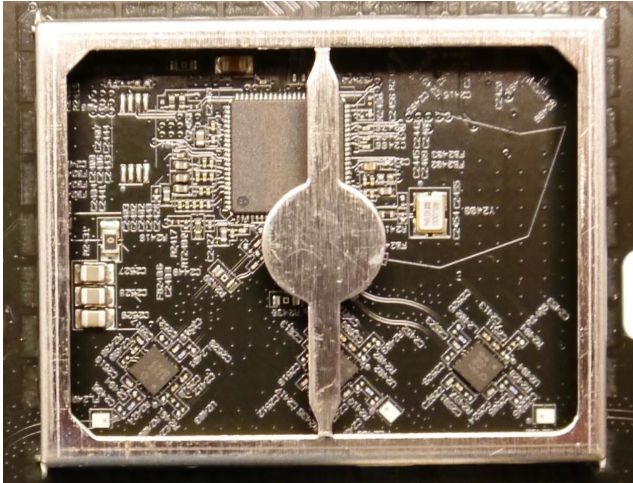
2.4GHz Radio – Can Removed
