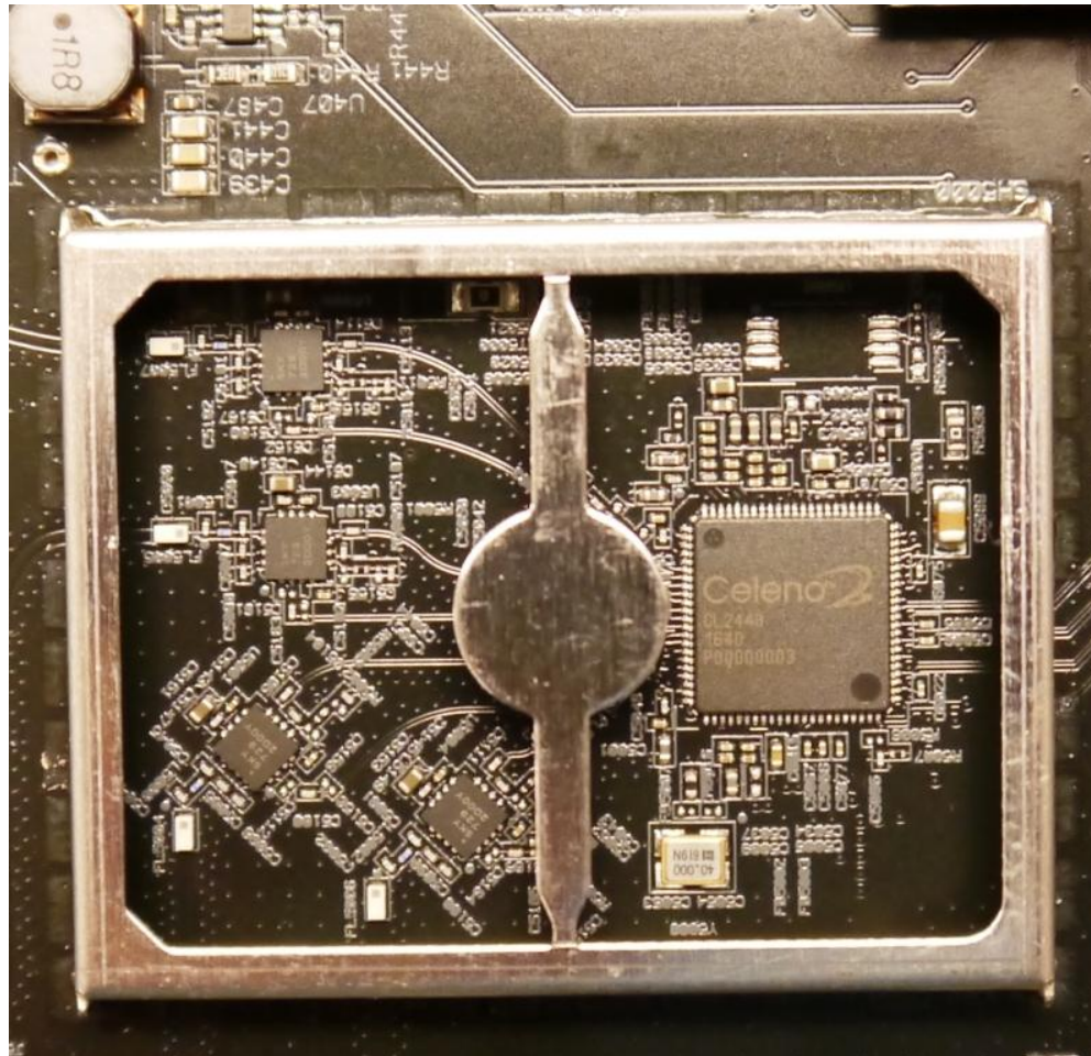
5GHz Radio – Can Removed
