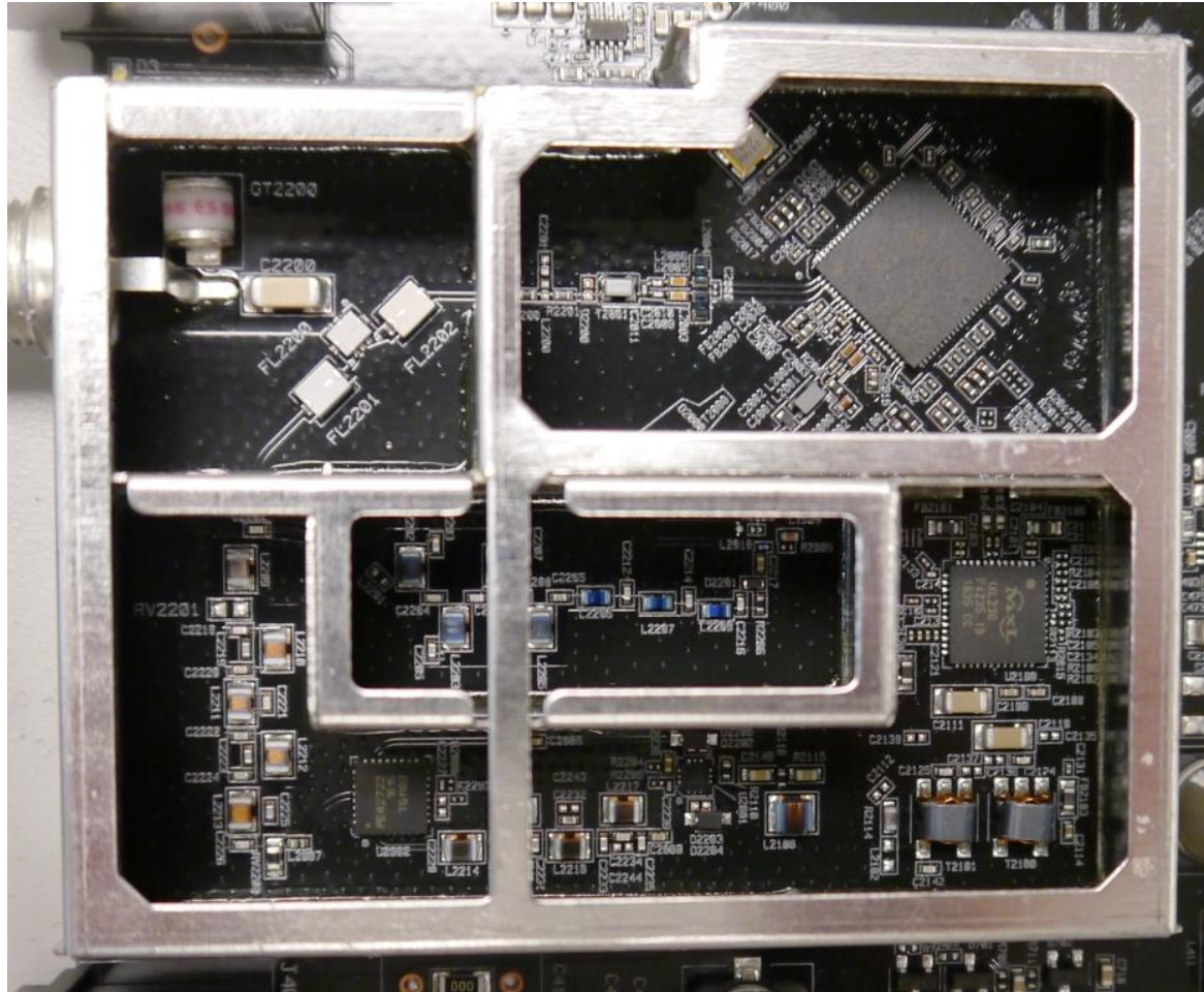
RF Cable Interface – Can Removed
