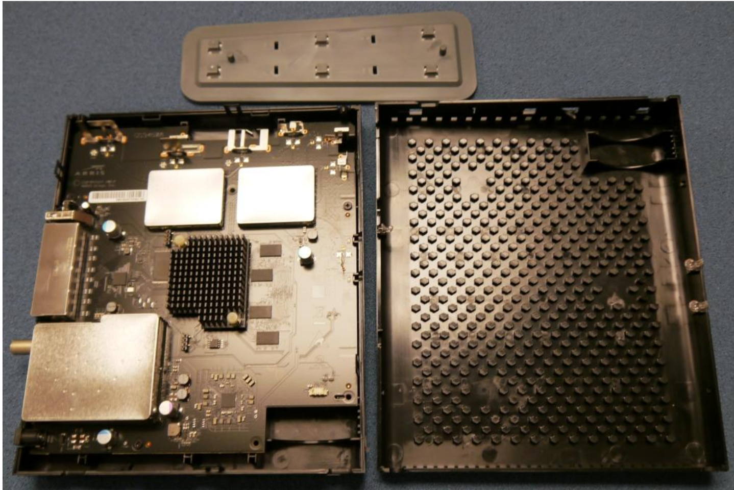
Open cover view - Top
