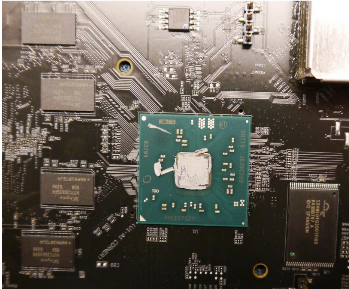
Processor – Heat Sink Removed
