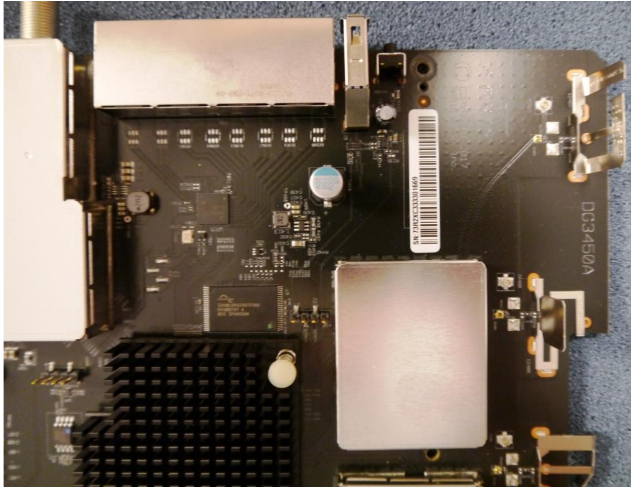
PCB Top – Upper / Right Quadrant
